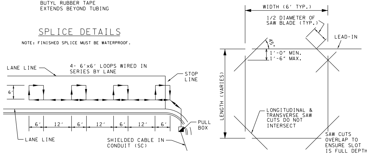
ALT. LAYOUT OF LOOP DETECTORS (FOR PRESENCE DETECTION)
