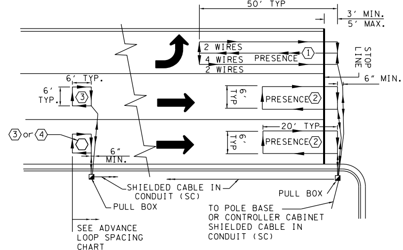
ALTERNATE HIGH SPEED APPROACH**
