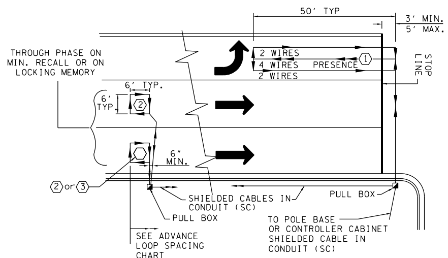
TYPICAL HIGH SPEED APPROACH*
