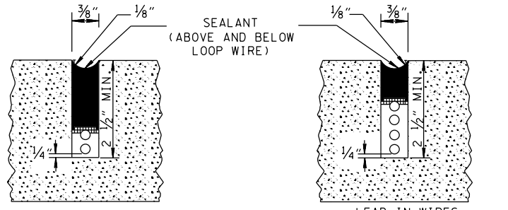
LOOP IN ASPHALT LOOP IN CONCRETE TYPICAL SAW SLOT & LOOP WIRE DETAIL
