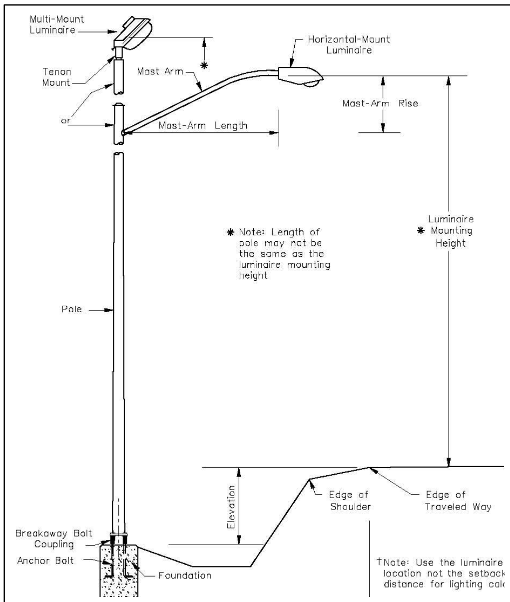
Figure 1.13 – Typical Highway Lighting Structure
