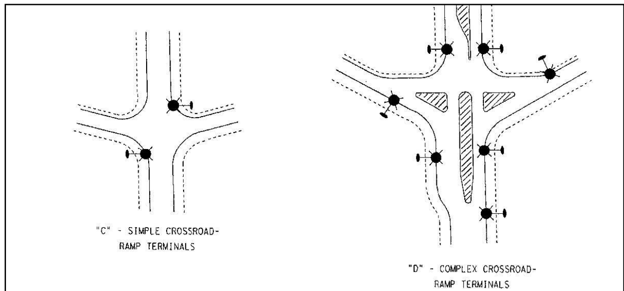
Figure 1.2 – Partial Interchange Lighting (Crossing Types C and D)
