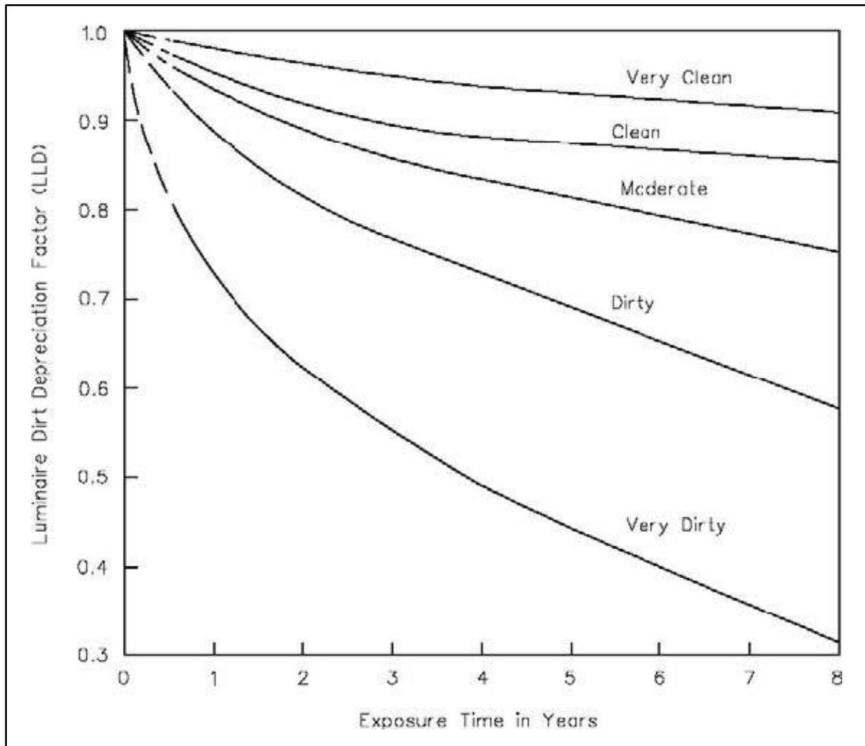
Figure 1.6 – Roadway Luminaire Dirt Depreciation Curve
