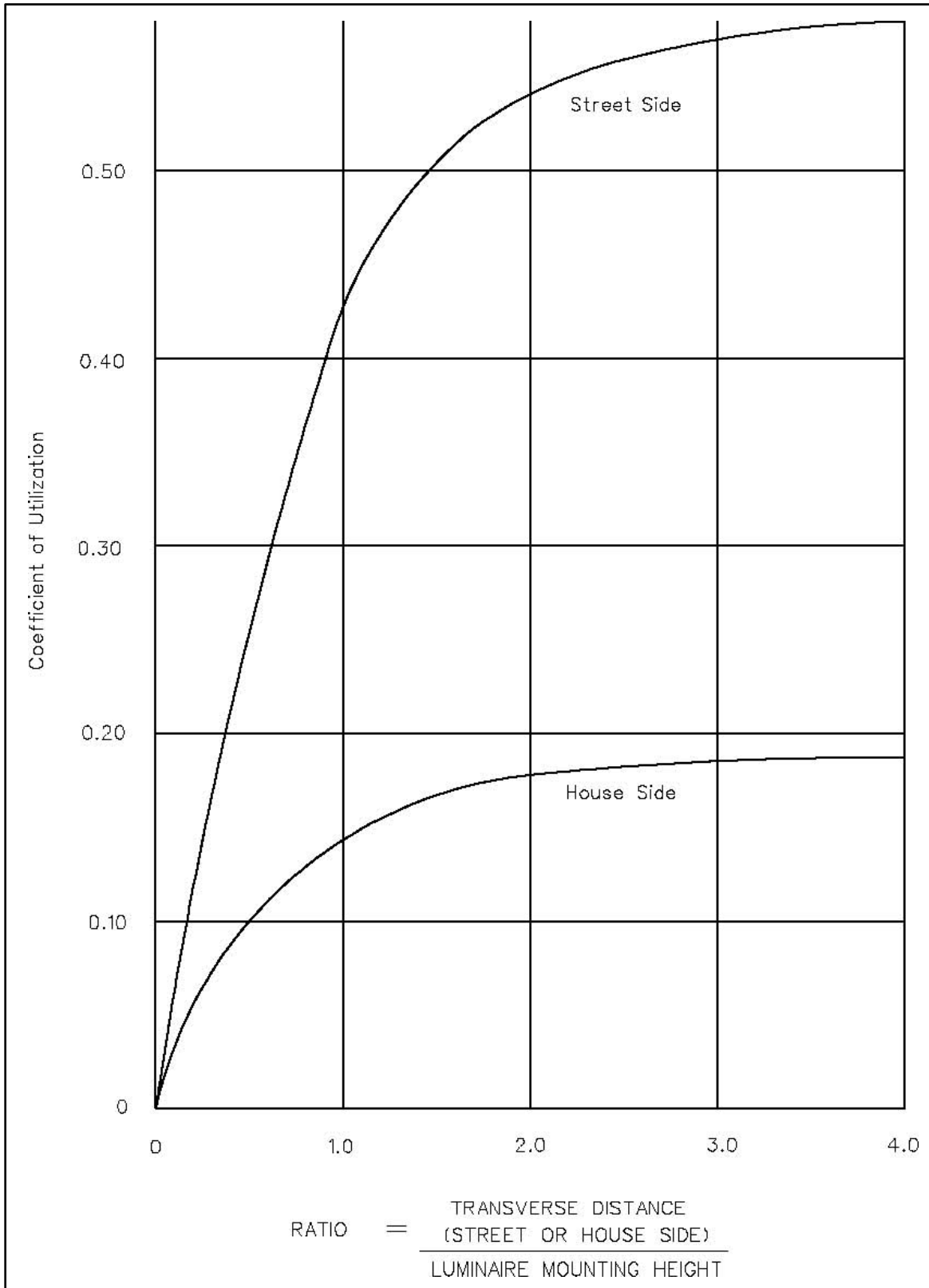
Figure 1.5 – Sample Utilization Curve
