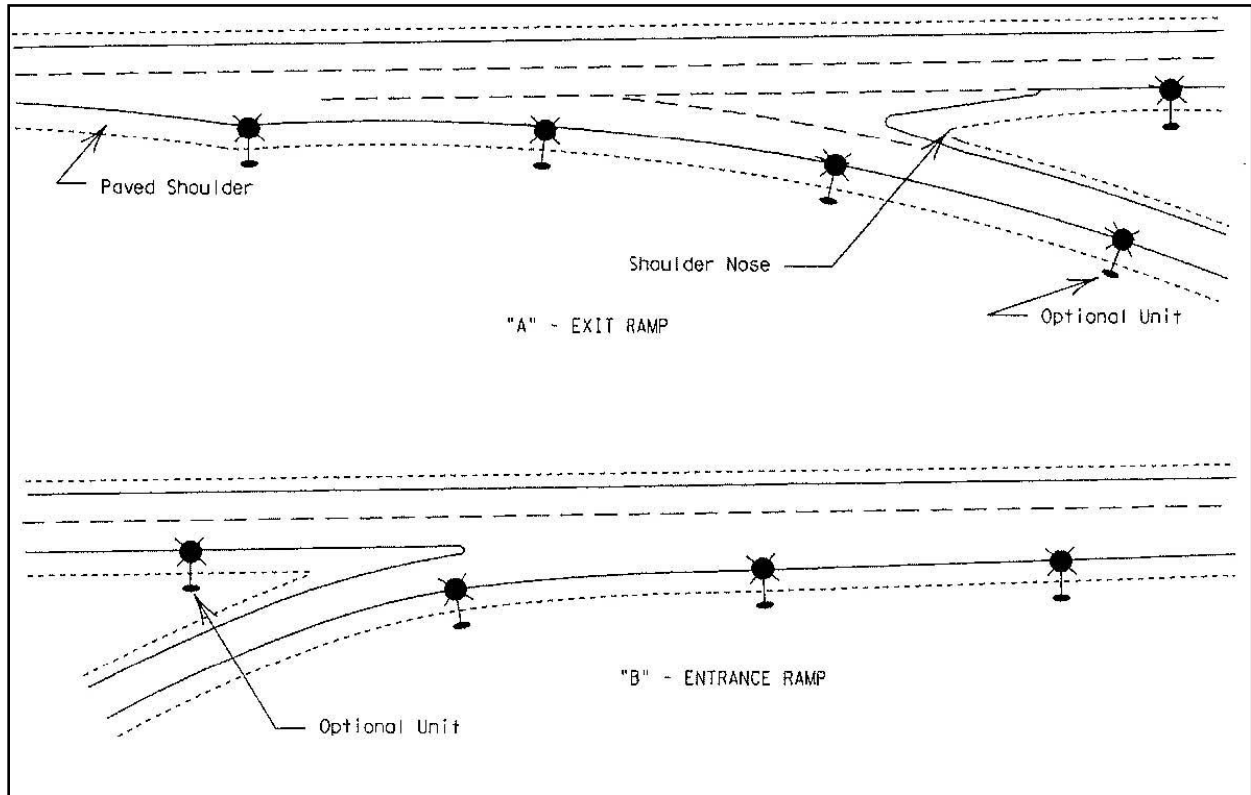
Figure 1.1 – Partial Interchange Lighting (Crossing Types A and B)
