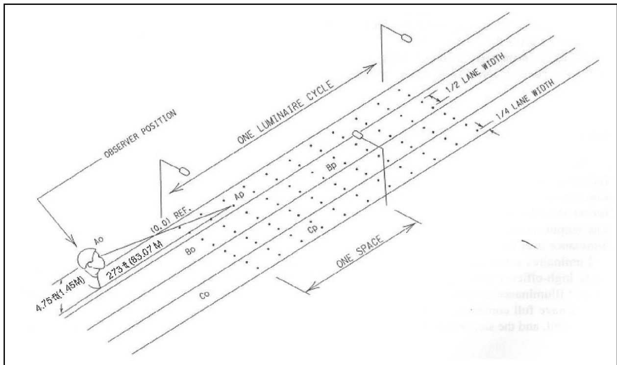
Figure 1.8 – Calculation Points for Luminance and Illuminance Design Methods
