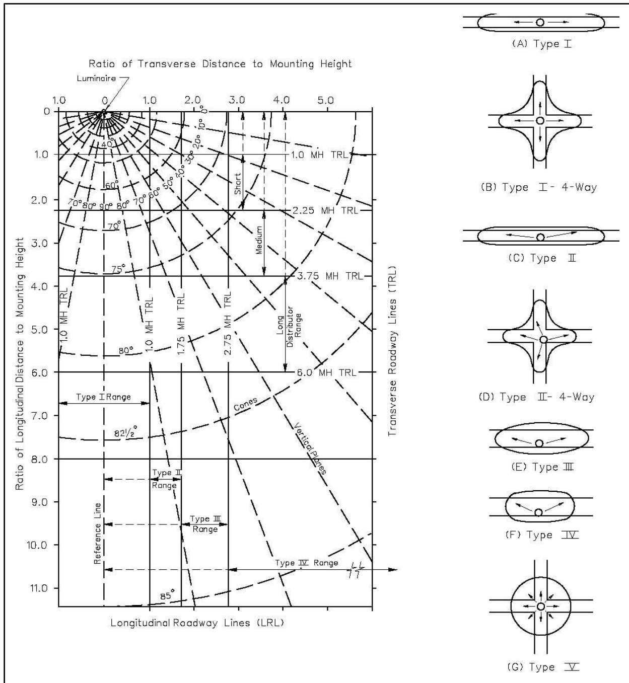
Figure 1.4 – Plan View of Roadway Coverage from IES Luminaries
