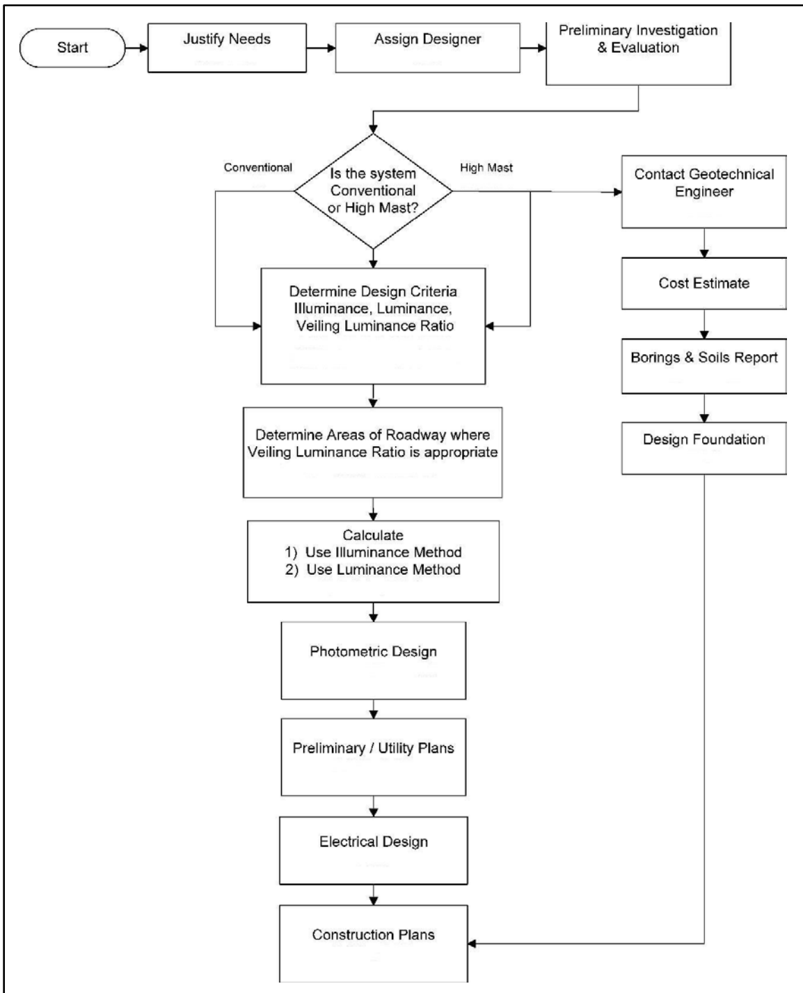
Figure 1.3 – Lighting Design Process Flow Chart
