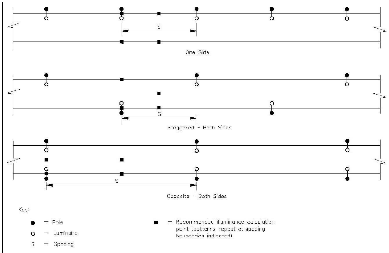
Figure 1.7 – Typical Luminaire Arrangements for Conventional Highway Lighting Design
