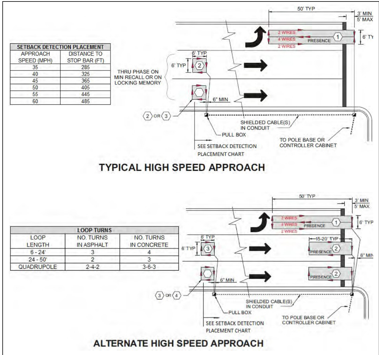
Figure 5.4 – Inductive Loop Detection (≥ 35 MPH)
