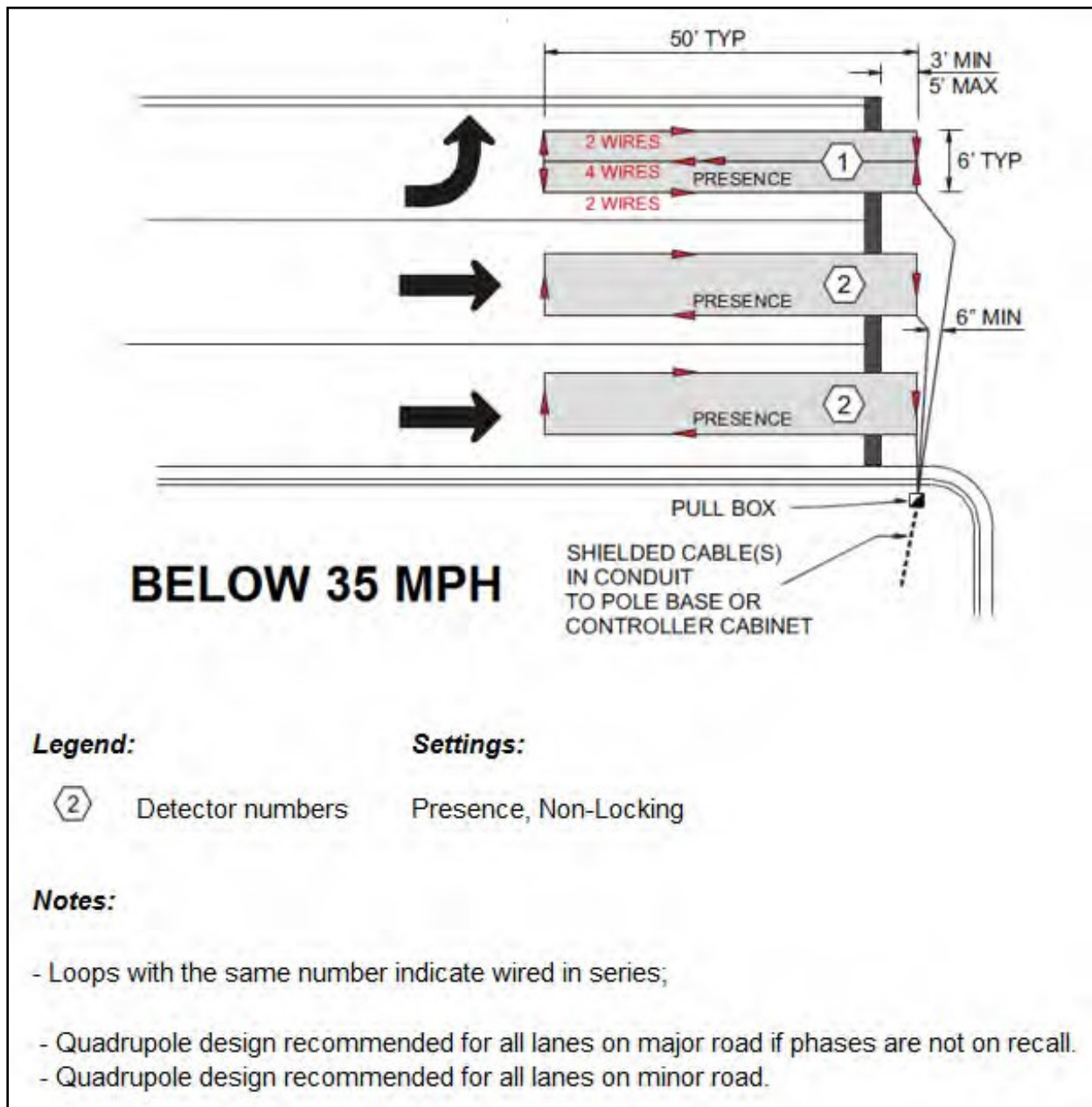
Figure 5.2 – Inductive Loop Detection (< 35 MPH)
