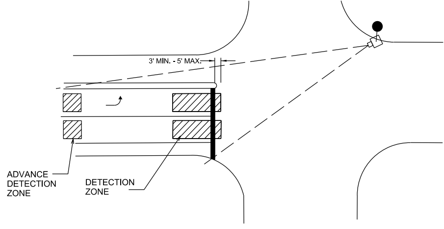
ALTERNATIVE VIDEO DETECTOR DETAIL
