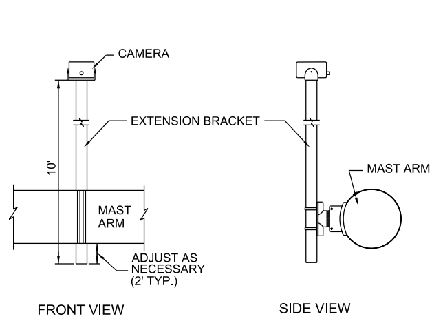
ALTERNATE CAMERA MOUNTING DETAIL (MAST ARM) (TO EXTEND CAMERA HEIGHT ABOVE MAST ARM)
