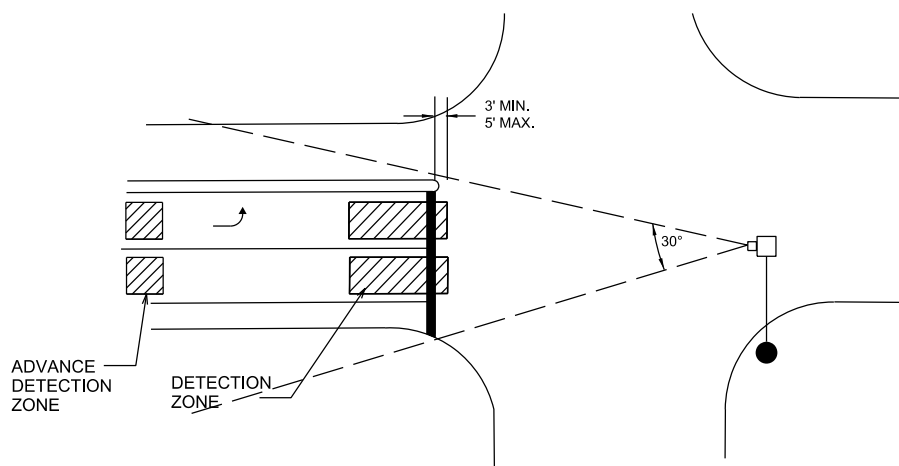
STANDARD VIDEO DETECTOR DETAIL
