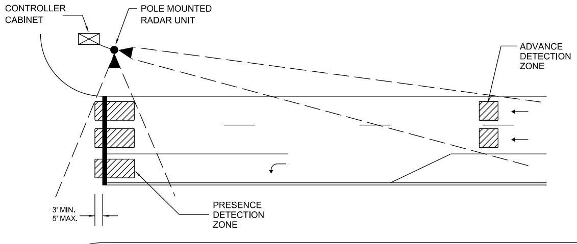
RADAR DETECTOR DETAIL
