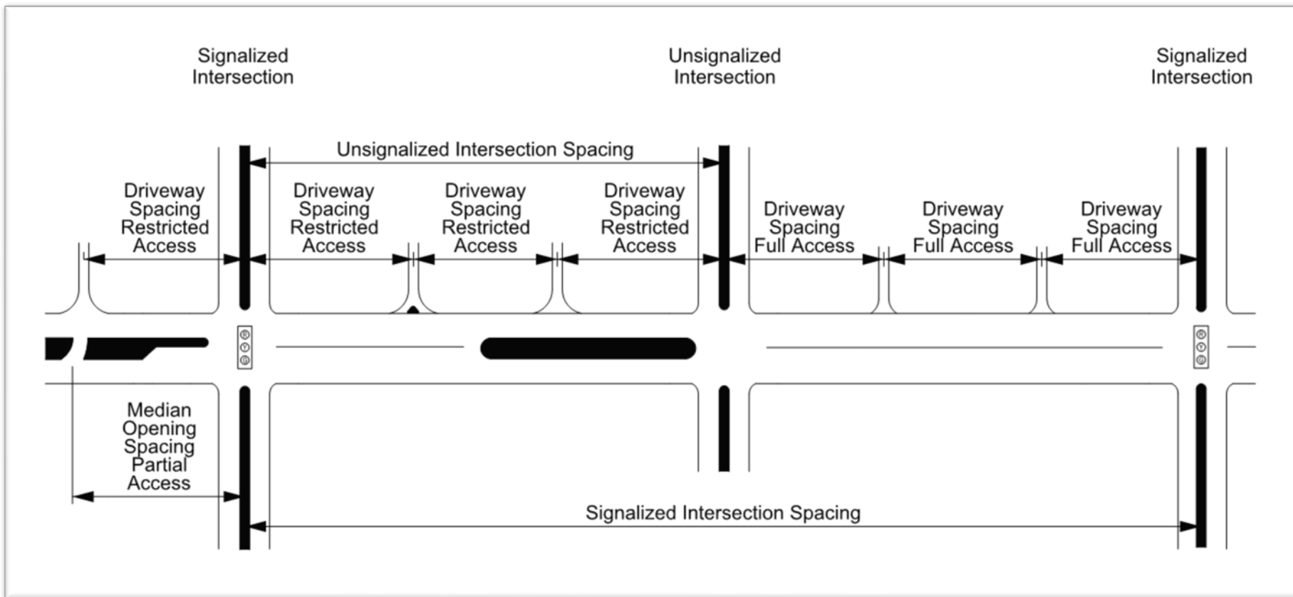
Figure 3-5: Typical Access Point Spacing
