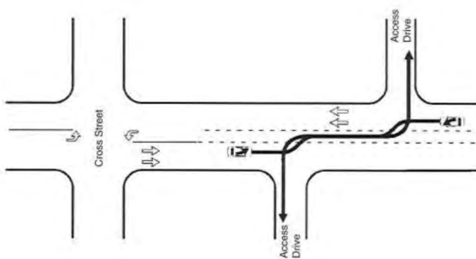
Figure 3-10: Overlapping Left-Turn Movements with Two-Way Left-Turn Lane 11, 12
