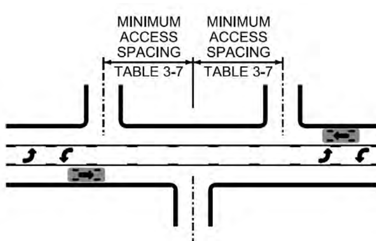
Figure 3-12: Minimum Spacing of Offset Access Points
