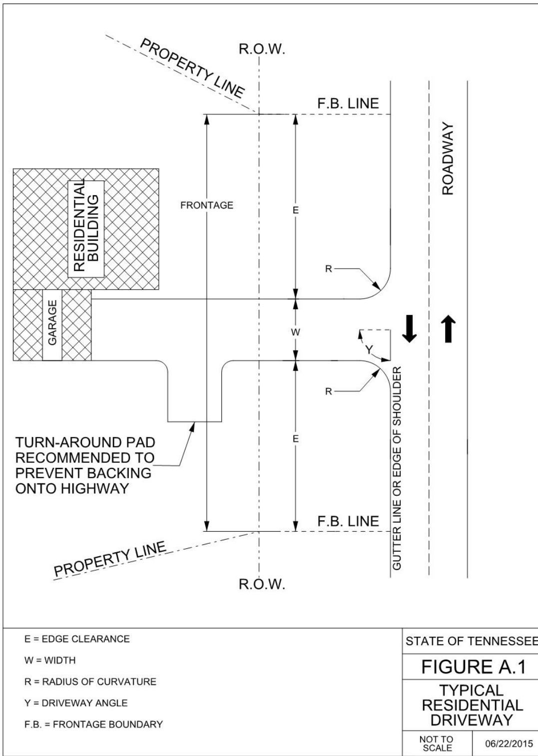
Figure A.1: Typical Residential Driveway
