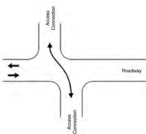
Figure 3-7: Adverse Jog Maneuver 9, 10
