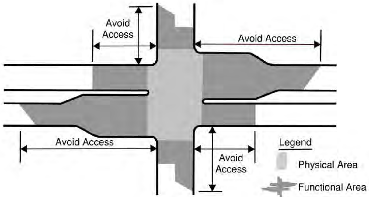
Figure 3-1: Intersection Functional Area [TRB, Access Management Manual, 2014] 3, 4
