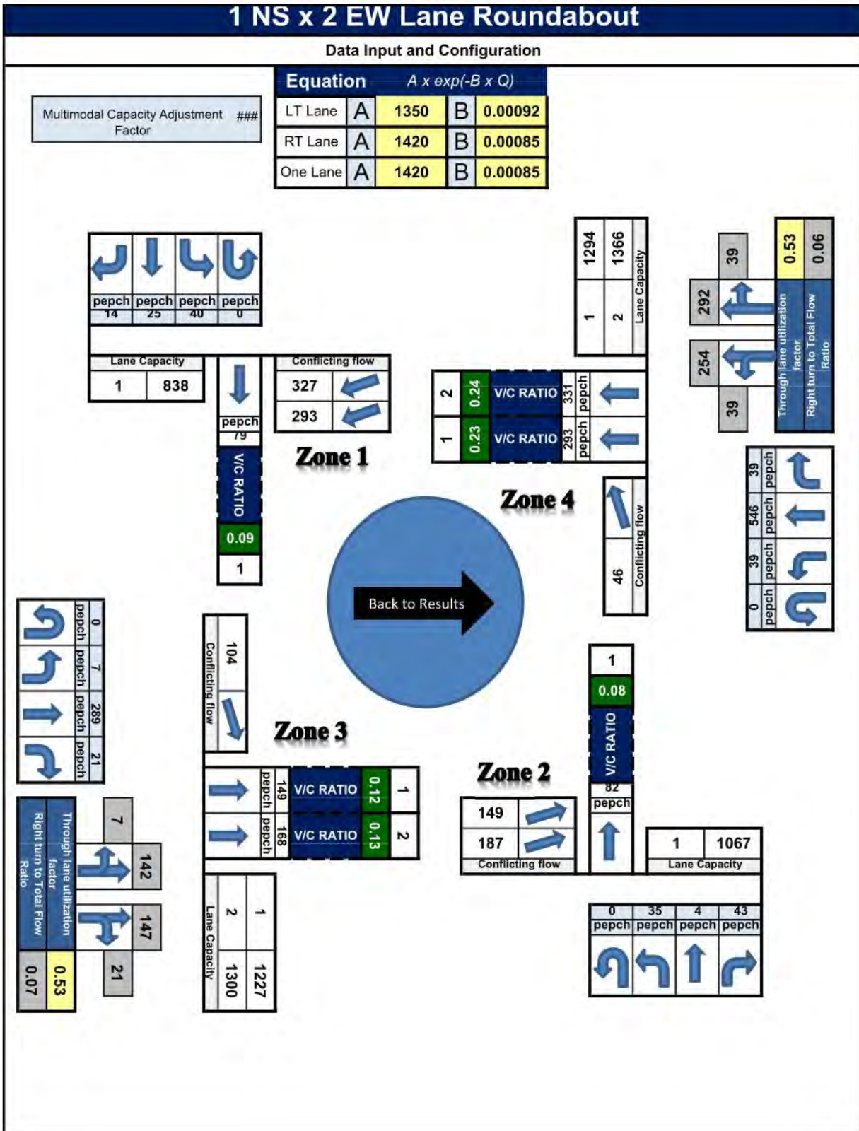
Figure 2-21: Roundabout Intersection Detailed Option Tab (2 of 2)
