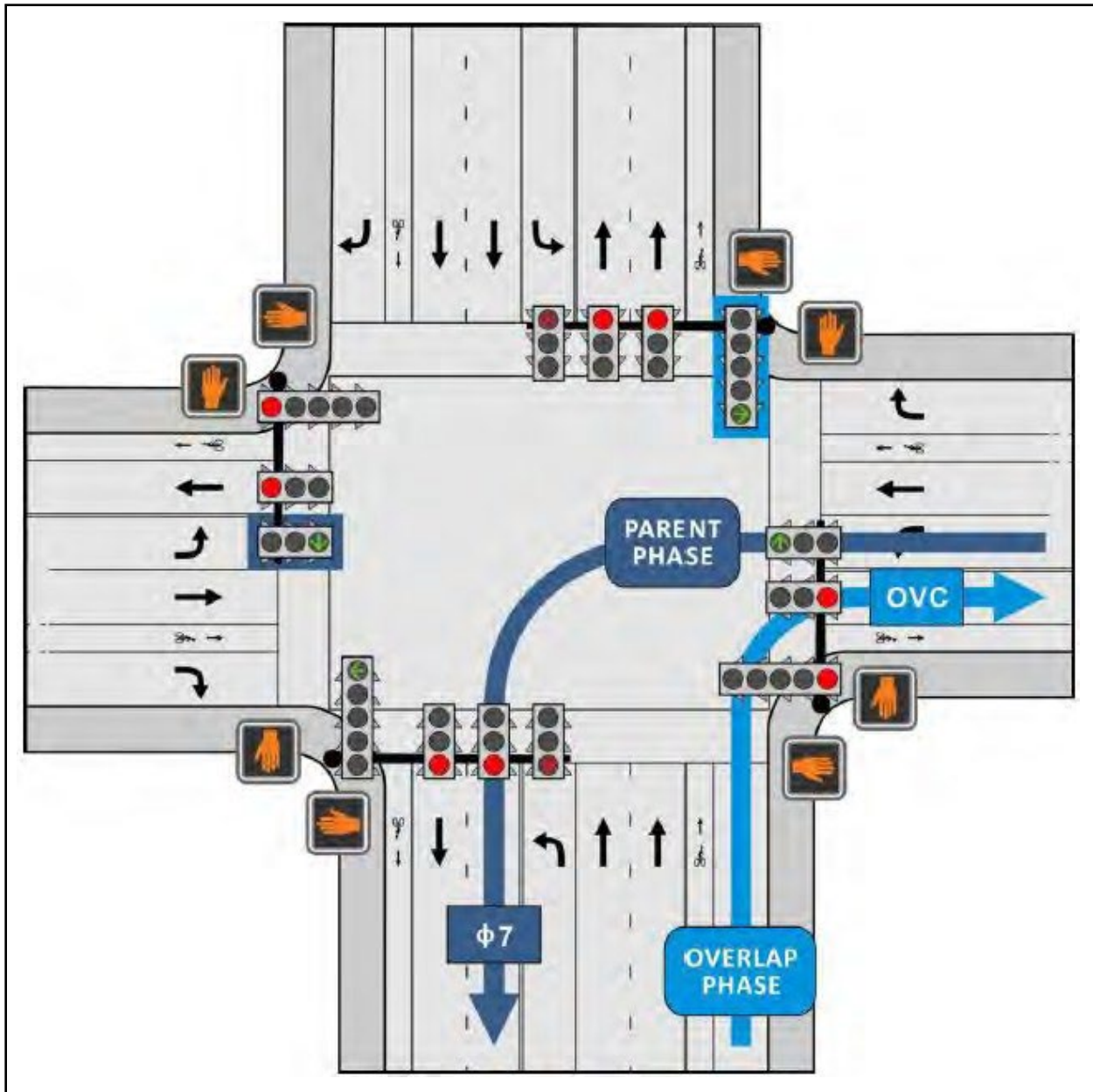
Figure 4.12 – Right-Turn Overlap Source: Traffic Signal Timing Manual
