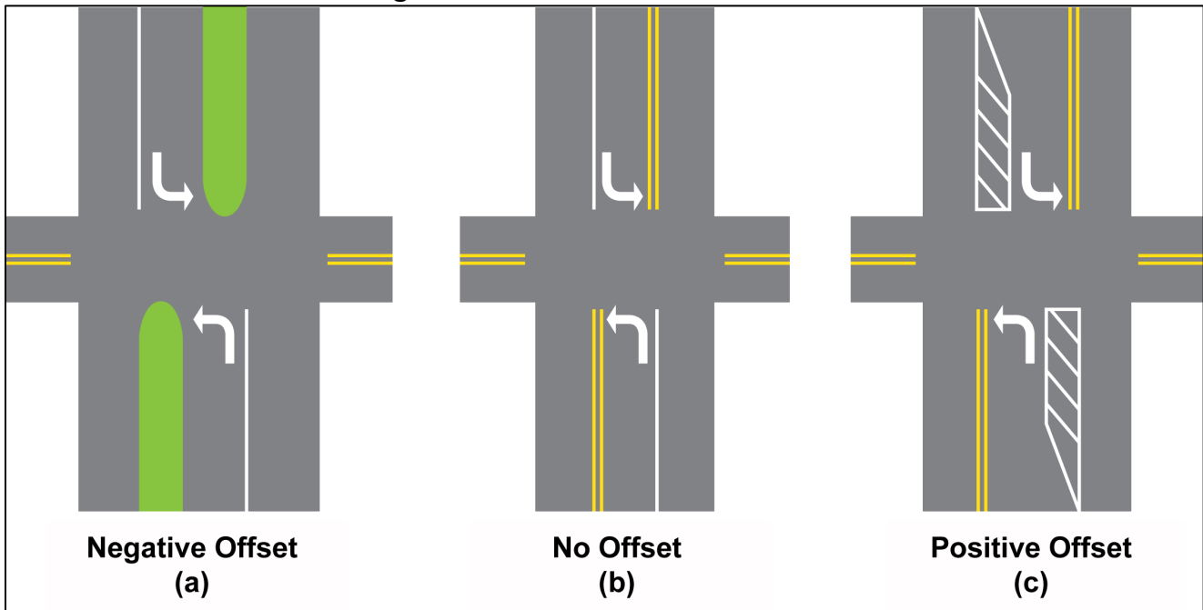
Figure 4.7 – Offset Left-Turn Lanes
