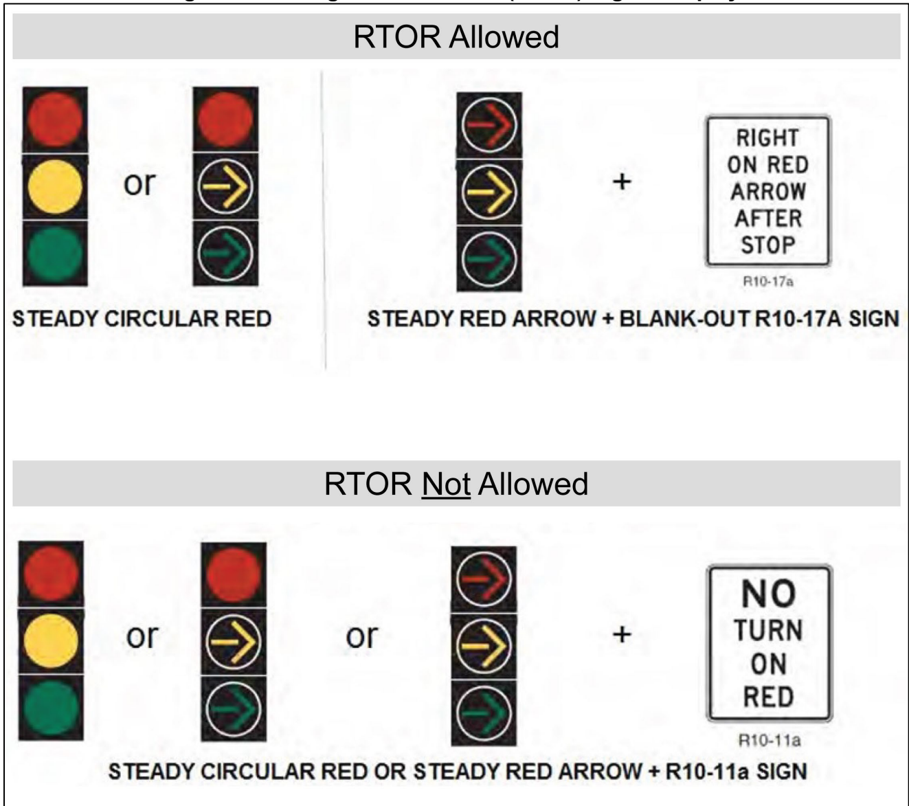
Figure 4.14 – Right-Turn On Red (RTOR) Signal Displays
