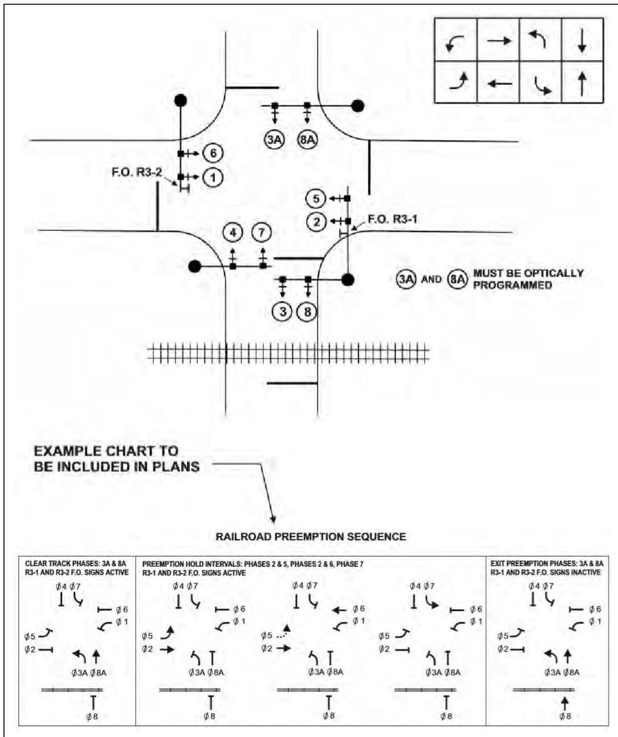
Figure 4.29 – Railroad Preemption Design Example
