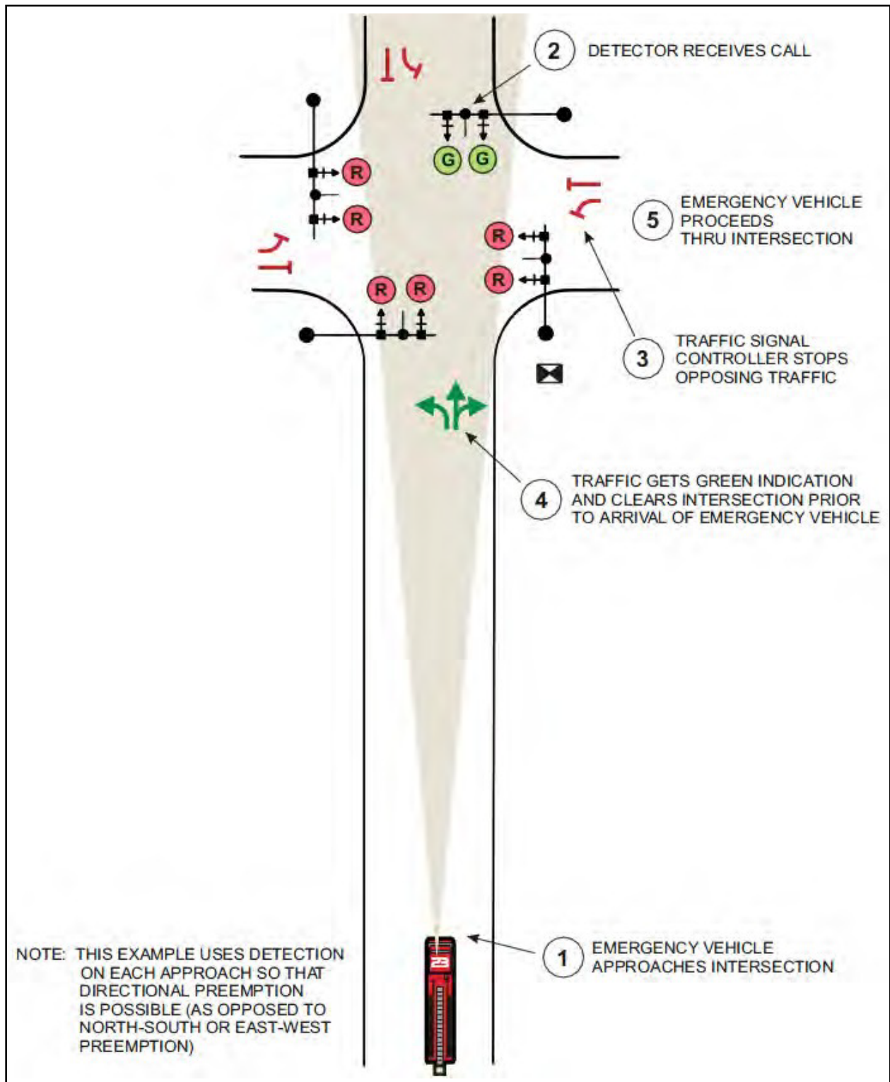
Figure 4.25 – Emergency Vehicle Preemption Sequence
