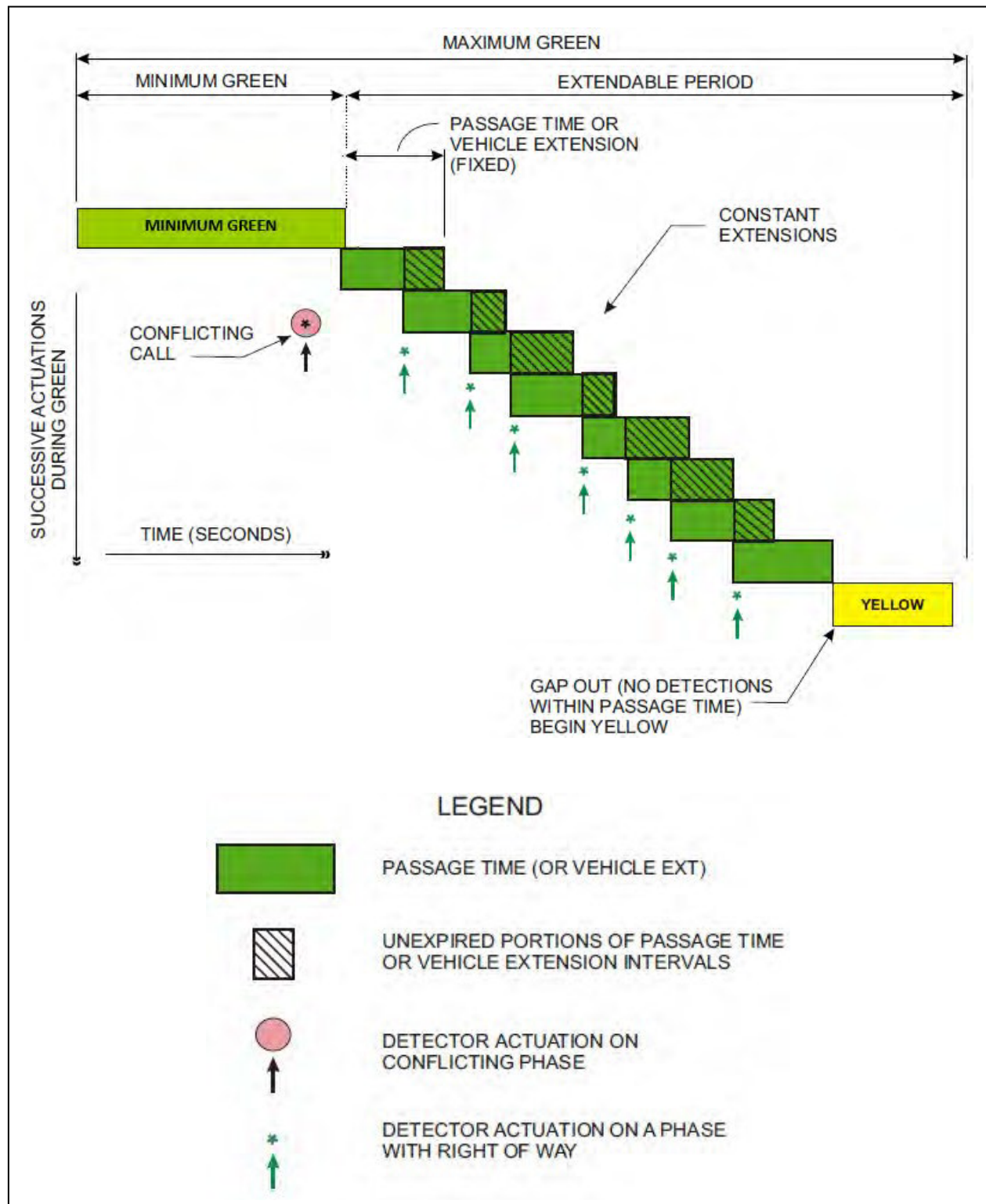
Figure 4.19 – Actuated Phase Operation Parameters
