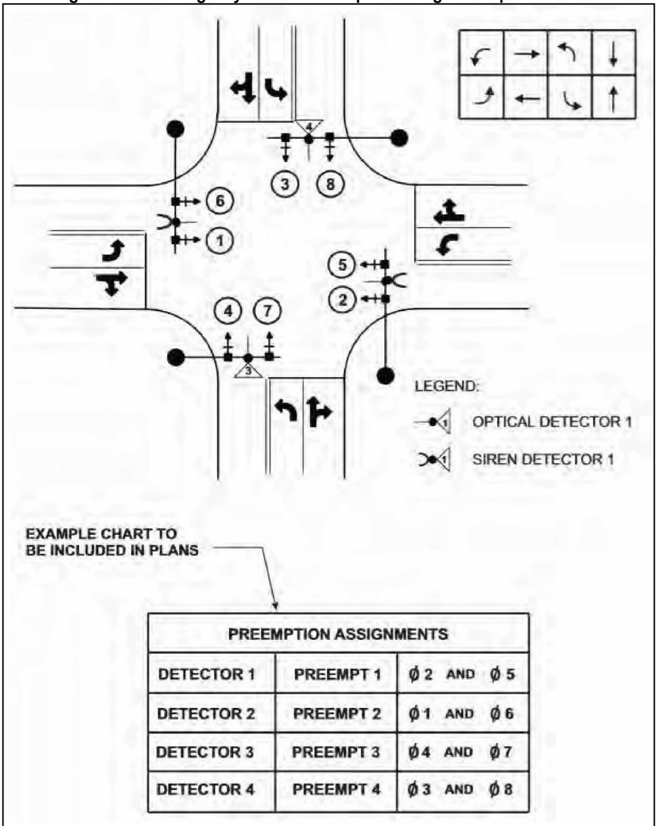
Figure 4.26 – Emergency Vehicle Preemption Design Example
