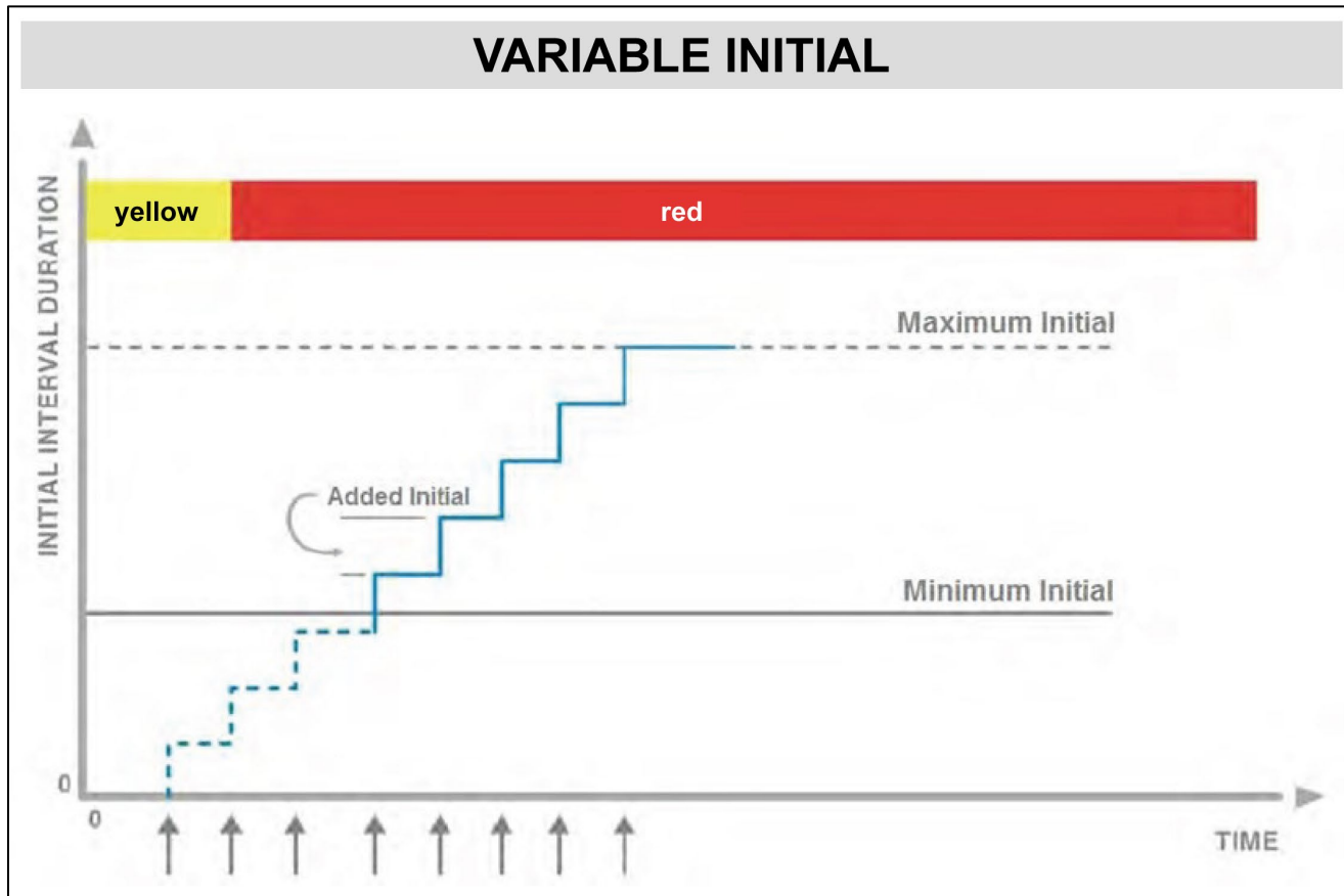
Figure 4.23 – Volume Density (Variable Initial)
