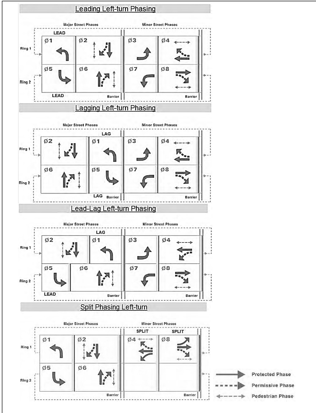
Figure 4.10 – Sequence of Left-Turn Phasing Source: Traffic Signal Timing Manual
