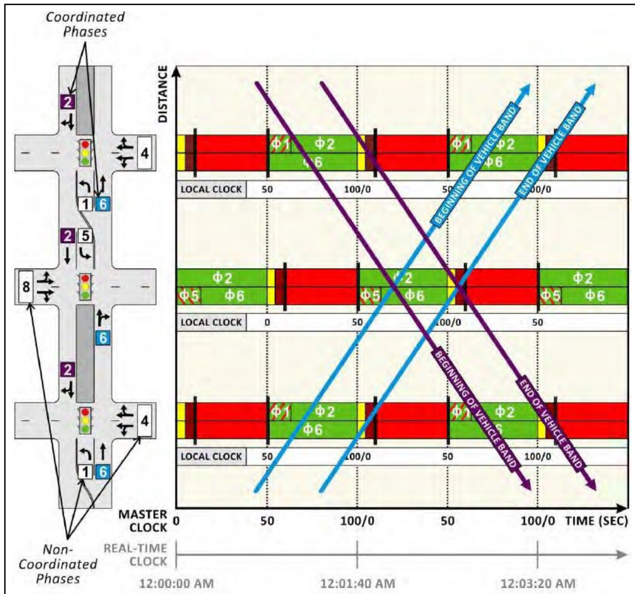
Figure 4.20 – Time-Space Diagram
