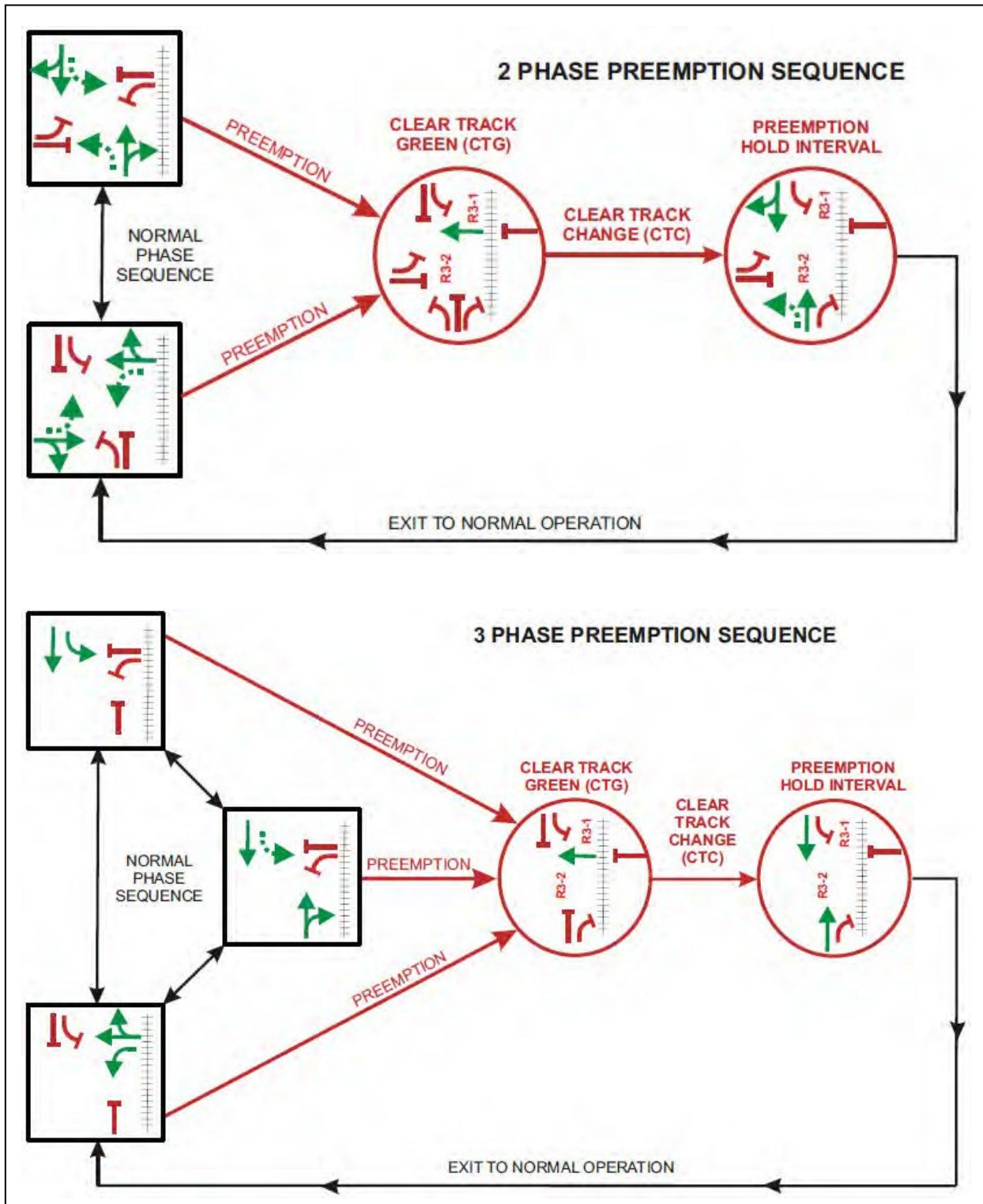
Figure 4.27 – Railroad Preemption Sequence (2 or 3-Phase Operation)
