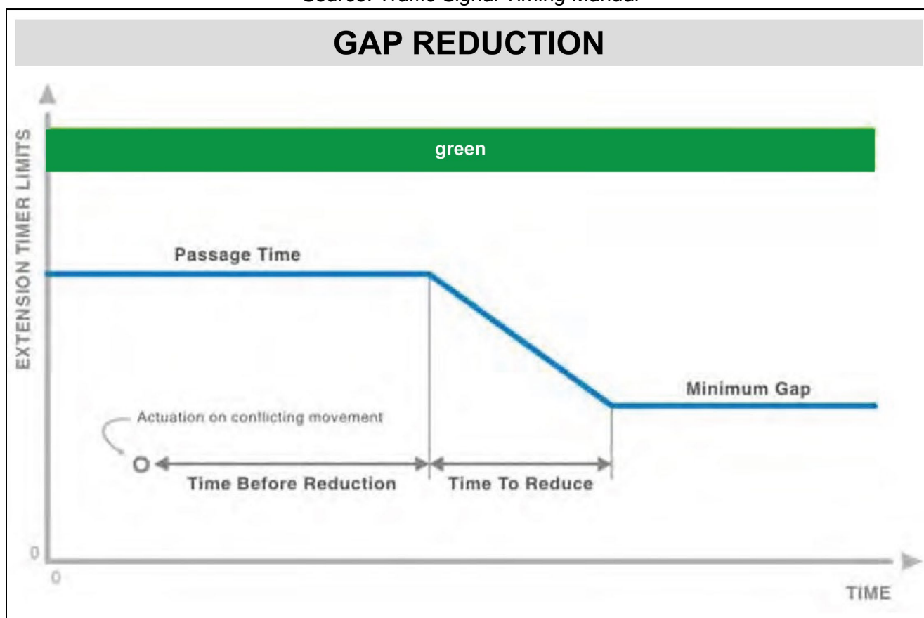
Figure 4.24 – Volume Density (Gap Reduction)
