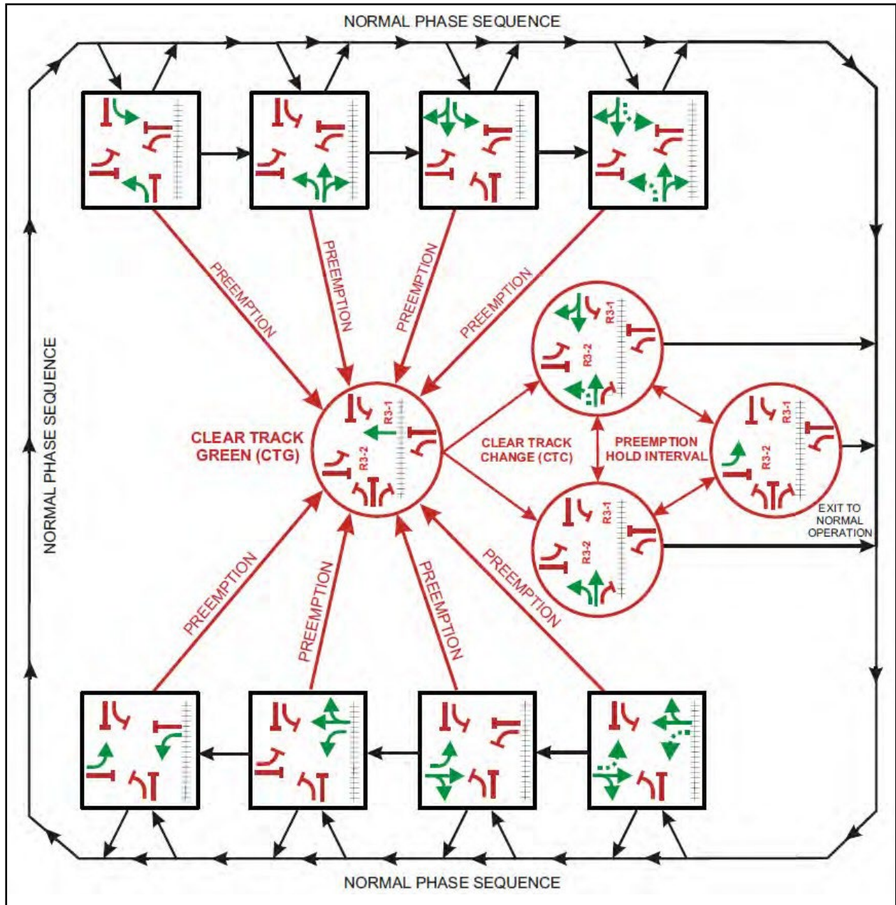
Figure 4.28 – Railroad Preemption Sequence (8-Phase Operation)
