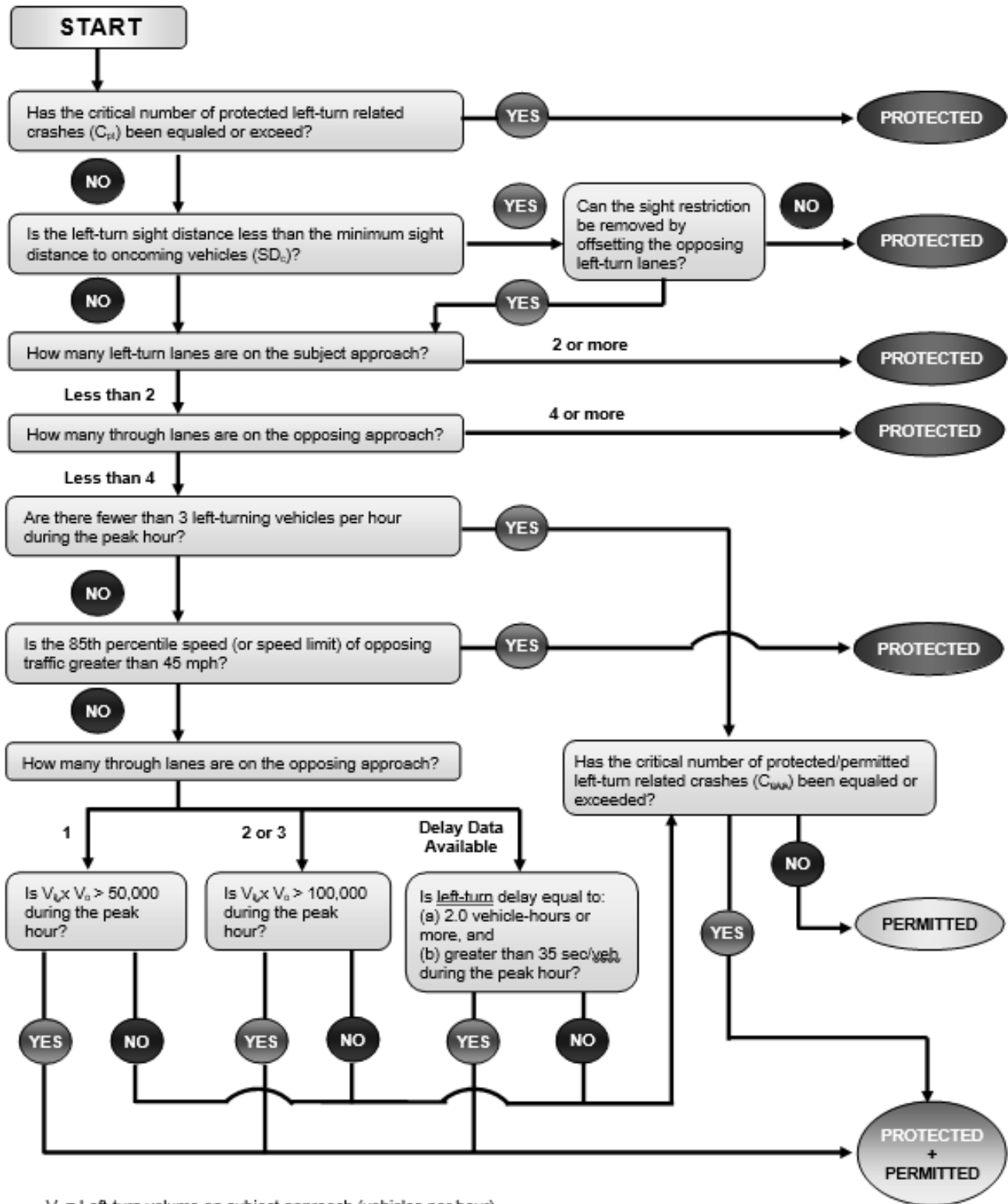
Figure 4.9 – Guidelines for Selecting Left-Turn Phasing
