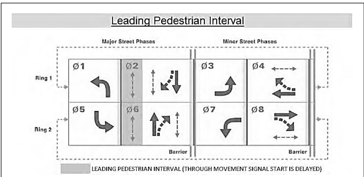
Figure 4.16 – Leading Pedestrian Interval
