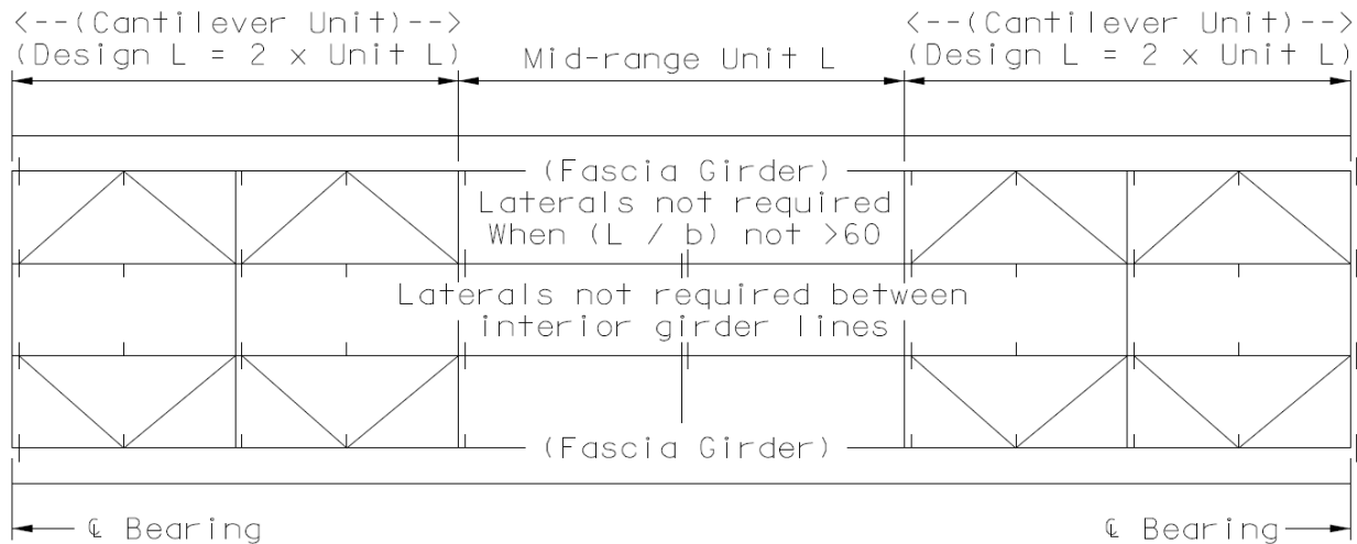
Figure 1. Partial Framing Plan
