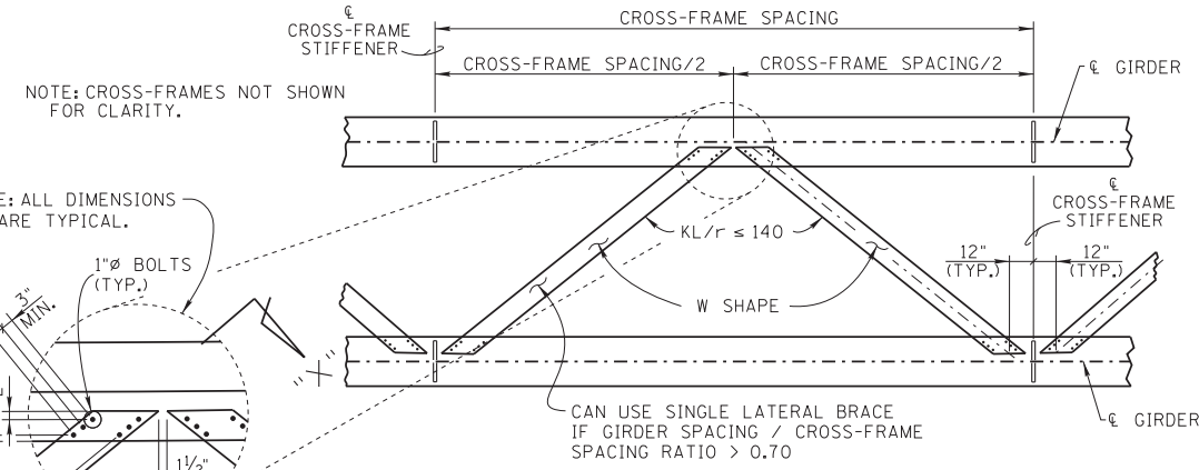
LATERAL BRACING DETAIL
