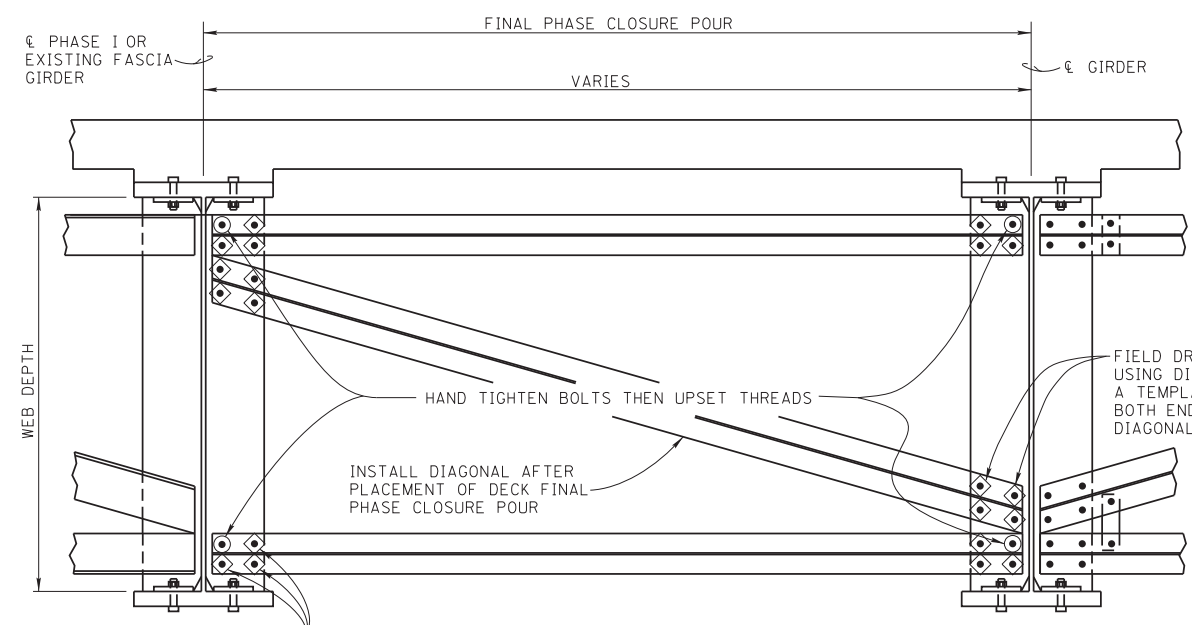
Z-FRAME DETAILS FOR CLOSURE POURS
