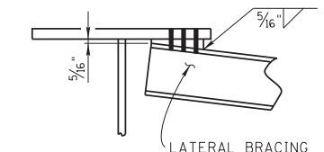
SECTION "X"-X"
