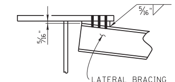
SECTION "X"- "X"
