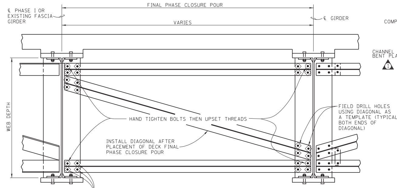
Z-FRAME DETAILS FOR CLOSURE POURS
