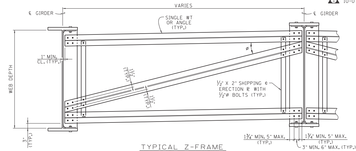
TYPICAL Z-FRAME
