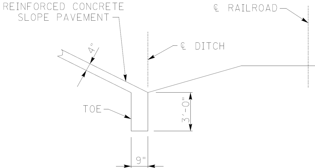
Figure 2. Slope Pavement Detail at Railroad Ditch
