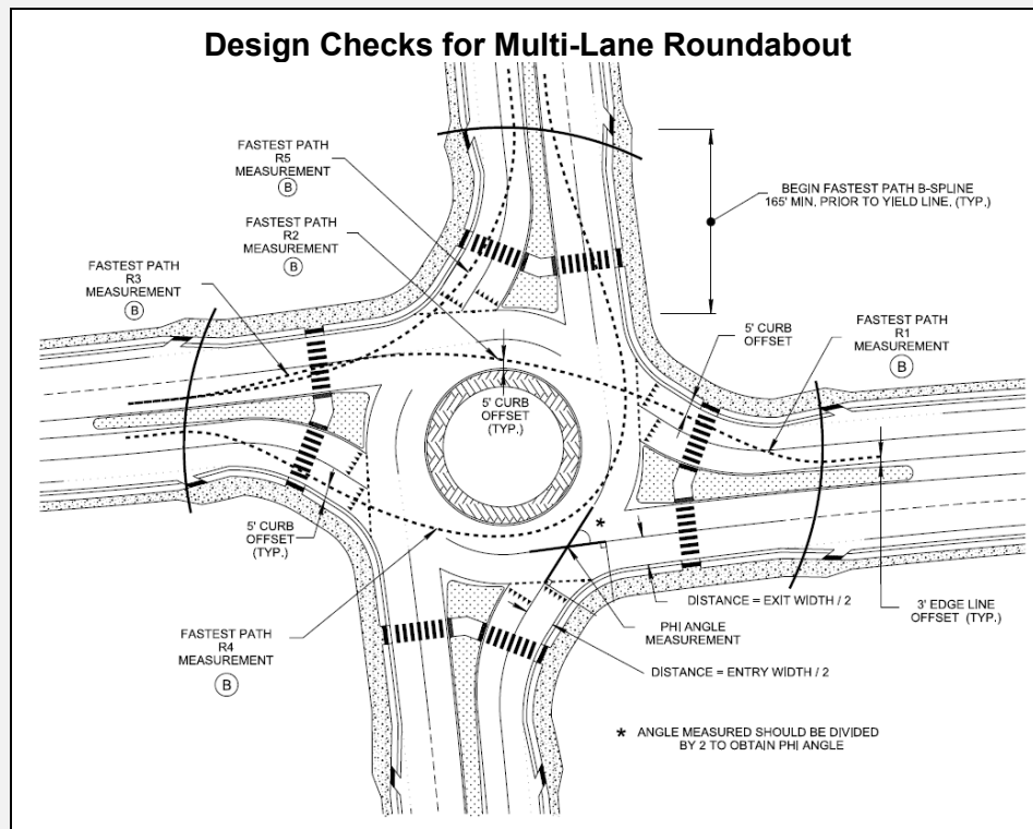
Figure 8 Design Checks for Single and Multi-Lane Roundabouts Adapted from: Roundabouts: An Informational Guide, Second Edition (NCHRP, 2010)
