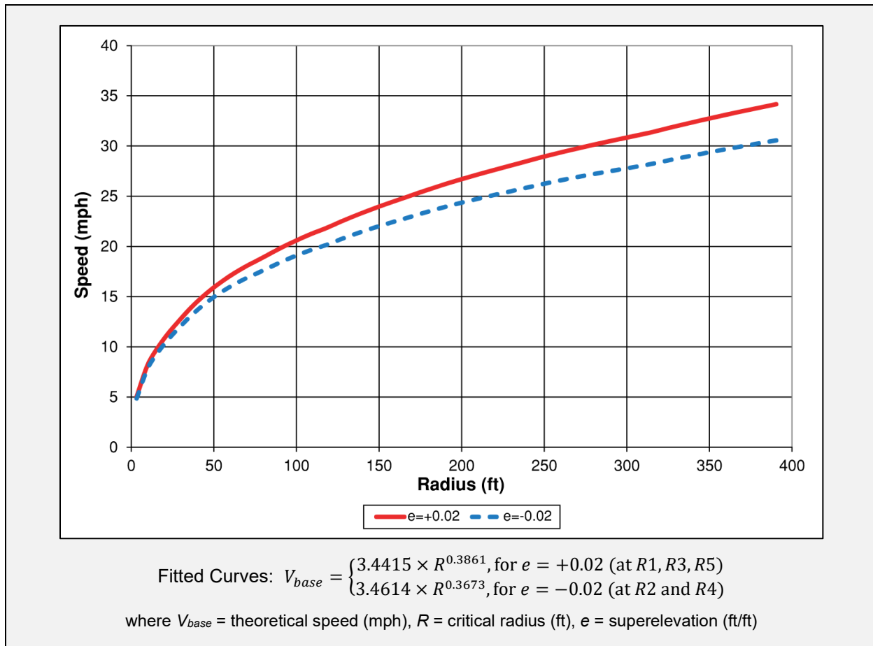
Figure 9 Speed-Radius Relationship
