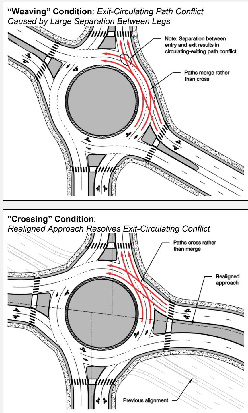
Figure 5 Example of Vehicle Exit-Circulating Path Conflict and Desirable Path Alignment Adapted from: Roundabouts: An Informational Guide, Second Edition (NCHRP, 2010)
