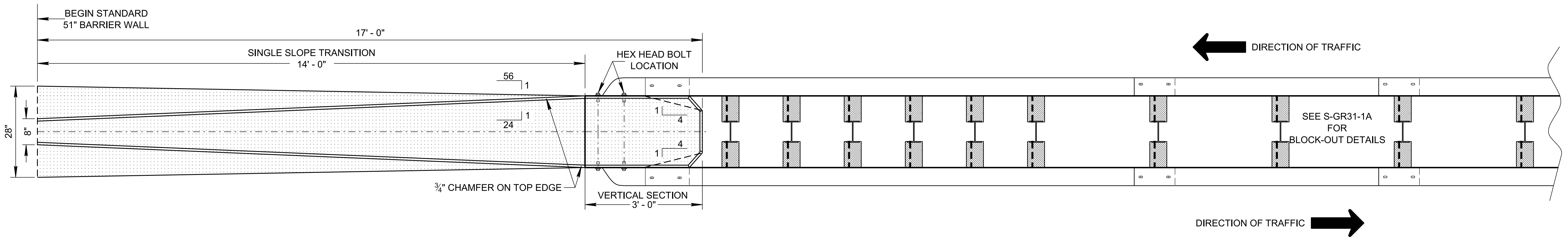
PLAN VIEW
