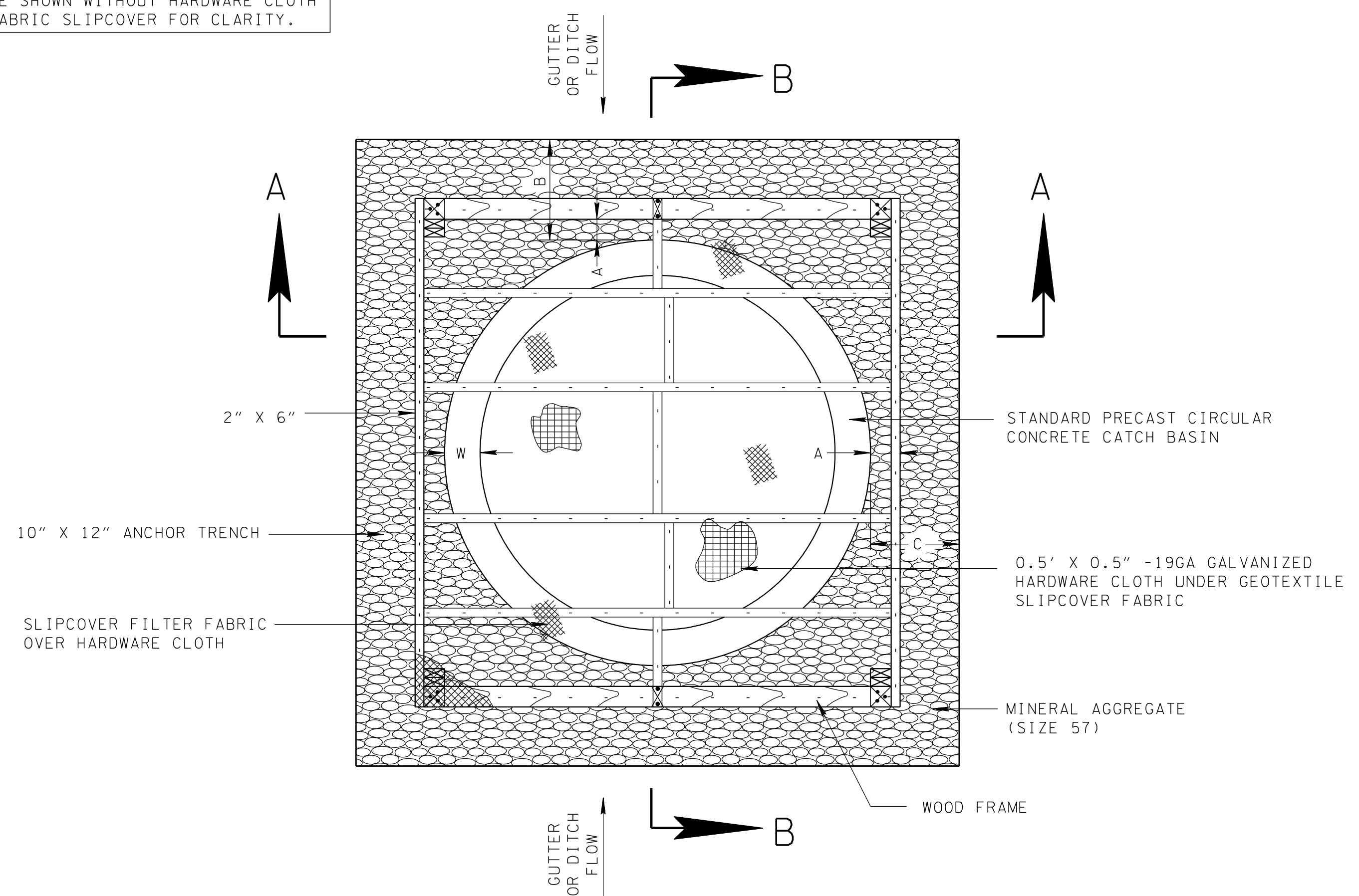
PLAN VIEW - CATCH BASIN FILTER ASSEMBLY N.T.S.
