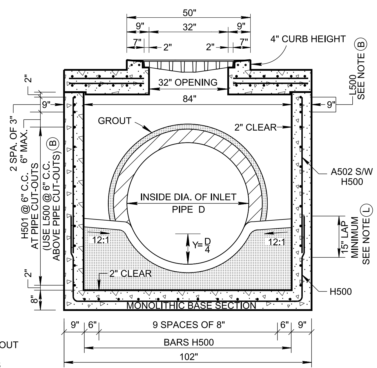
SECTION B-B
