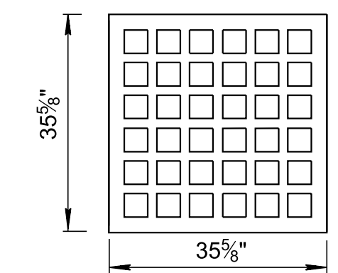
GRATE UNIT NO. 42 (SEE STD. DWG. D-CBB-42 FOR GRATE DETAILS)
