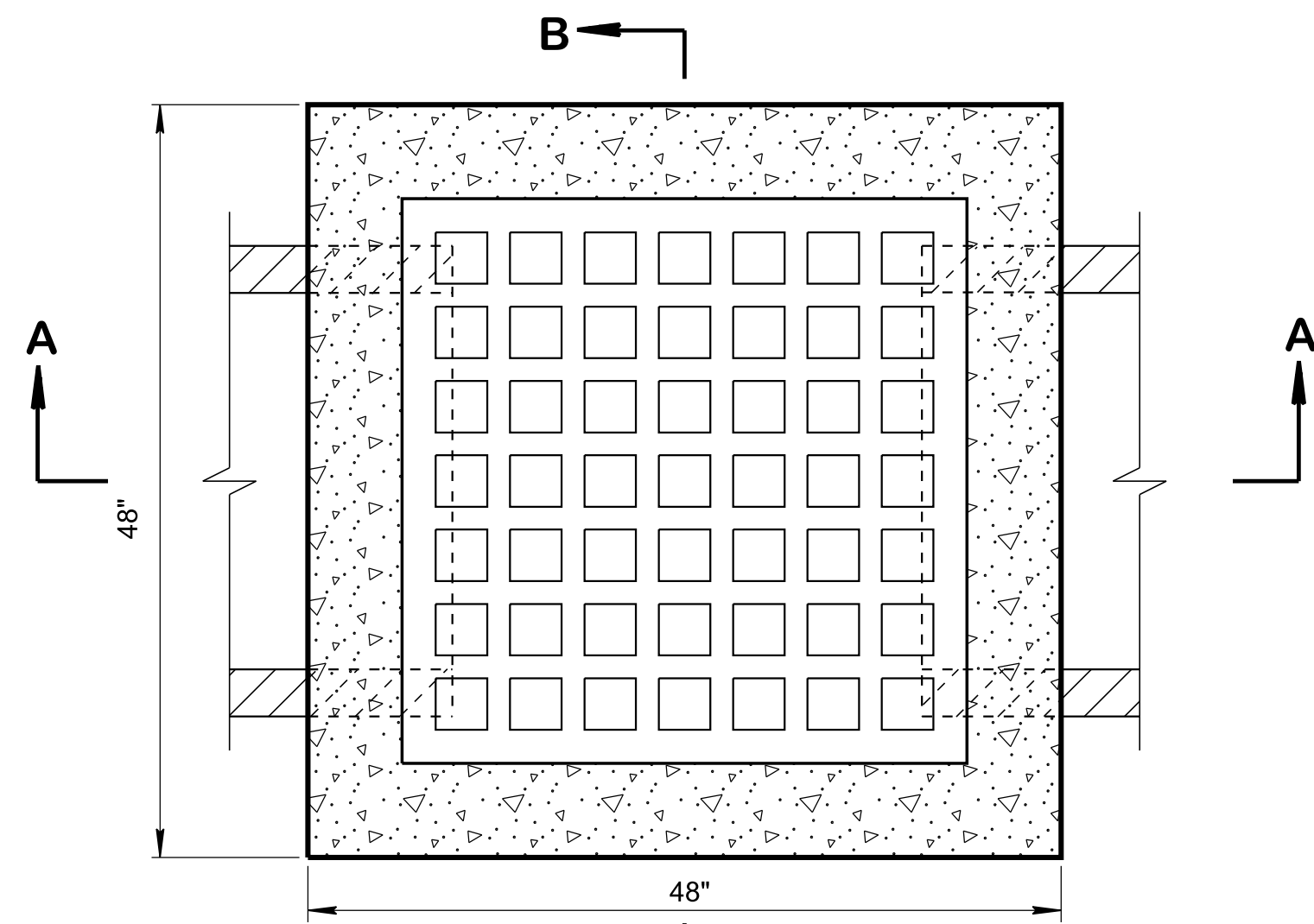
PLAN VIEW
