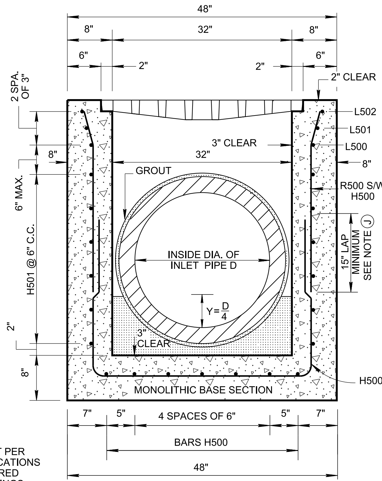
SECTION B-B
