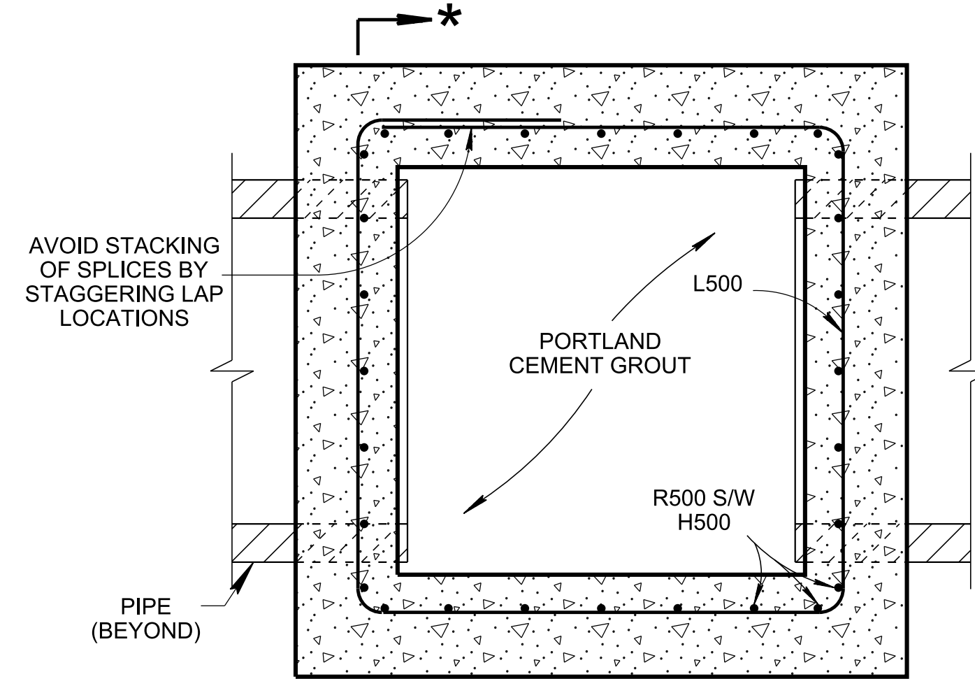
SECTION C-C
