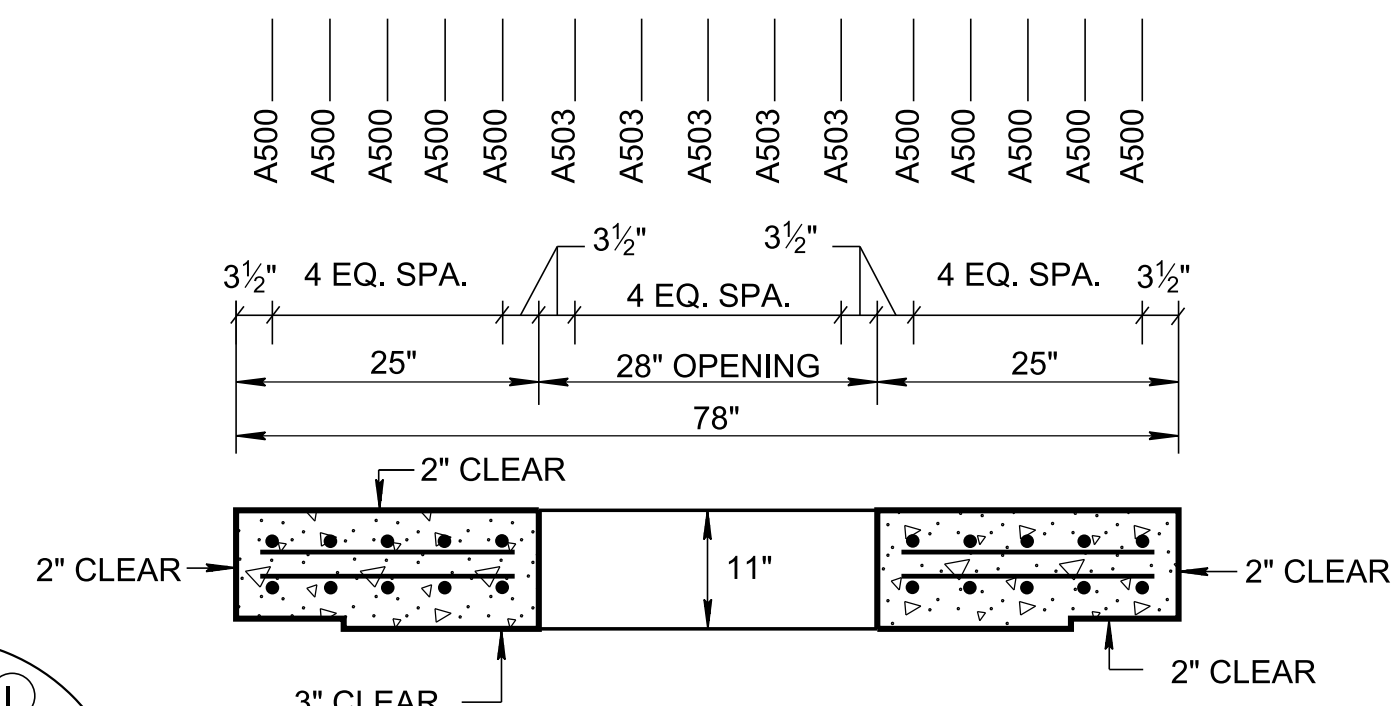
SECTION C-C
