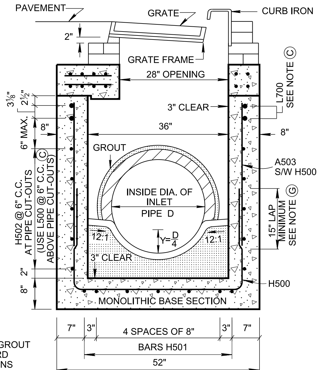
SECTION B-B
