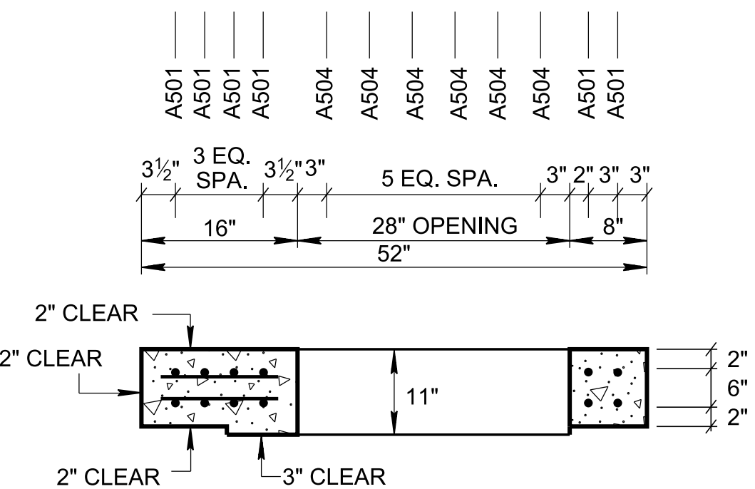
SECTION C-C
