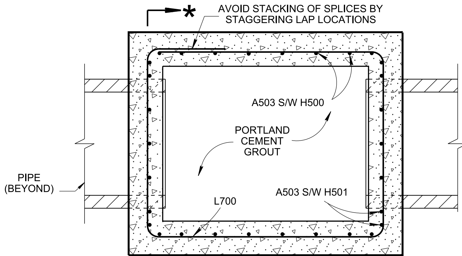
SECTION *-* ELEV. VIEW IS PROVIDED ON STANDARD DRAWING D-CB-99 SHOWING REINFORCEMENT REQUIREMENTS AROUND PIPE OPENINGS
