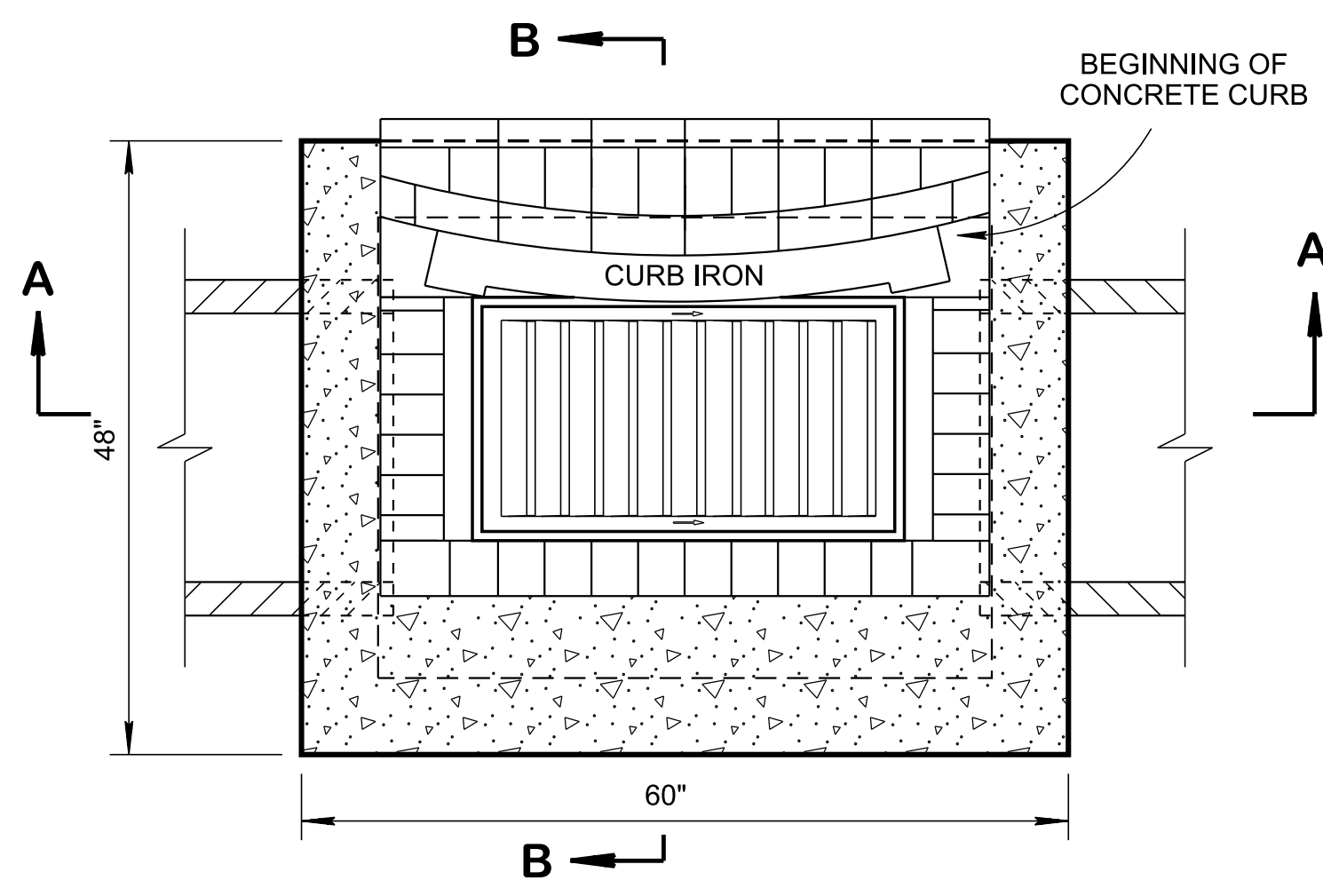
PLAN VIEW
