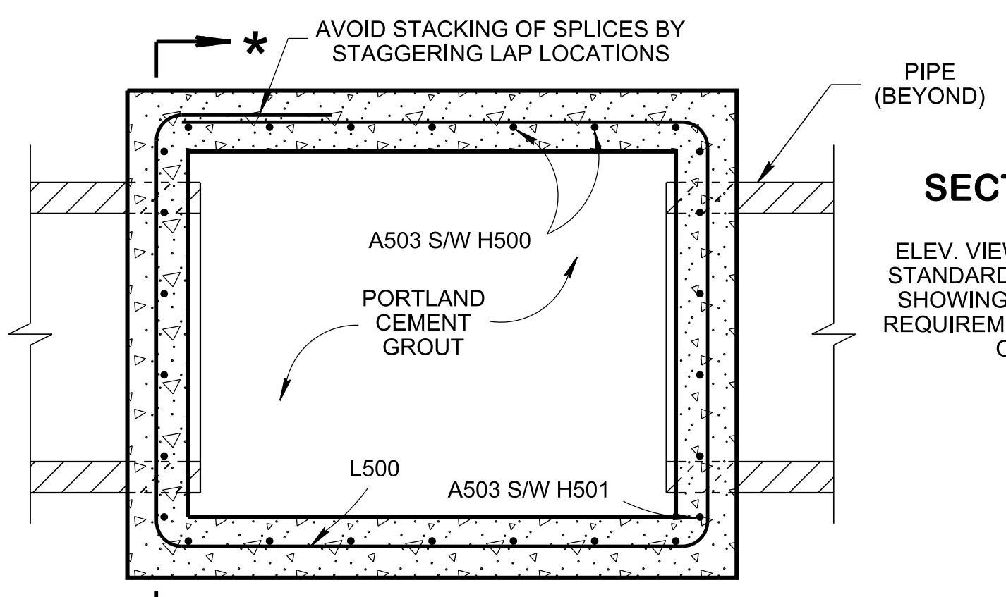
SECTION E-E
