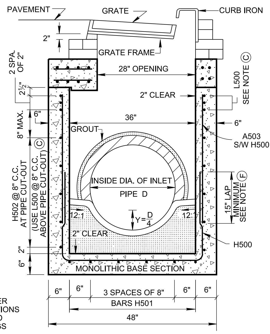
SECTION B-B
