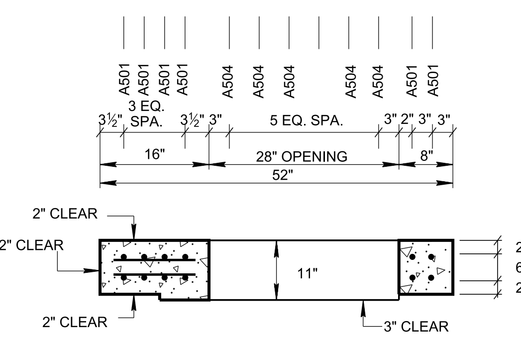
SECTION C-C
