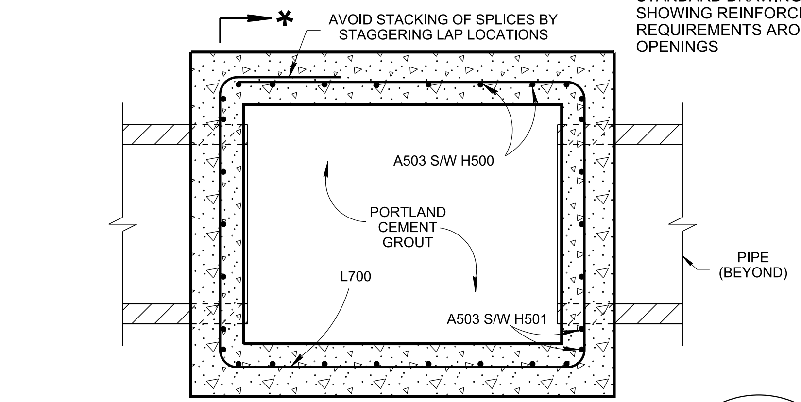
SECTION E-E
