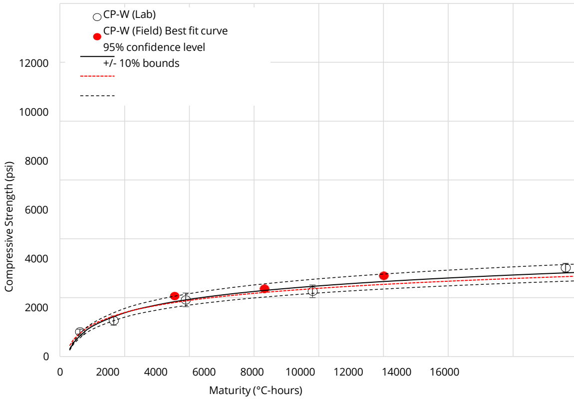
Figure 4-11 Field verification of Class CP-W mix.
