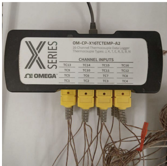
Figure 3-5 A 16-channel data logger for monitoring of 8 different concrete mixes.
