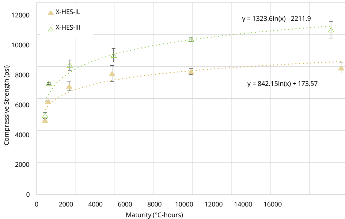
Figure 4-5 Strength-maturity relationship for Class X-HES mixes (datum temperature = 32 °F (0 °C)).
