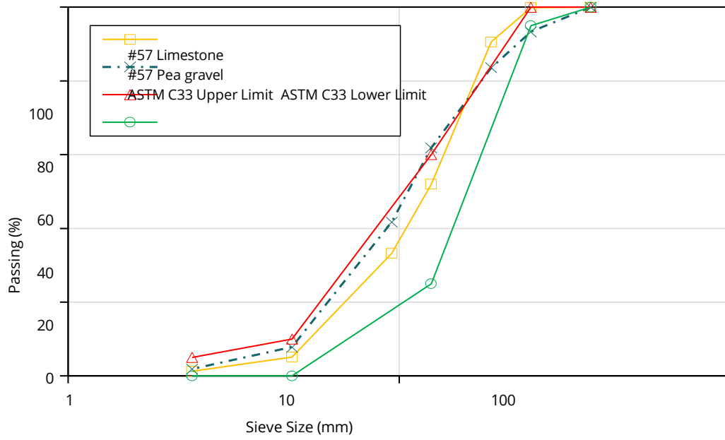
Figure B-2 Gradation of coarse aggregates.
