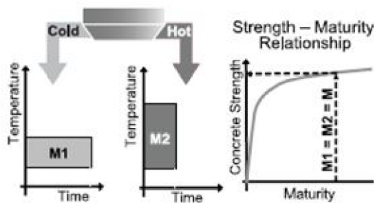
e 2-1 Maturity concept (Kaburu et al. 2016).
