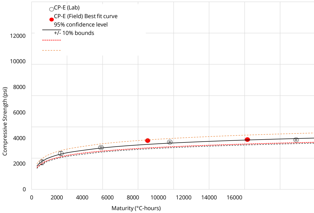
Figure 4-10 Field verification of Class CP-E mix.
