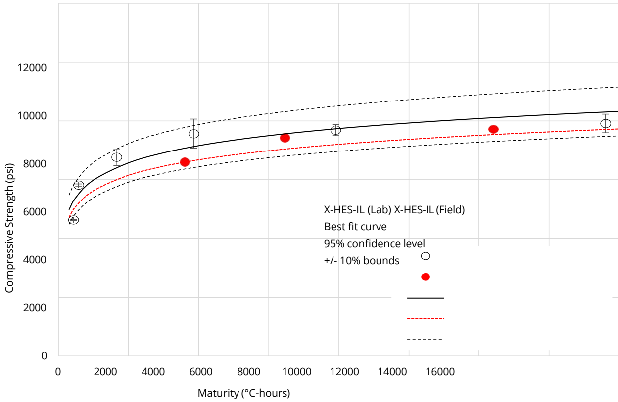
Figure 4-12 Field verification of Class X-HES-IL mix.
