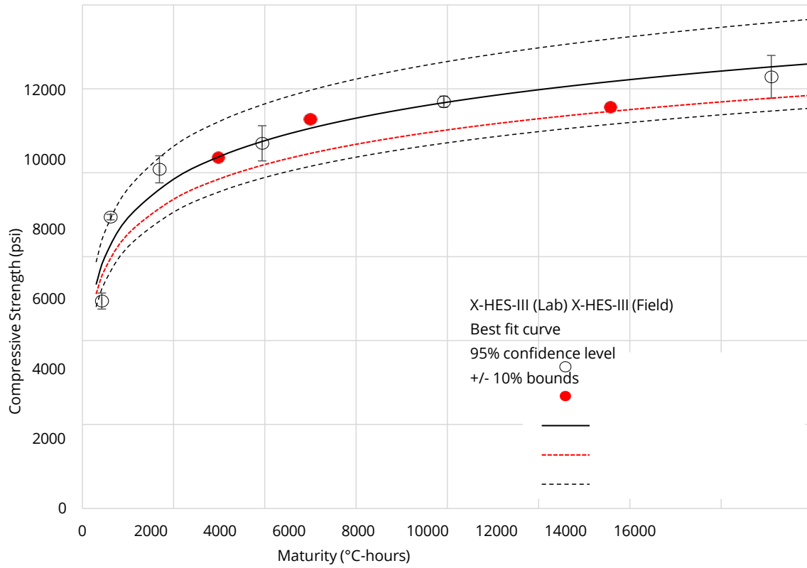
Figure 4-13 Field verification of Class X-HES-III mix.
