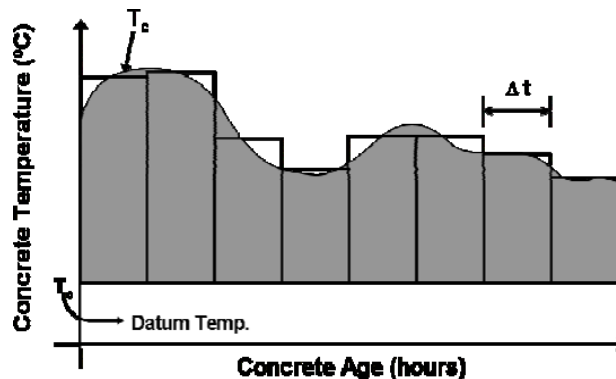
Figure 2-2 Typical temperature-time relationship (Nixon et al. 2008).
