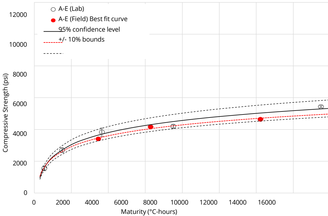
Figure 4-6 Field verification for Class A-E mix.
