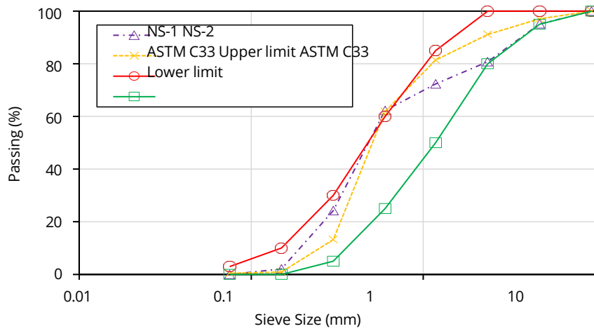
Figure B-1 Gradation of fine aggregates.
