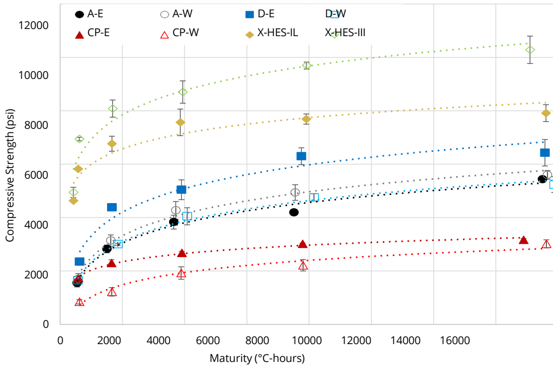
Figure 4-1 Strength-maturity relationships for all 8 mixes (datum temperature = 32 °F (0 °C)).
