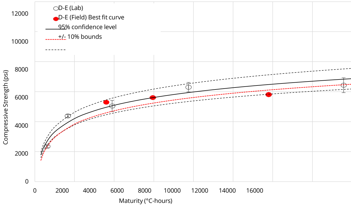
Figure 4-8 Field verification of Class D-E mix.
