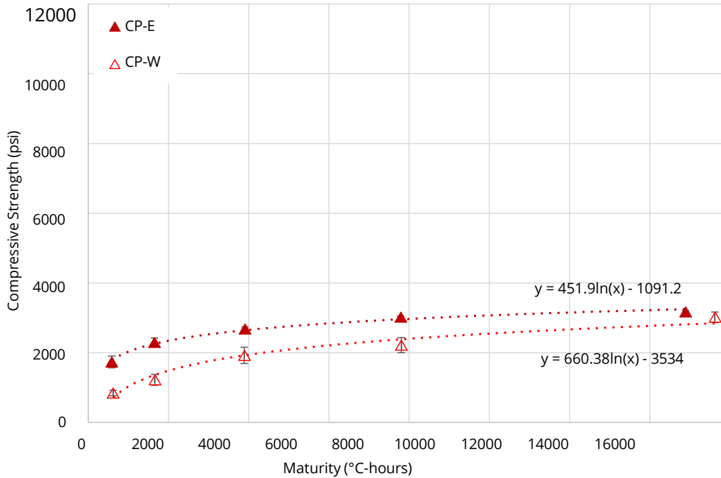
Figure 4-4 Strength-maturity relationship for Class CP mixes (datum temperature = 32 °F (0 °C)).
