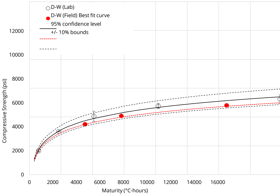
Figure 4-9 Field verification of Class D-W mix.
