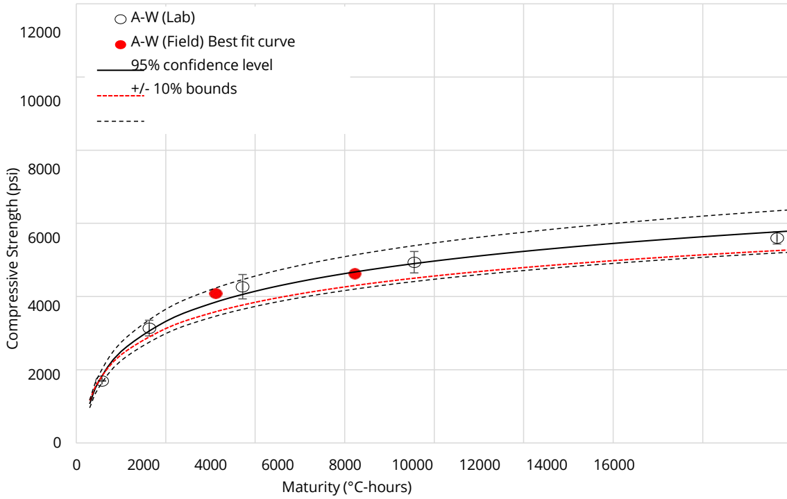
Figure 4-7 Field verification for Class A-W mix.
