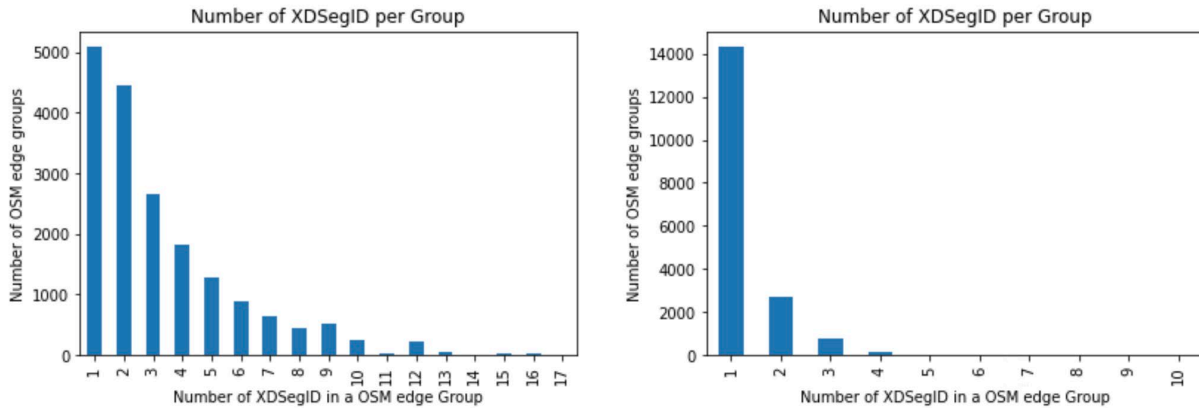
Figure 3: Number of Multiple INRIX Segments matches per OSM edge before (left) and after (right) geospatial join within each OSM edge group
