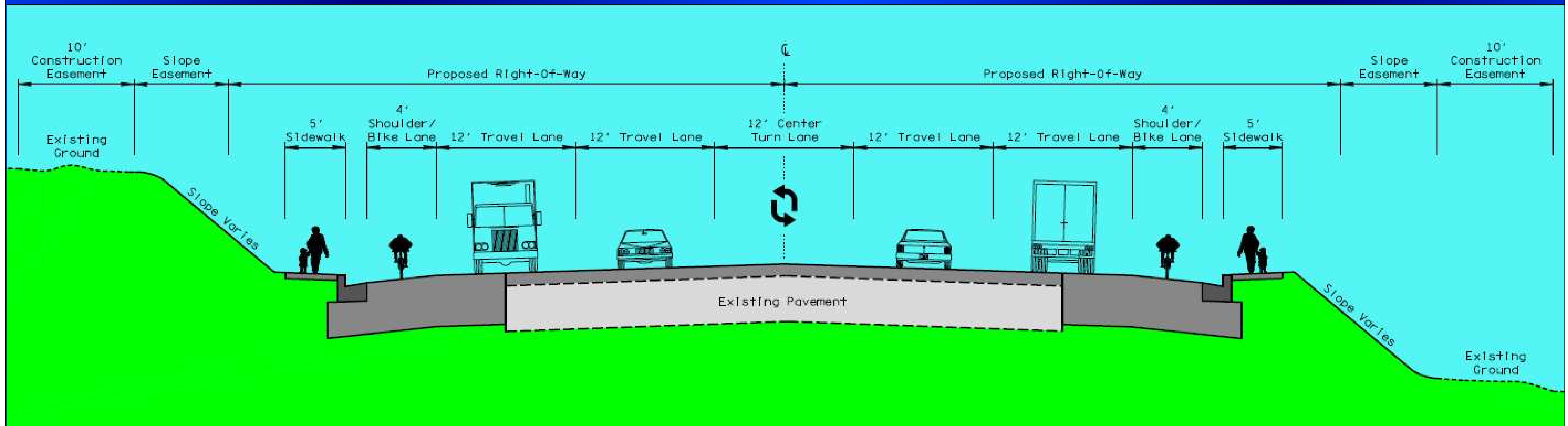
TYPICAL SECTION - WIDENING
