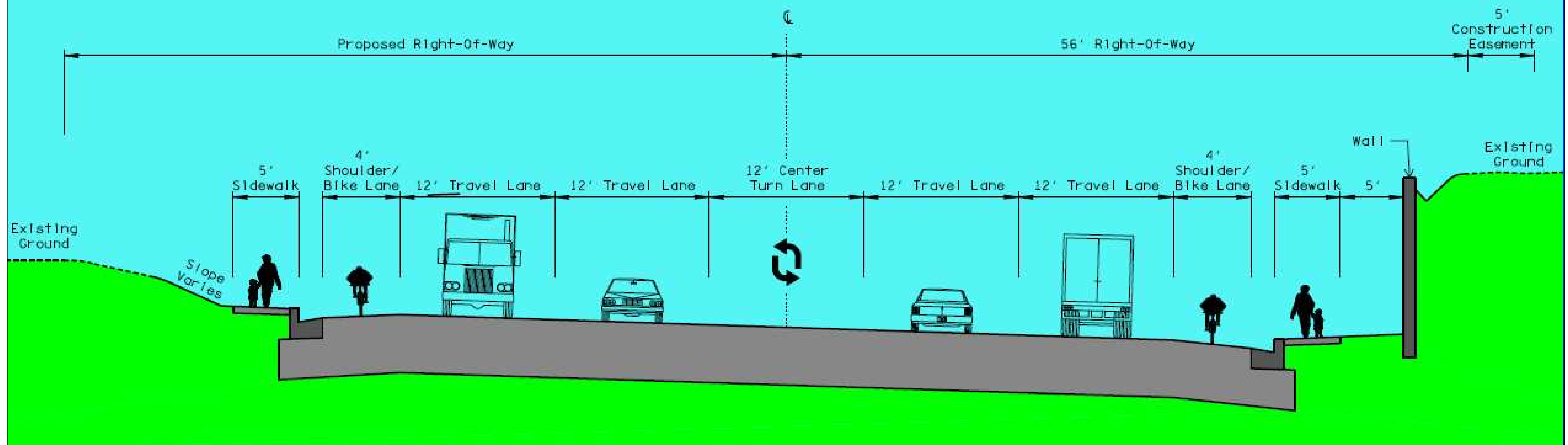
TYPICAL SECTION – AT CREST OF HILL
