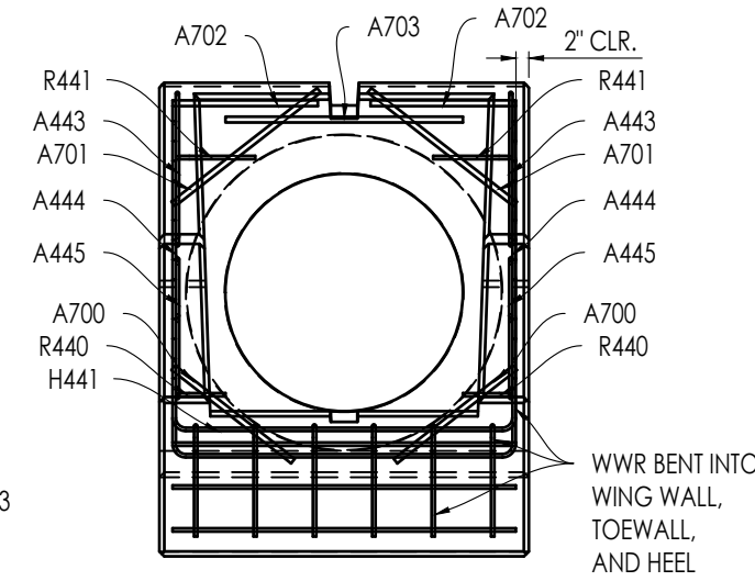
END ELEVATION SCALE 3/8" = 1'-0"
