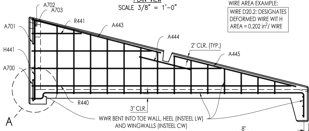
WINGWALL ELEVATION SCALE 3/8" = 1'-0"
