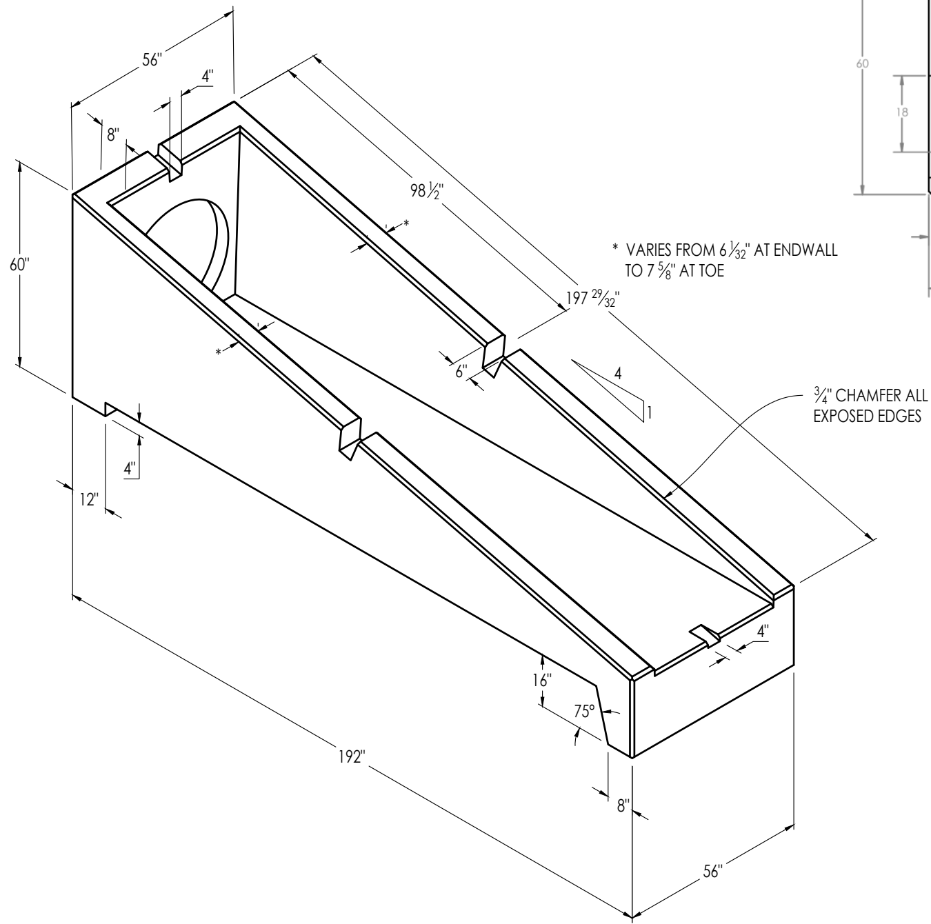
ISOMETRIC VIEW SHOWING DIMENSIONS, 4:1 SLOPE
