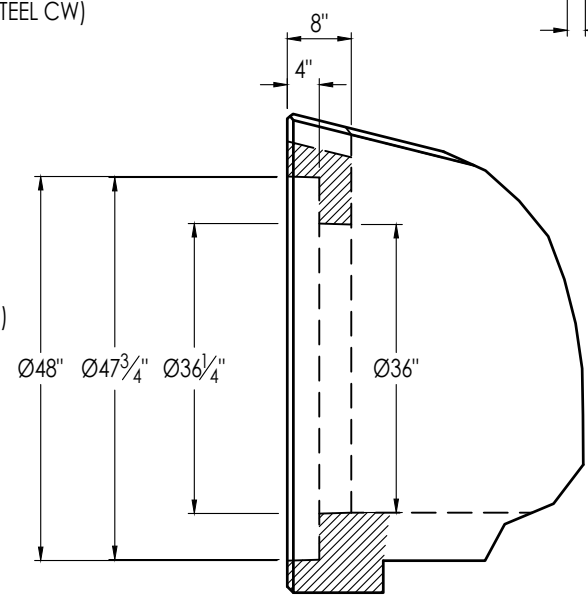
PIPE OPENING DETAIL SCALE 1/2" = 1'-0"
