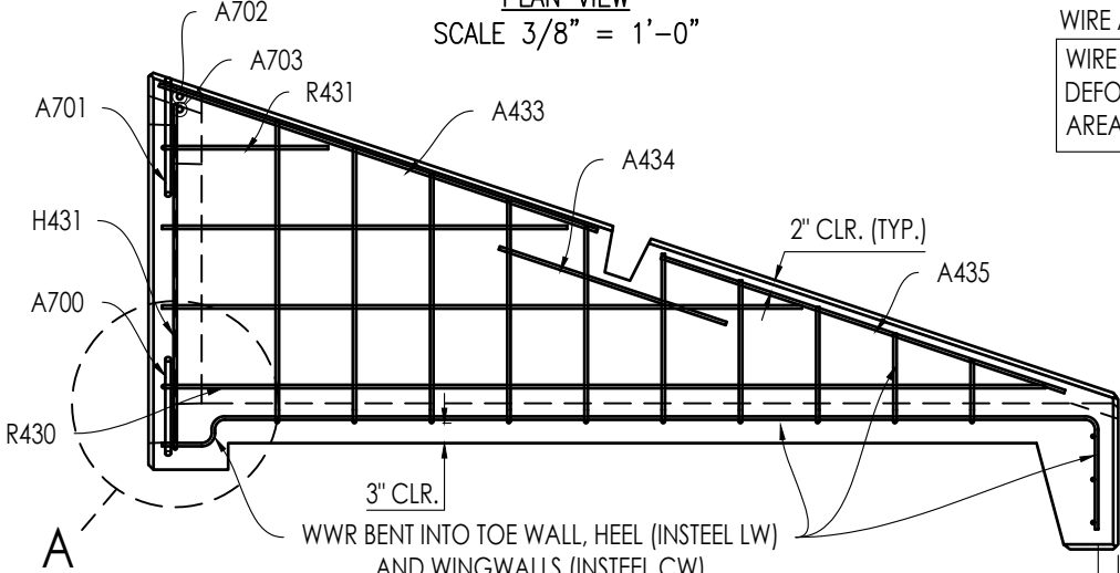
WINGWALL ELEVATION SCALE 3/8" = 1'-0"
