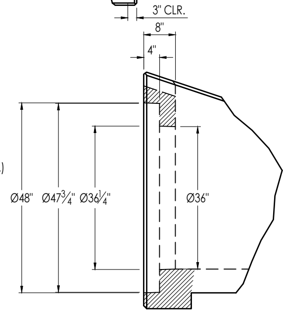
PIPE OPENING DETAIL SCALE 1/2" = 1'-0"
