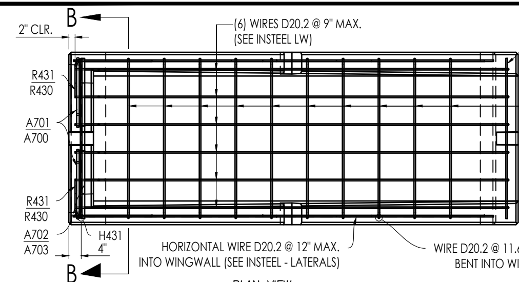
PLAN VIEW SCALE 3/8" = 1'-0"
