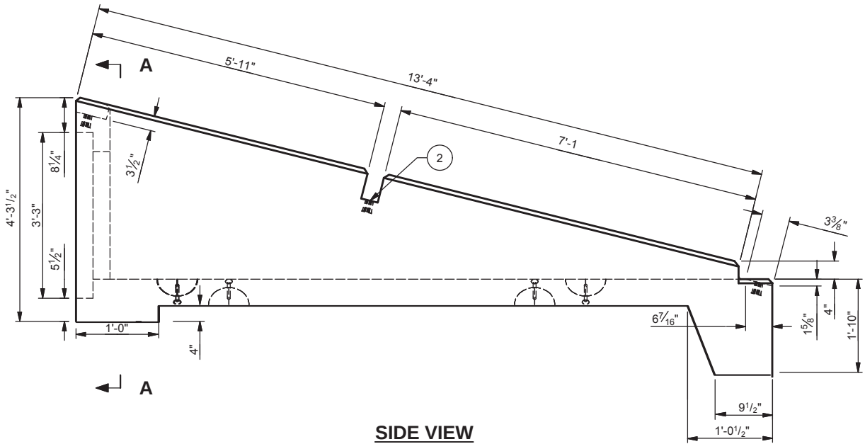
SIDE VIEW SCALE 3/8"=1'-0"
