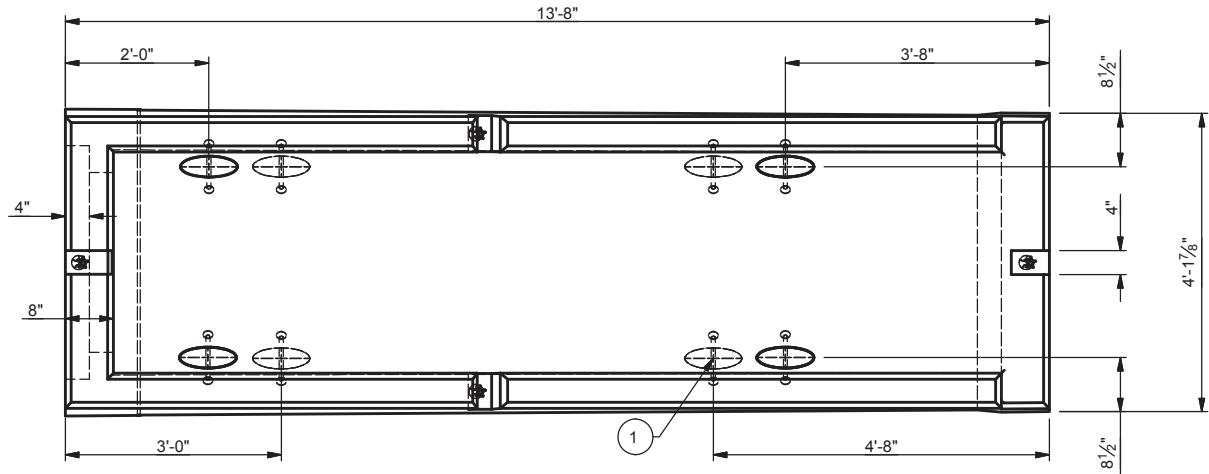
PLAN VIEW SCALE 3/8"=1'-0"
