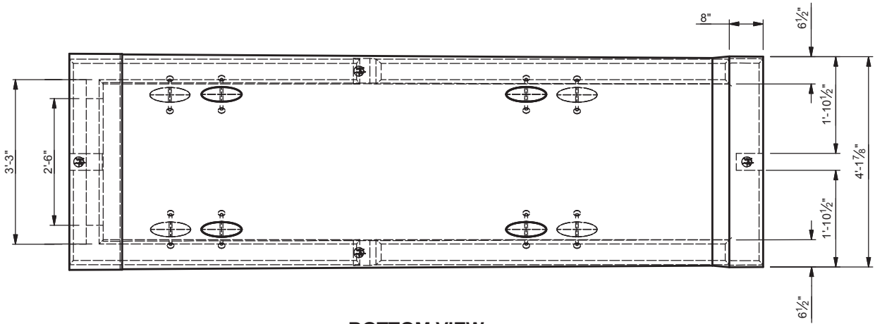
BOTTOM VIEW SCALE 3/8"=1'-0"
