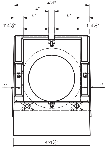
FRONT VIEW SCALE 3/8"=1'-0"
