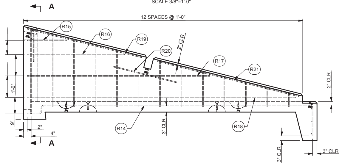
SIDE VIEW SCALE 3/8"=1'-0"
