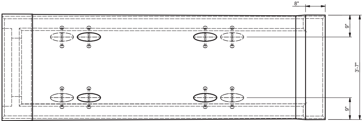
BOTTOM VIEW SCALE 1/2"=1'-0"
