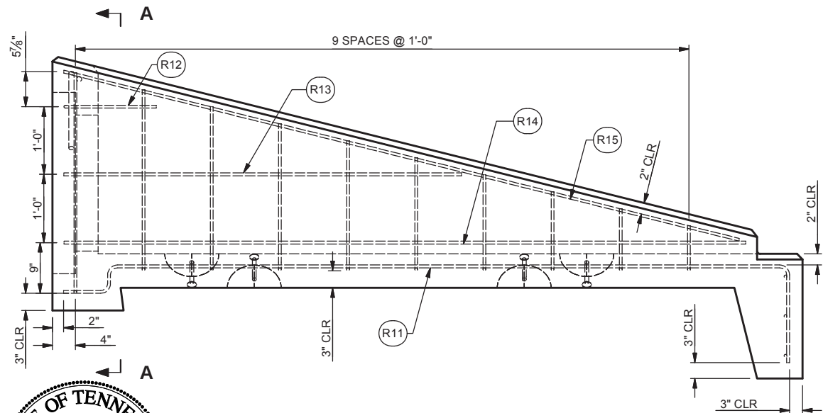
SIDE VIEW SCALE 1/2"=1'-0"
