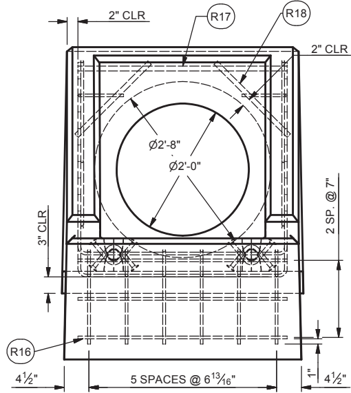
FRONT VIEW SCALE 1/2"=1'-0"
