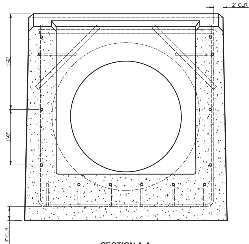
SECTION A-A SCALE 1"=1'
