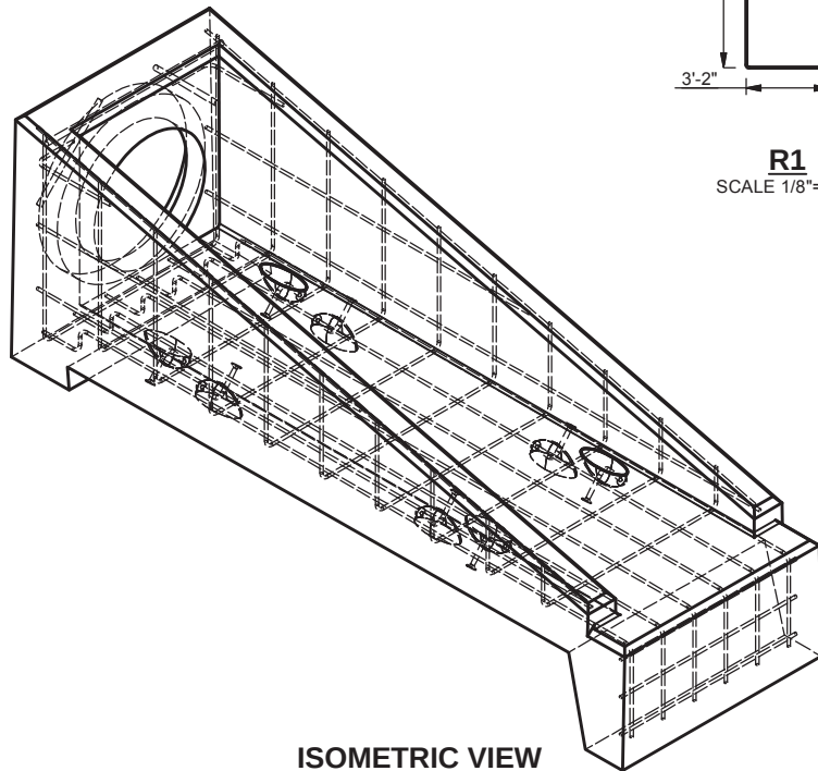
ISOMETRIC VIEW SCALE 3/8"=1'-0"
