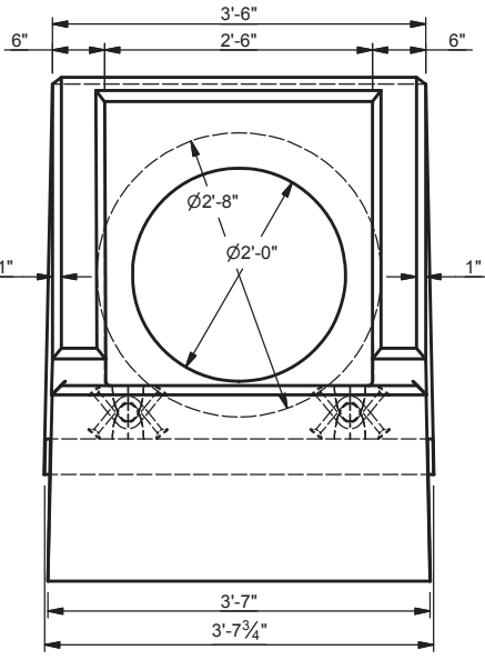
FRONT VIEW SCALE 1/2"=1'-0"
