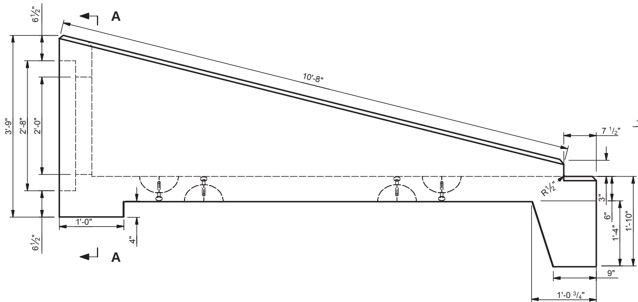
SIDE VIEW SCALE 1/2"=1'-0"
