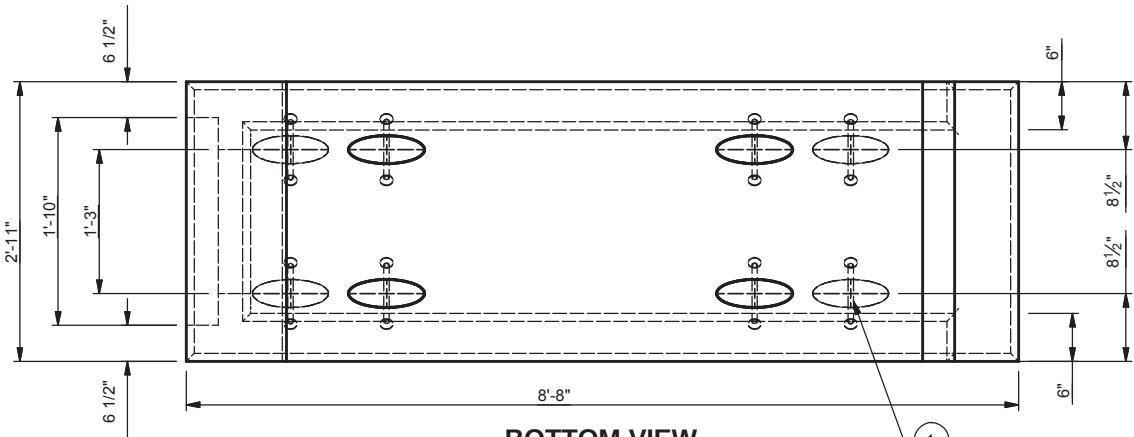
BOTTOM VIEW SCALE 1/2"=1'-0"
