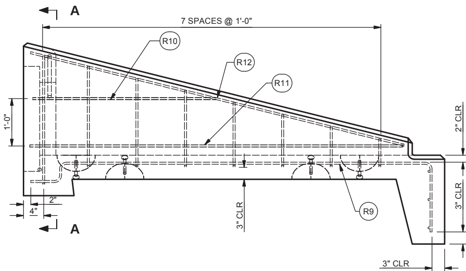
SIDE VIEW SCALE 1/2"=1'-0"
