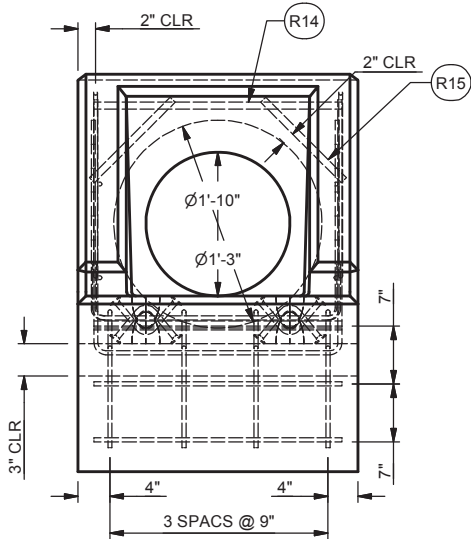
FRONT VIEW SCALE 1/2"=1'-0"
