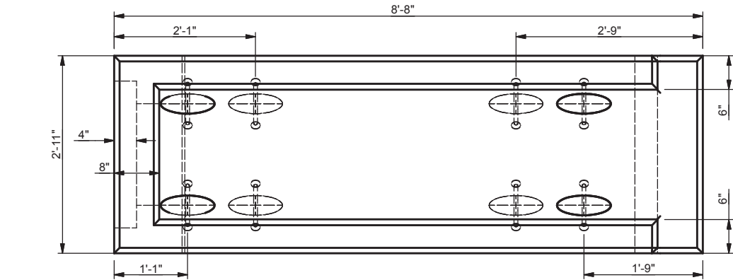
TOP VIEW SCALE 1/2"=1'-0"
