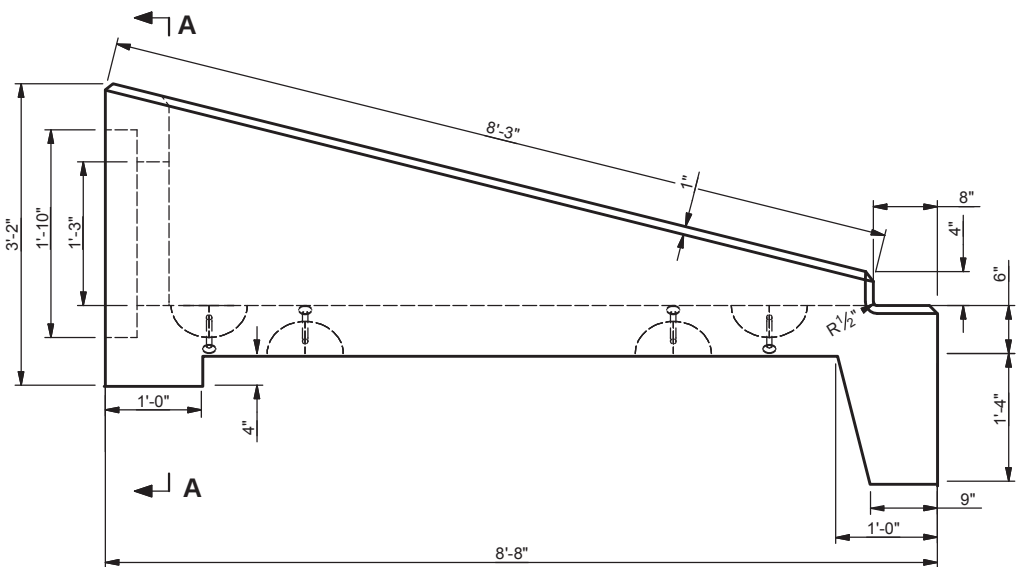
SIDE VIEW SCALE 1/2"=1'-0"
