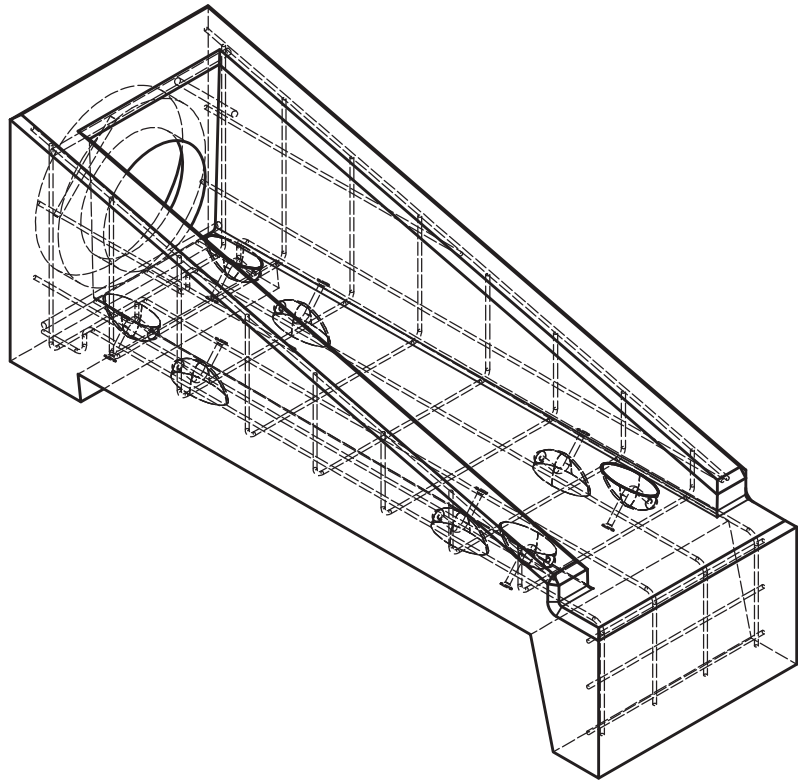
ISOMETRIC VIEW SCALE 1/2"=1'-0"
