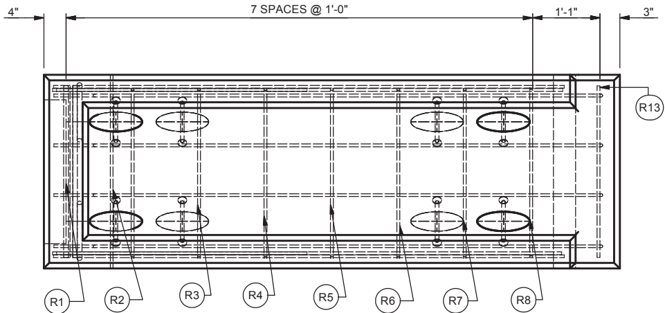
TOP VIEW SCALE 1/2"=1'-0"
