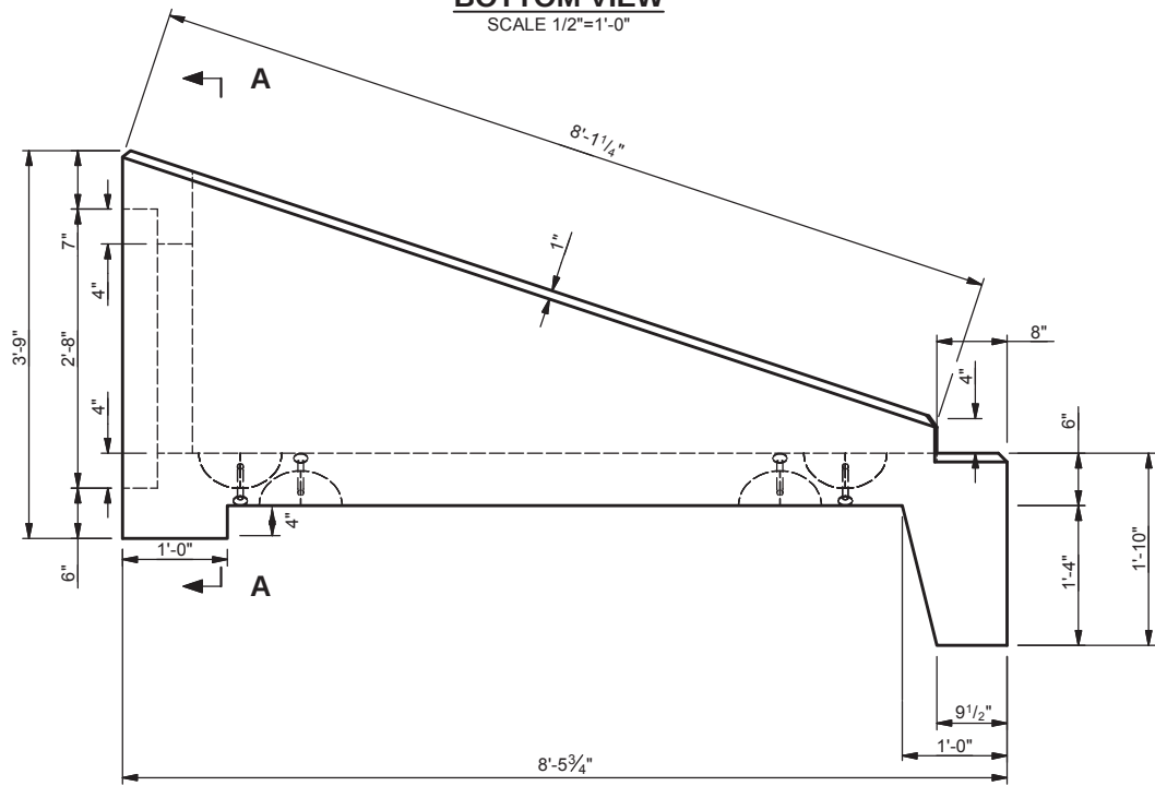
SIDE VIEW SCALE 1/2"=1'-0"
