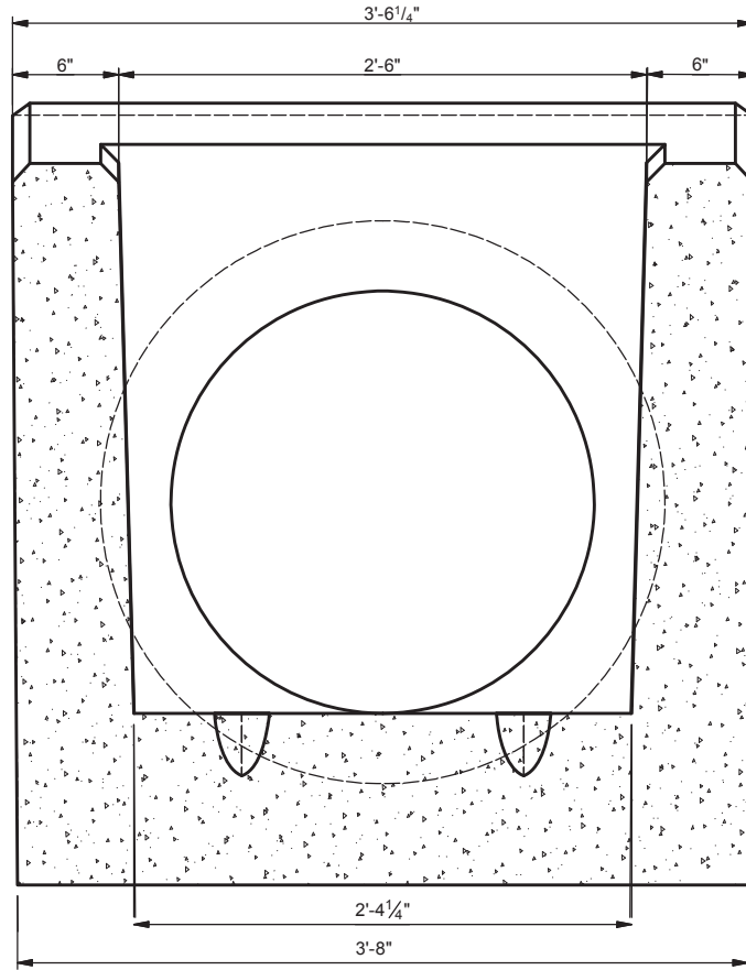
SECTION A-A SCALE 1"=1'
