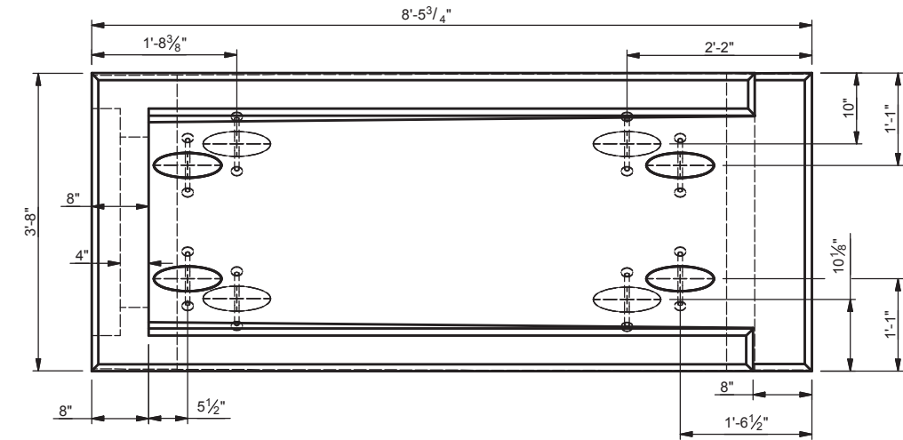
PLAN VIEW SCALE 1/2"=1'-0"
