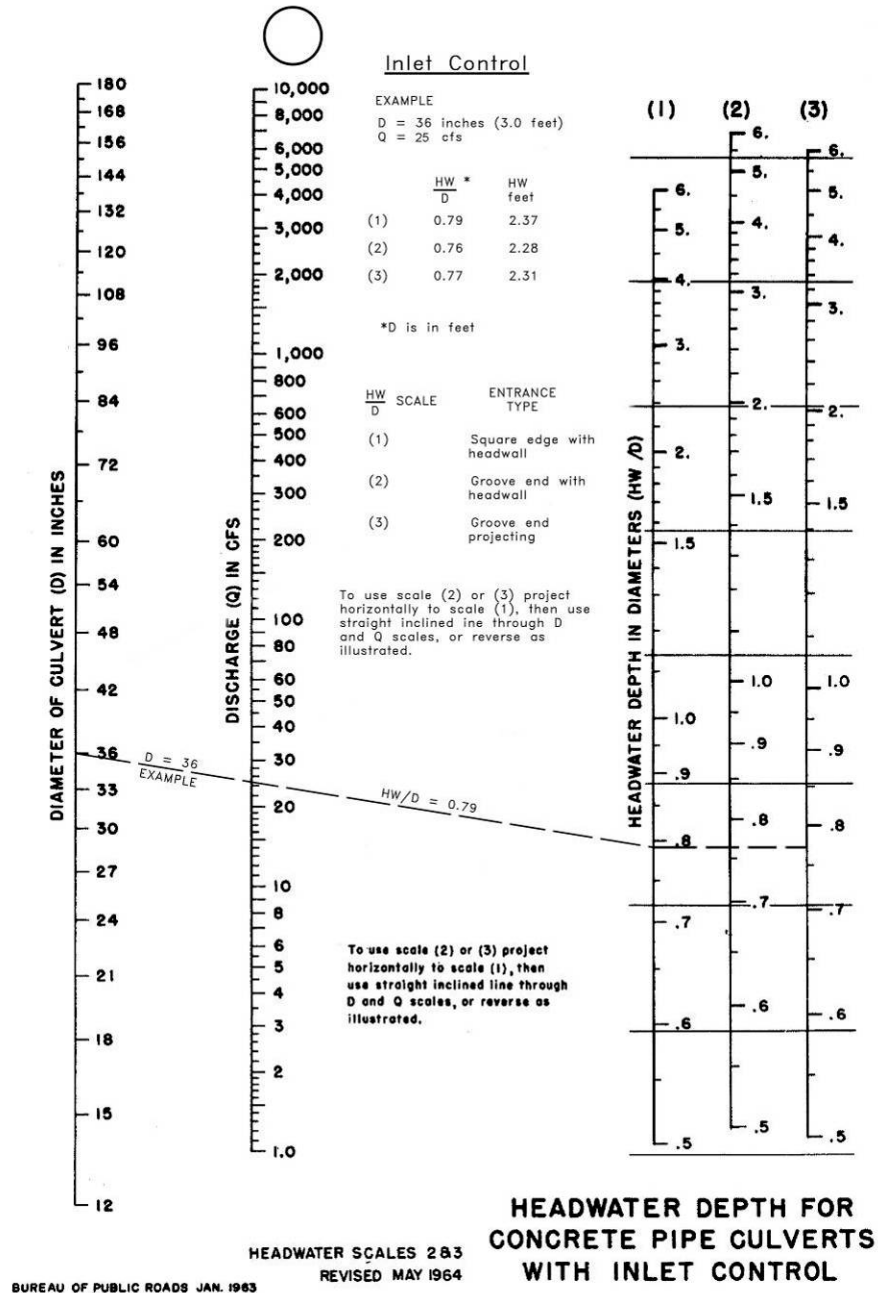
Figure 6A-13 Completed Inlet Control Headwater Chart (Problem #1) Reference: USDOT, FHWA, HDS-5 (1985)
