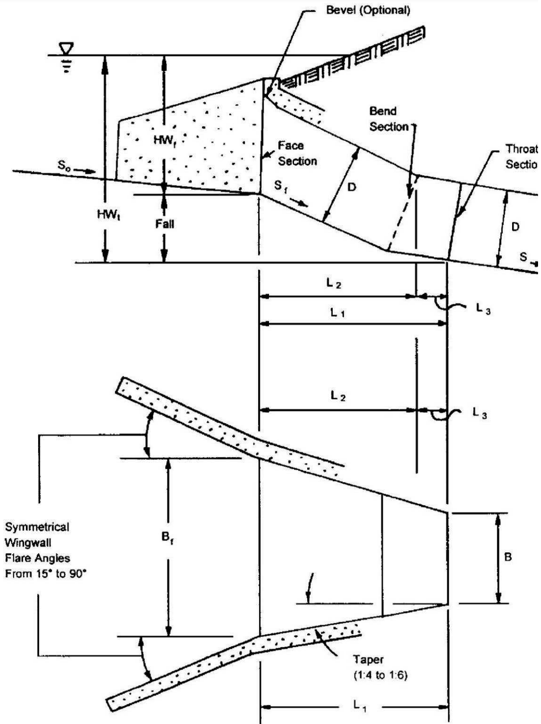
Figure 6A-4 Slope Tapered Inlet with Vertical Face Reference: USDOT, FHWA, HDS-5 (1985)
