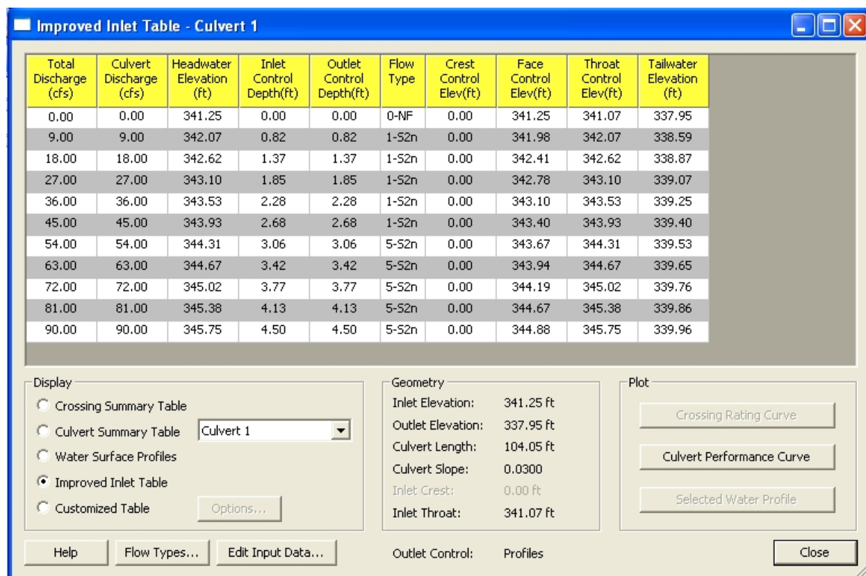
Figure 6A-26 HY-8 Side-Tapered Inlet Performance Curve Screen
