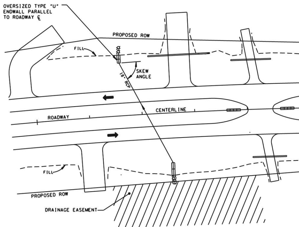
Figure 6-9 Skewed Culvert with Endwall Parallel to Roadway Centerline
