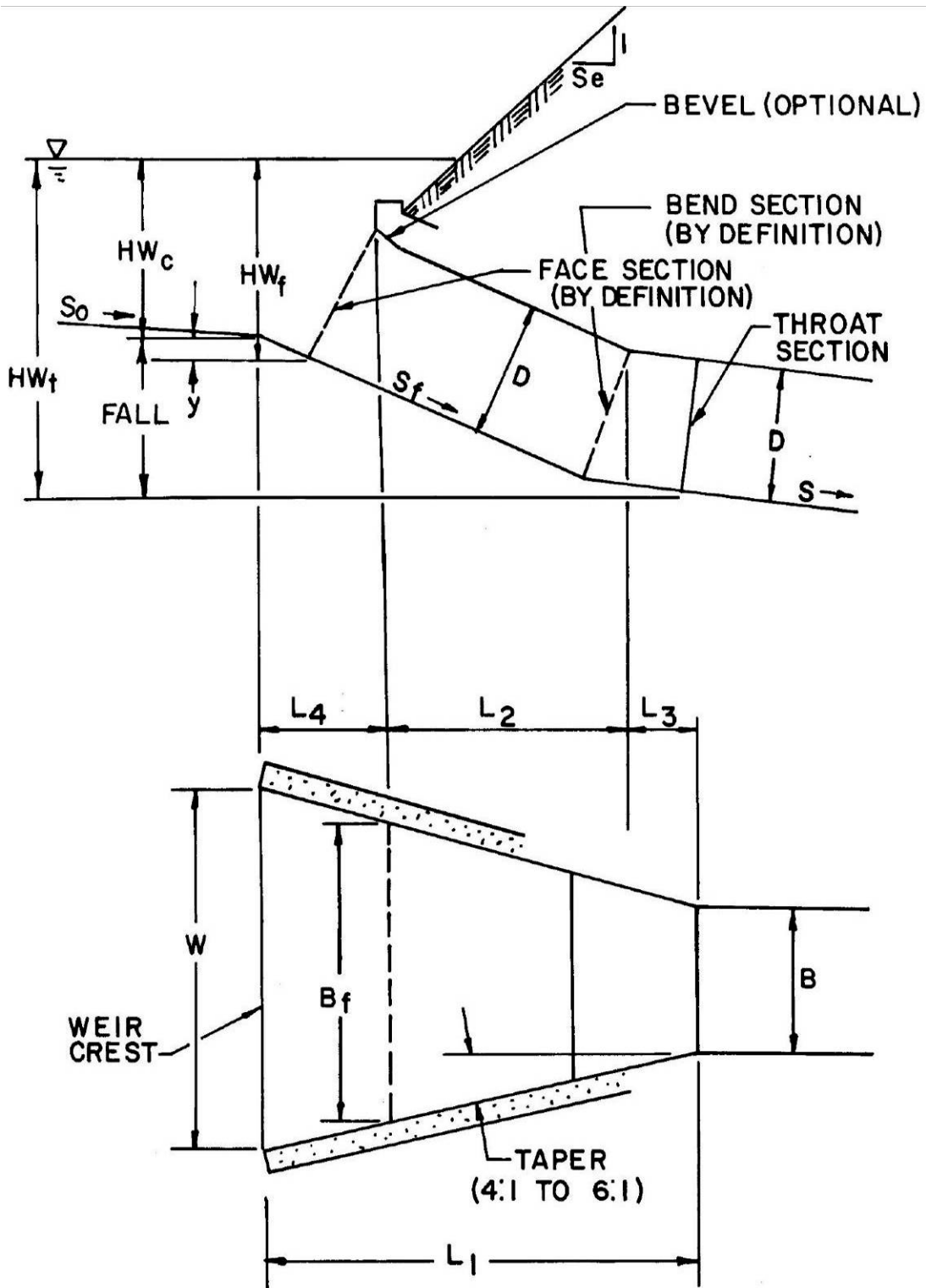
Figure 6A-5 Slope Inlet with Mitered Face Reference: USDOT, FHWA, HDS-5 (1985)
