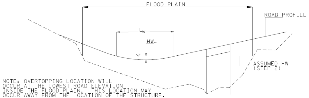
Figure 6-11 Coefficients for Roadway Overtopping
