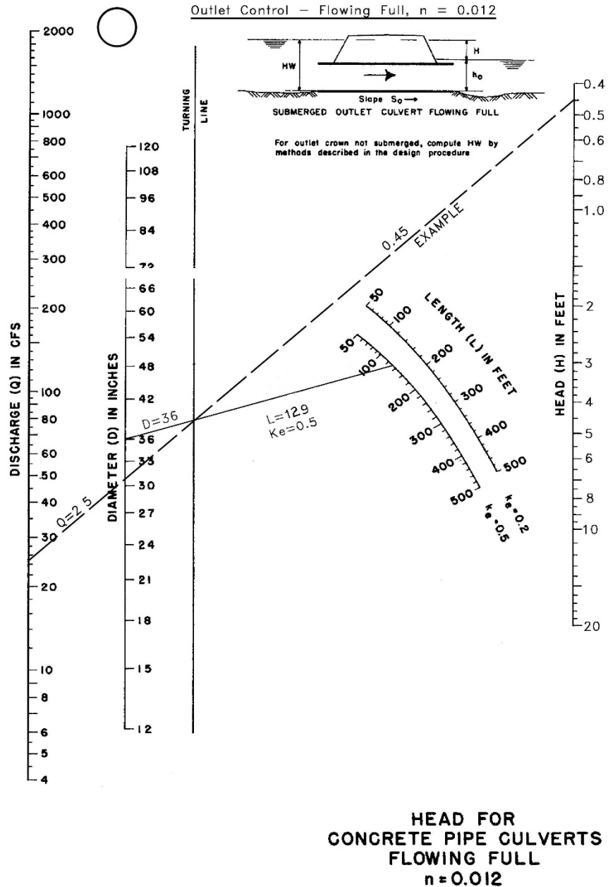
Figure 6A-14 Completed Outlet Control Headwater Chart ( Problem #1) Reference: USDOT, FHWA, HDS-5 (1985)
