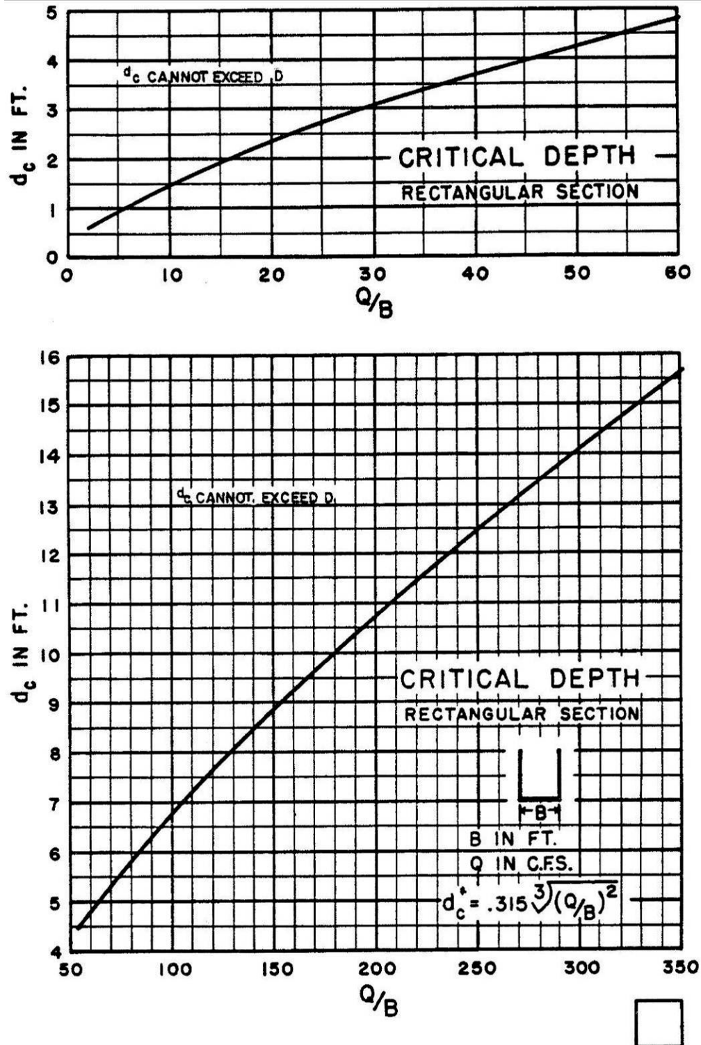
Figure 6A-6 Critical Depth Chart for Rectangular Sections Reference: USDOT, FHWA, HDS-5 (1985)
