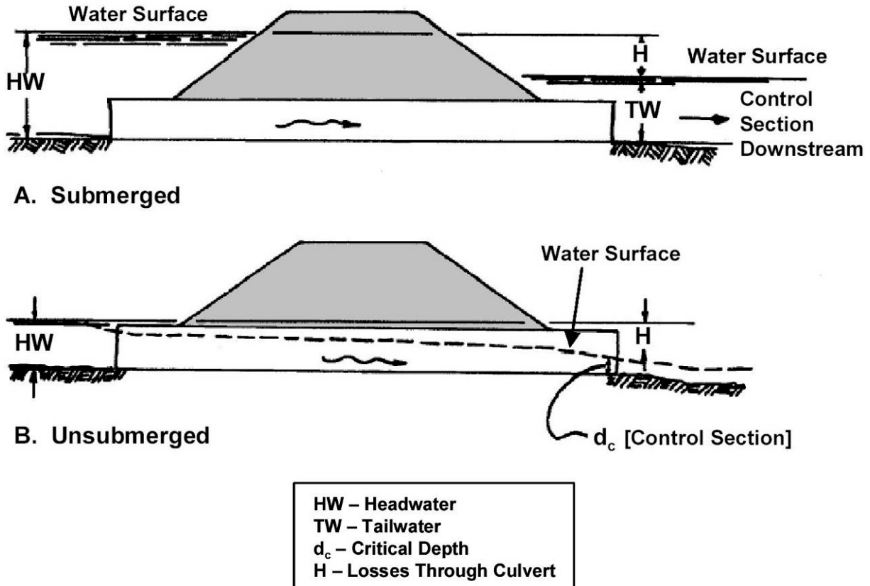
Figure 6-8 Outlet Control Flow Conditions
