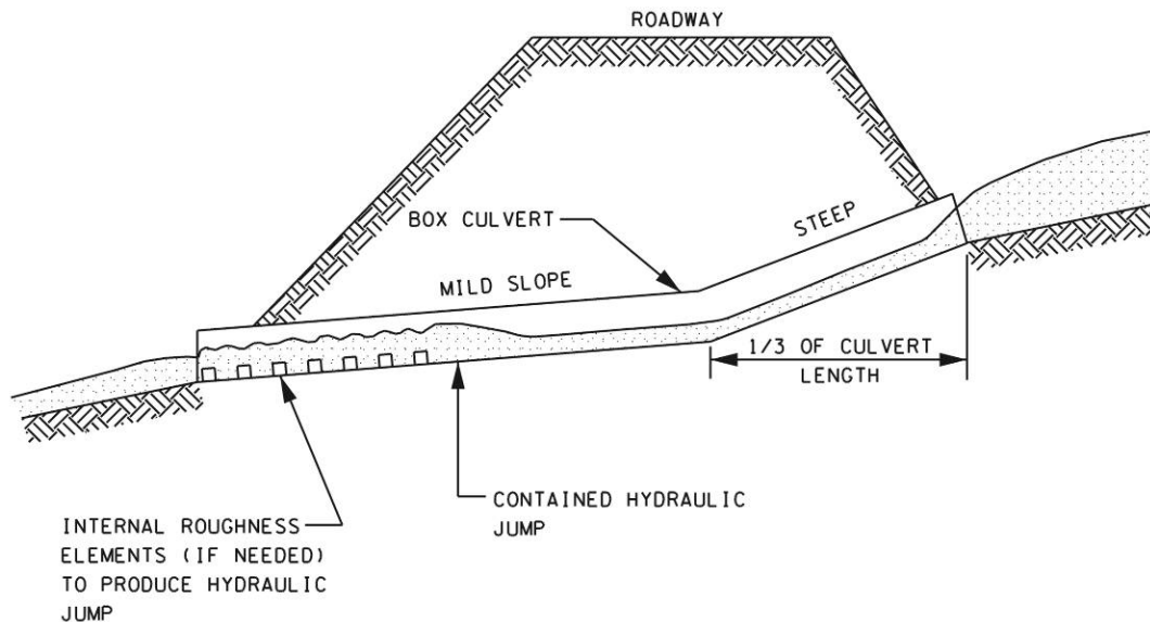
Figure 6-4 Broken-Back Culvert for Velocity Control
