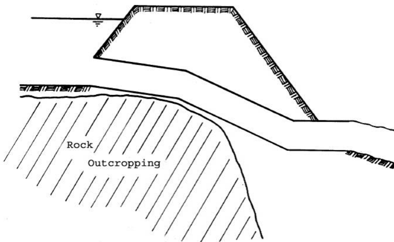
Figure 6-2 Broken Back Culvert Reference: USDOT, FHWA, HDS-5, (1985)
