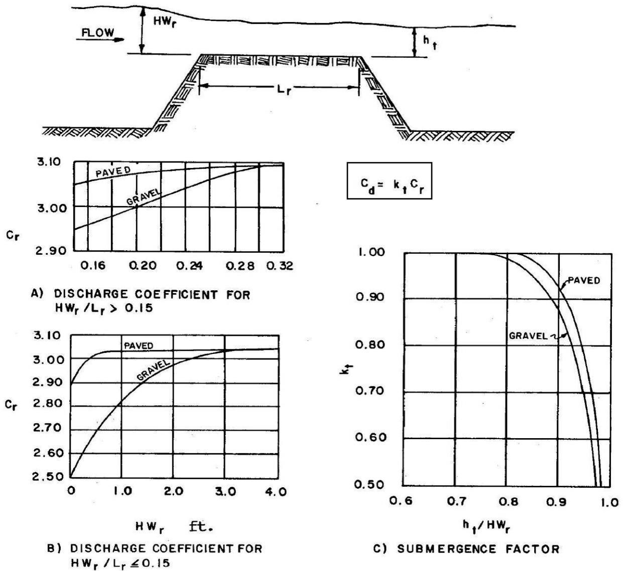
Figure 6A-3 Discharge Coefficients for Roadway Overtopping Reference: USDOT, FHWA, HDS-5 (1985)
