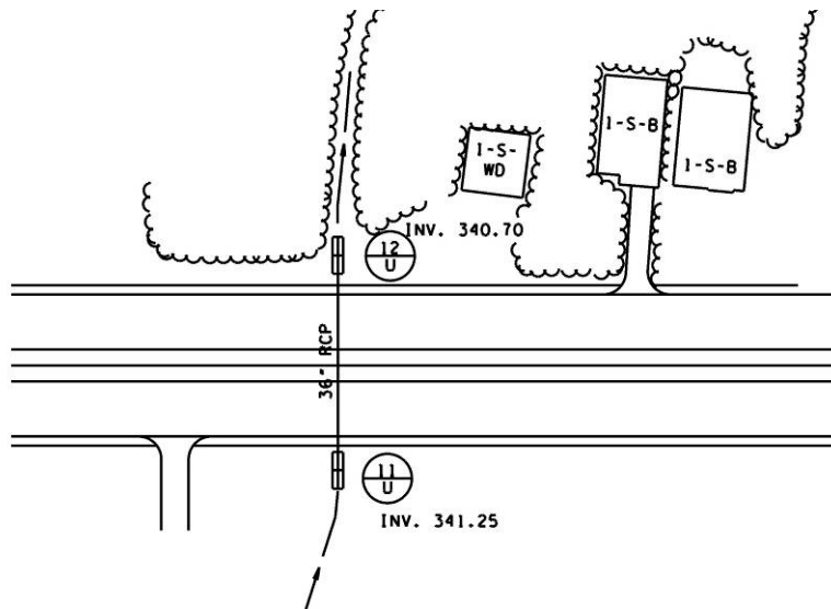
Figure 6A-11 Culvert Roadway Crossing
