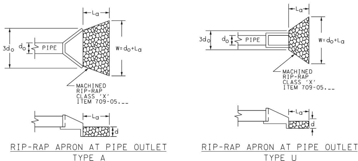
Figure 6-12 Definition Sketch for Riprap Apron Dimensions
