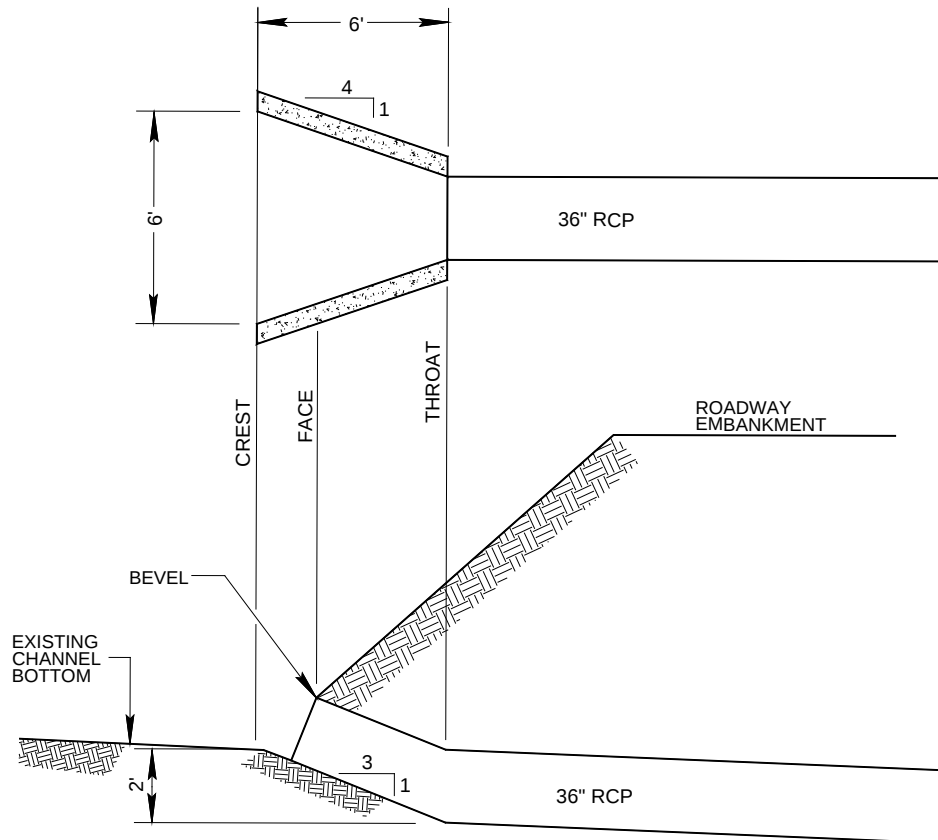
Figure 6A-27 Slope Tapered Improved Inlet Plan & Section
