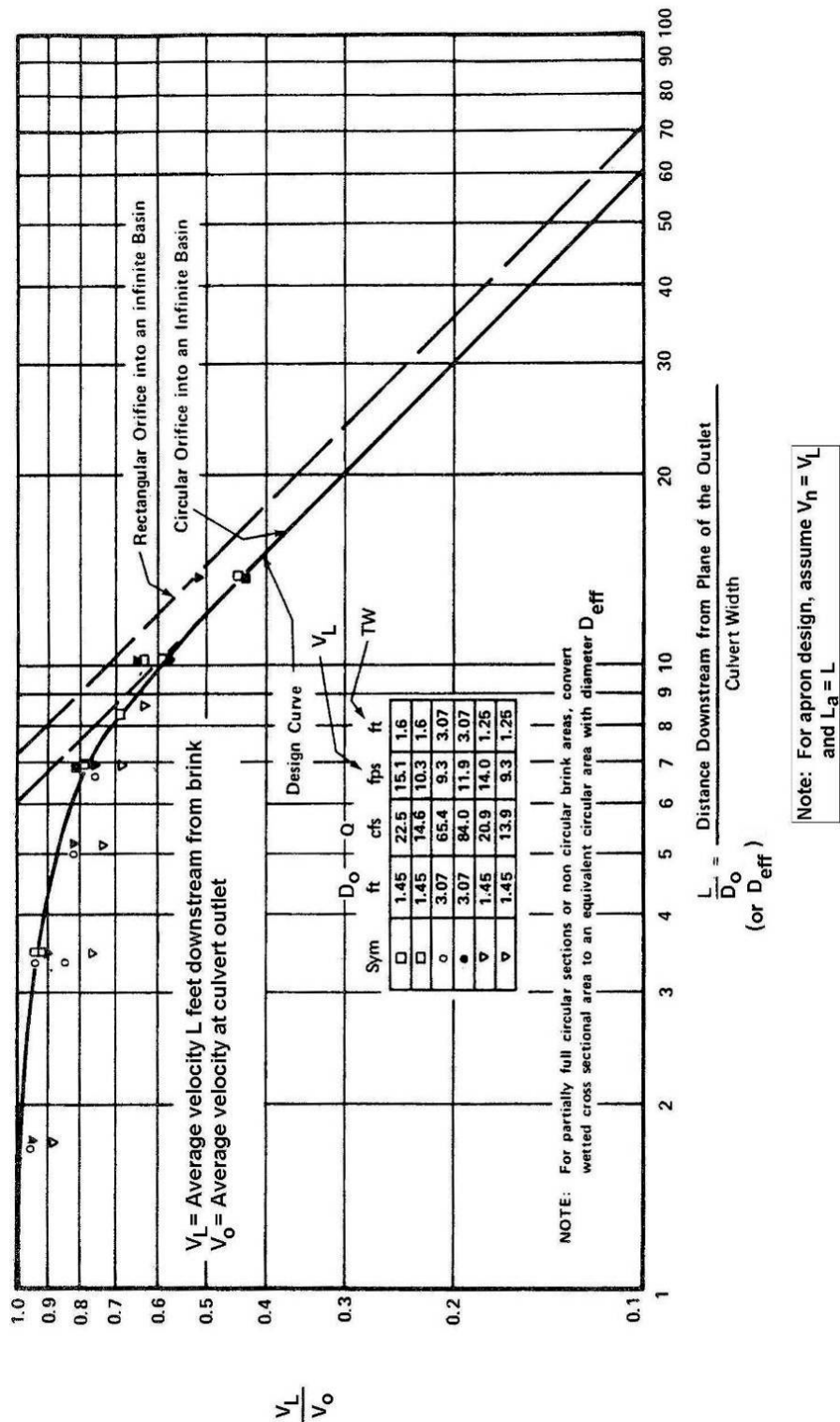
Figure 6A-10 Distribution of Centerline Velocity for Flow from Submerged Outlets
