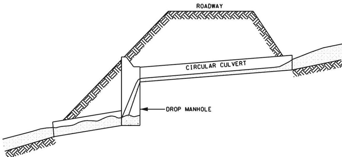
Figure 6-3 Drop Structure for Velocity Control
