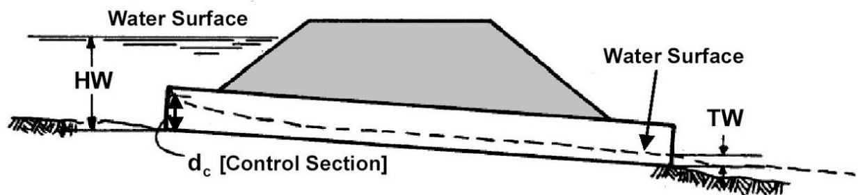
Figure 6-7 Inlet Control Flow Conditions
