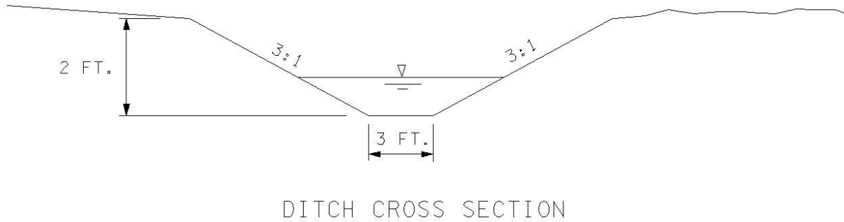
Figure 4A-7 Ditch Cross Section for Simple Drainage Area Example
