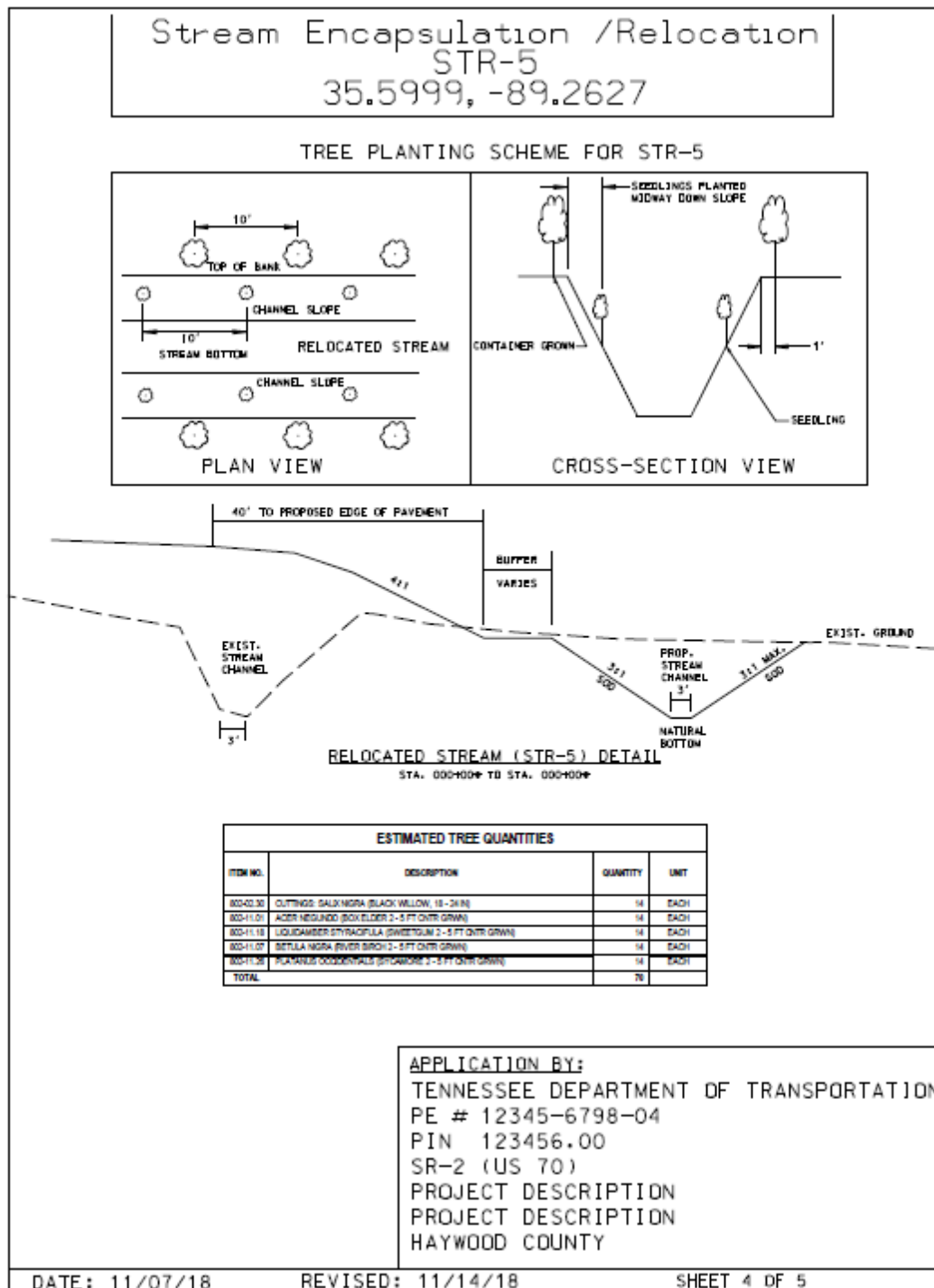
Figure 0.9 - Example Permit Sketches: Stream Relocation with Structures (continued)
