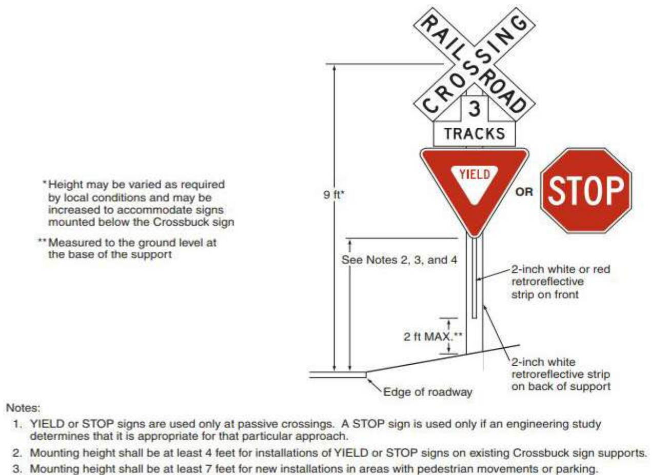
Figure 11. Highway-Rail Crossing (Crossbuck) Sign and STOP or YIELD Sign on Same Post
