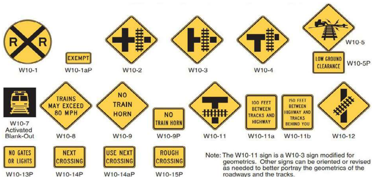
Figure 8. Warning Signs and Plaques for Crossings
