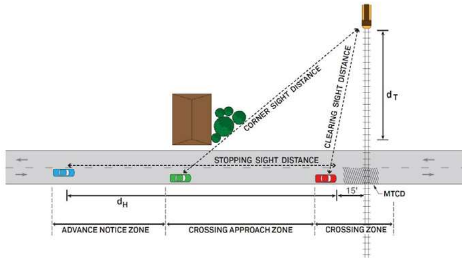
Figure 5. Approach Regions with Passive Traffic Control Devices
