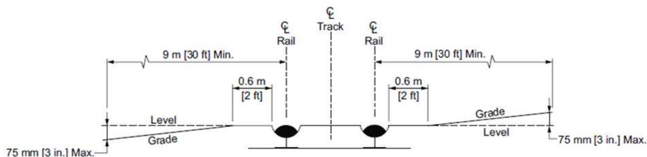
Figure 1. Highway-Rail Crossing Cross Section
