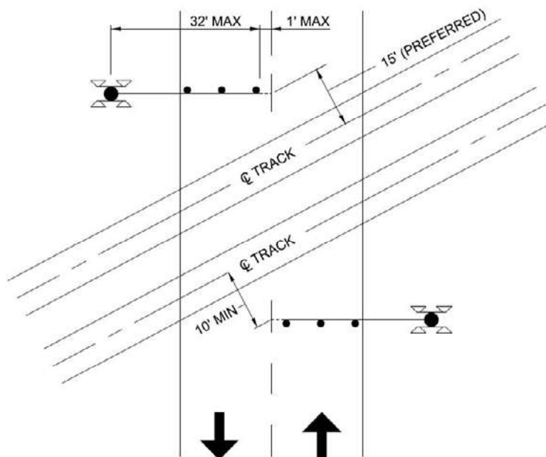
Figure 29. Typical Crossing Gate Placement at Obtuse Angled Crossing
