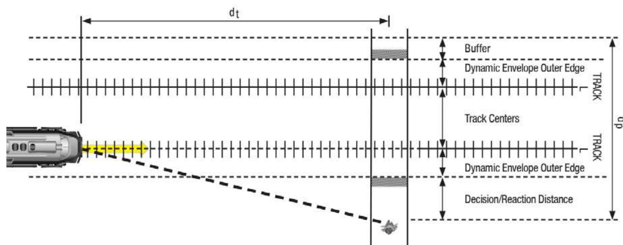
Figure C-6. Pedestrian Sight Distance Triangle (Double Track Crossing)
