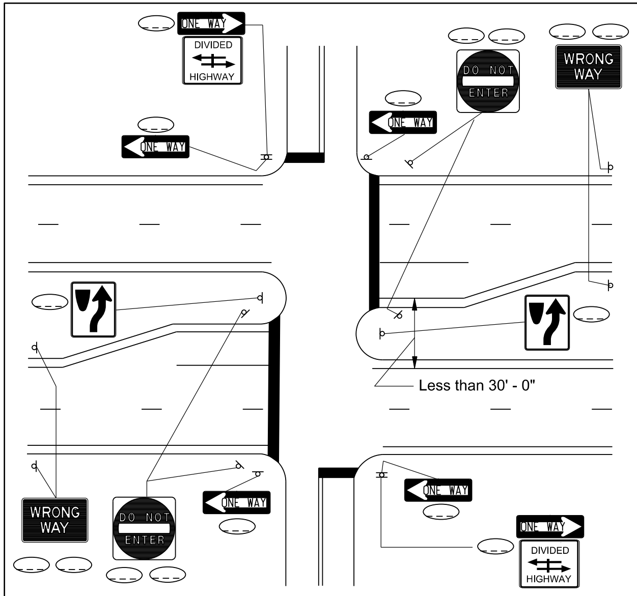
Figure 14.8 – Signalized Intersection, Medians less than 30 feet, One-Way and Wrong-Way Signing
