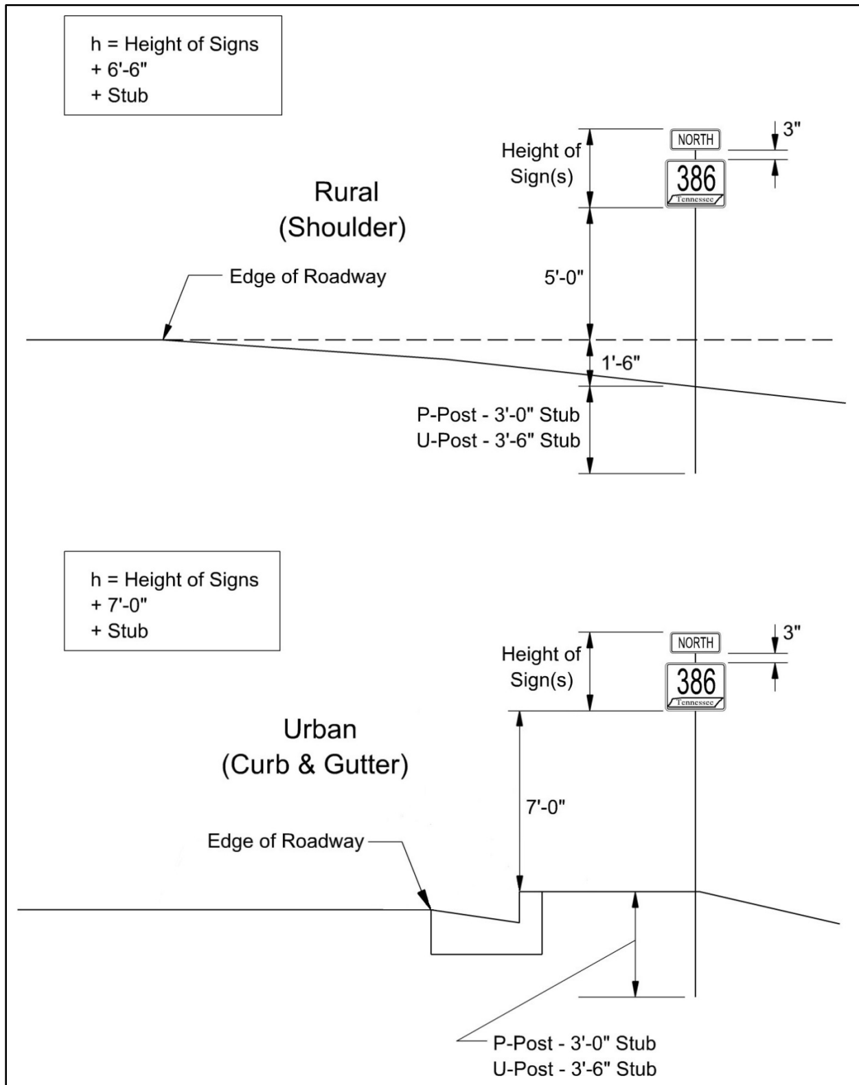
Figure 14.17 – Estimating Length of Support
