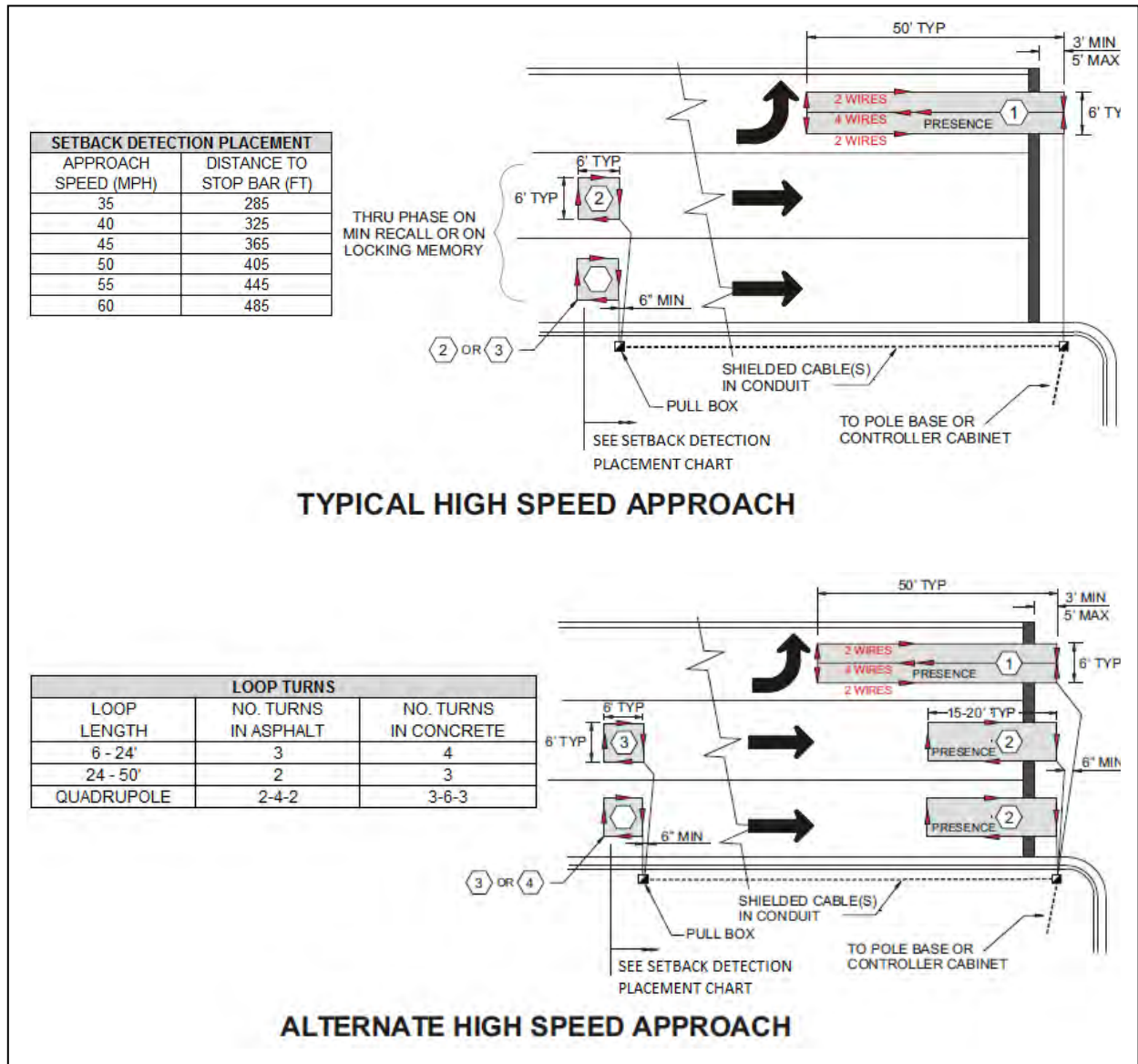
Figure 8.4 – Inductive Loop Detection ( \geq 35 MPH)
