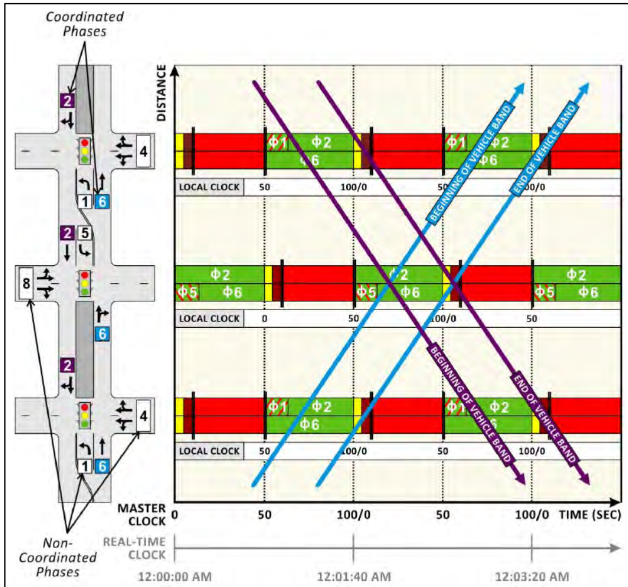
Figure 7.21 – Time-Space Diagram Source: Traffic Signal Timing Manual
