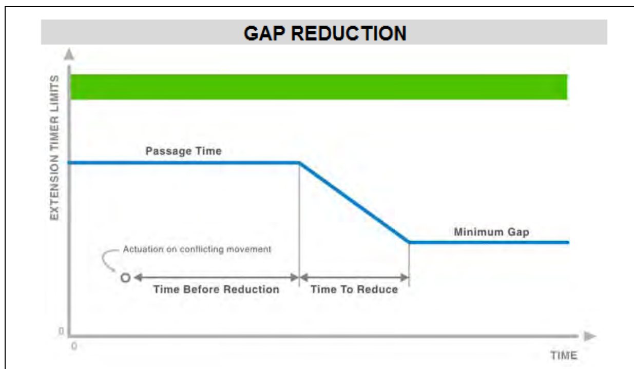
Figure 7.25 – Volume Density (Gap Reduction)
