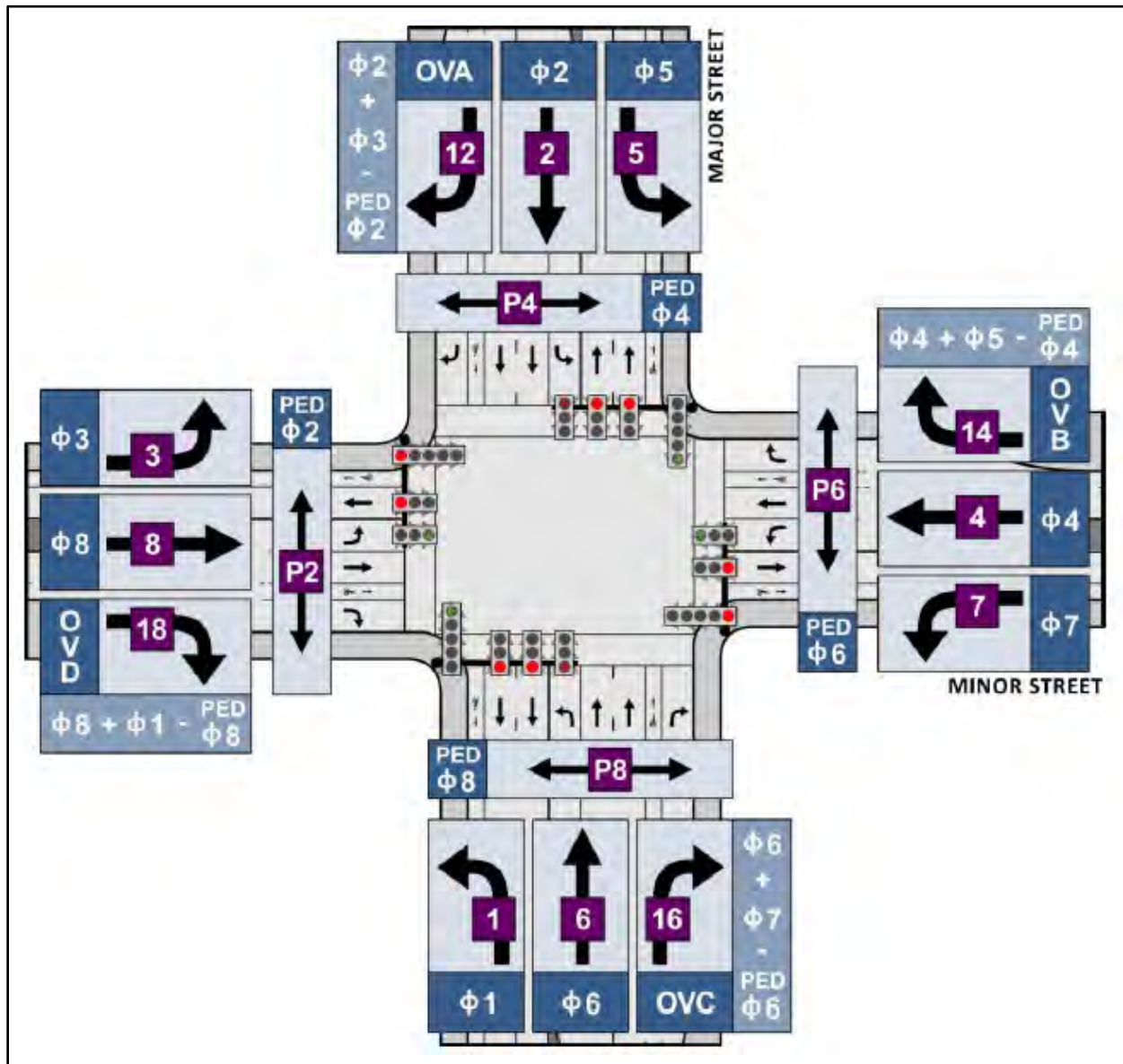
Figure 7.14 – Right-Turn Overlap Phase Lettering Scheme Source: Traffic Signal Timing Manual
