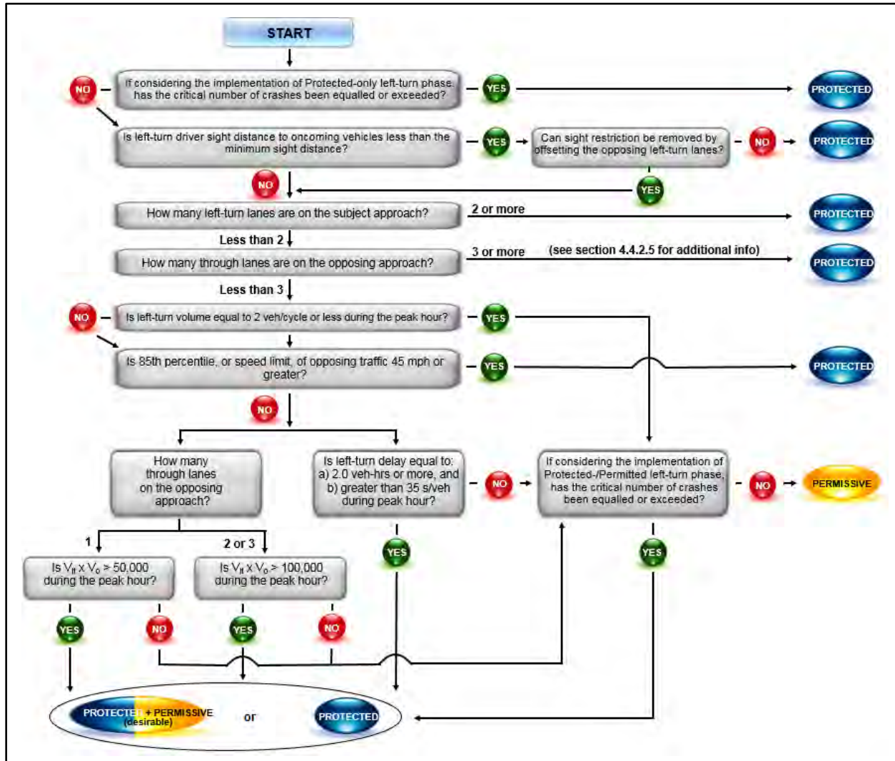
Figure 7.9 – Guidelines for Selecting Left-Turn Phasing Source: Traffic Signal Timing Manual
