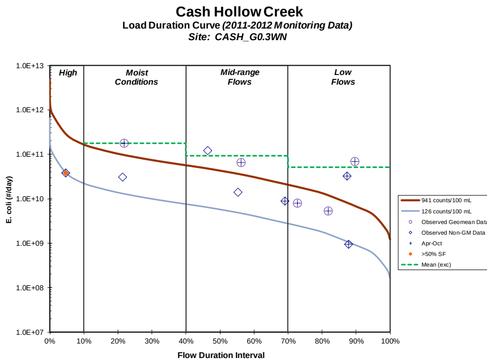
Figure E-13. E. Coli Load Duration Curve for Cash Hollow Creek – RM0.3
