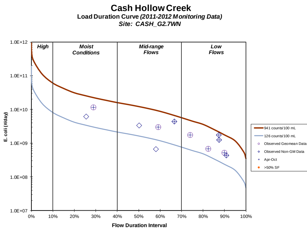
Figure E-14. E. Coli Load Duration Curve for Cash Hollow Creek – RM2.7
