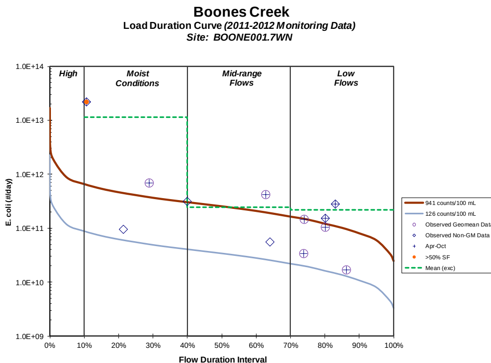
Figure E-6. E. Coli Load Duration Curve for Boones Creek – RM1.7
