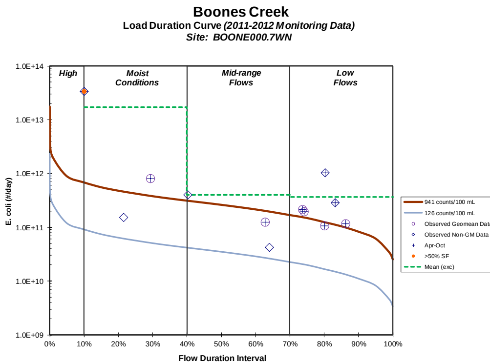
Figure E-5. E. Coli Load Duration Curve for Boones Creek – RM0.7
