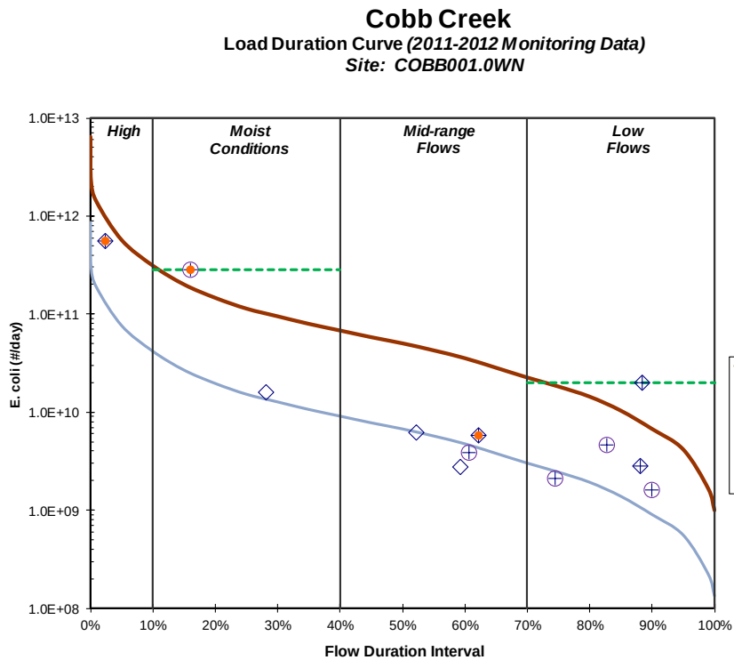
Figure E-16. E. Coli Load Duration Curve for Cobb Creek – RM1.0
