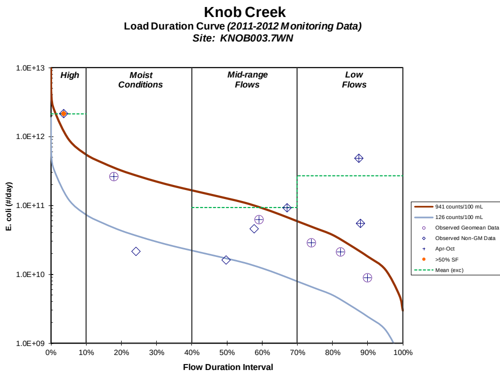
Figure E-21. E. Coli Load Duration Curve for Knob Creek – RM3.7
