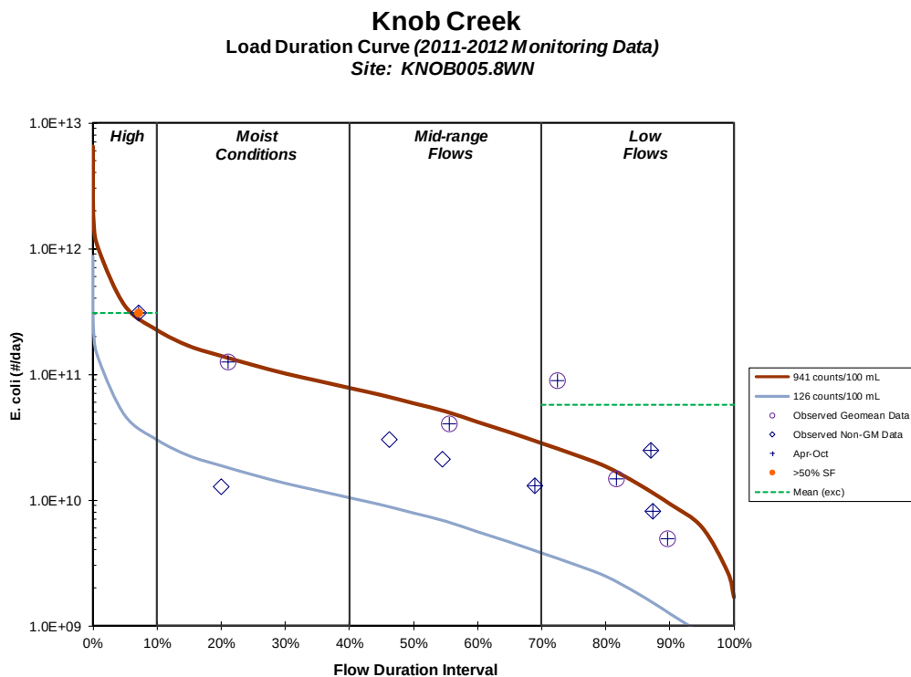
Figure E-22. E. Coli Load Duration Curve for Knob Creek – RM5.8
