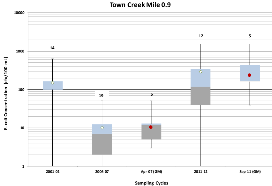
Figure F-4. Box and Whisker Plot for Town Creek – RM0.9
