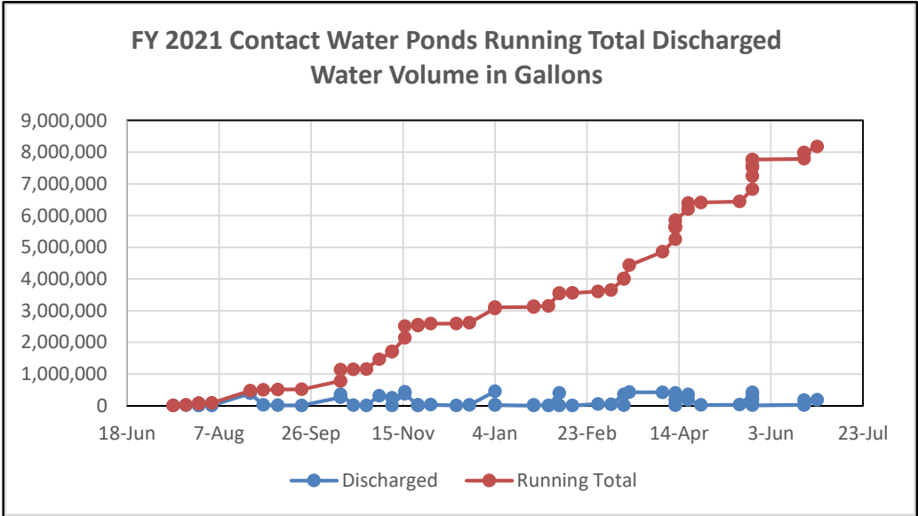
Figure 5.2.19: Contact Water Ponds Running Total of Discharged Water Volume in Gallons
