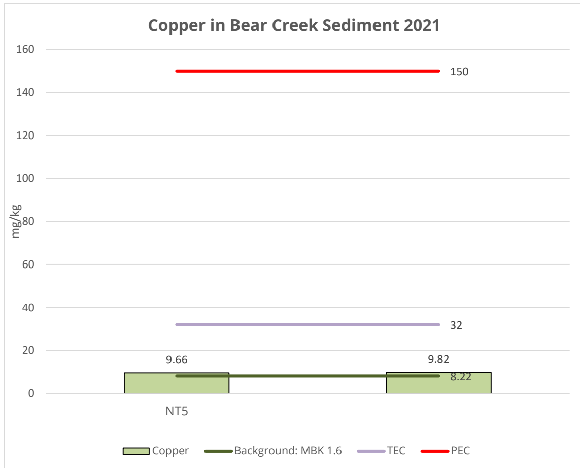
Figure 10.1.6: Sediment Copper
