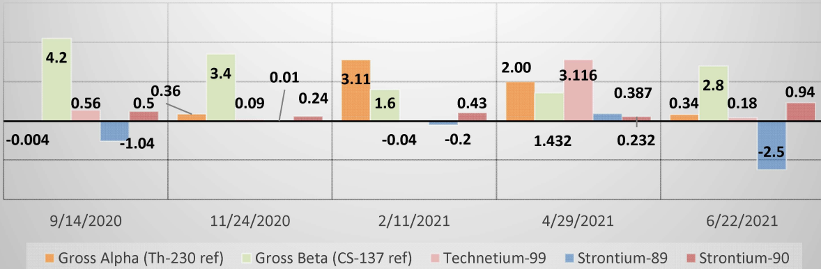
Figure 5.2.10: EMWFM-2 FY2021 Selected Radionuclides Results in pCi/L
