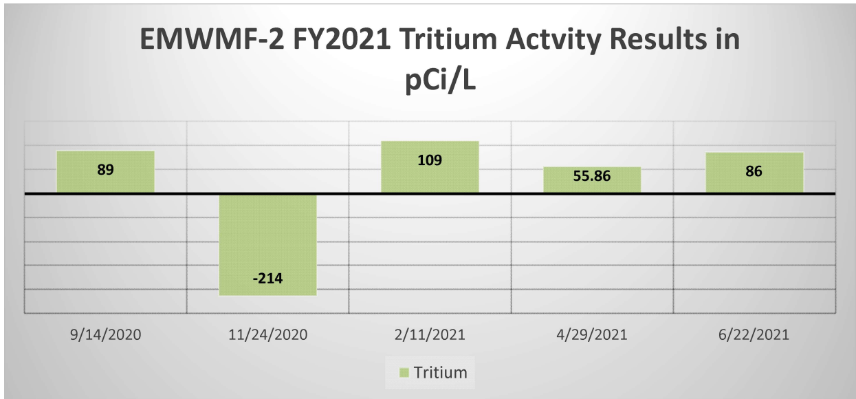
Figure 5.2.14: EMWWMF-2 FY2021 Tritium Activity Results in pCi/L
