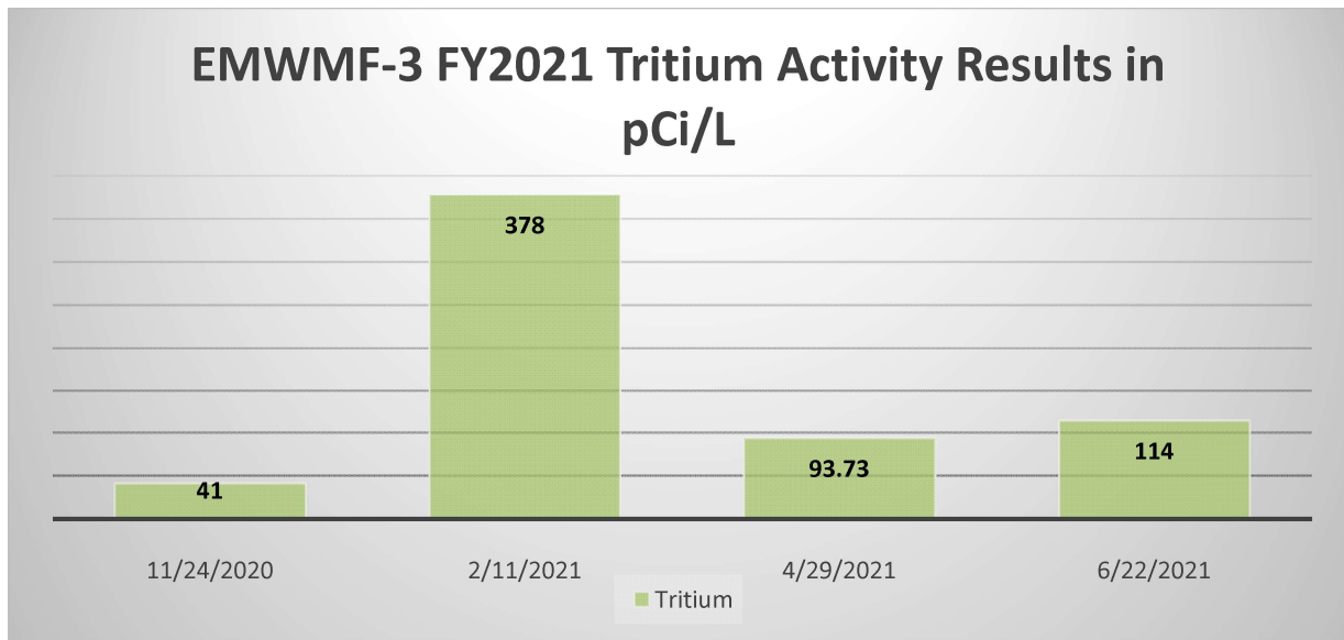
Figure 5.2.15: EMWWMF-3 FY2021 Tritium Activity Results in pCi/L
