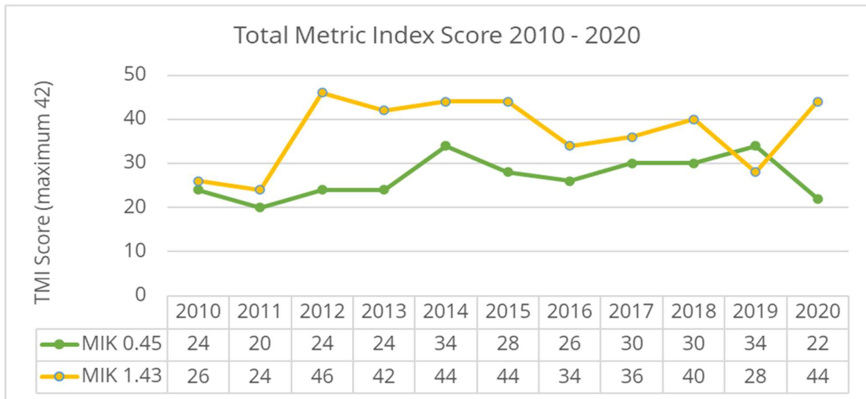
Figure 3.1.7: Total Metric Index Scores in Mitchell Branch from 2010 - 2020
