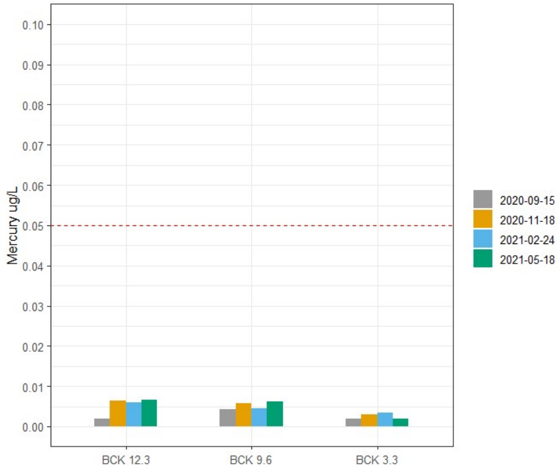
Figure 9.2.12: Mercury concentrations for each sampling event at each station on Bear Creek. The dashed red line indicates the TN criterion of 0.05 \mu\text{g/L} for water and organisms.
