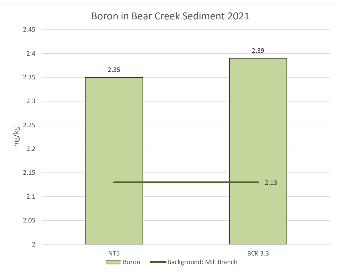
Figure 10.1.3: Sediment Boron
