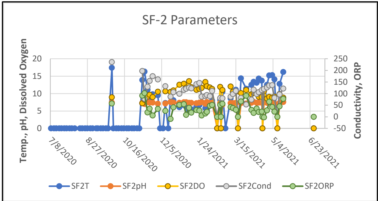
Figure 5.1.3: SF-2 Water Quality Parameters
