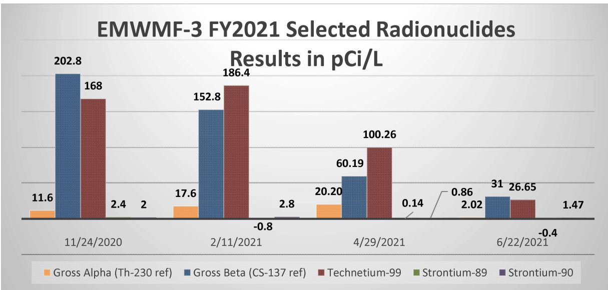
Figure 5.2.11: EMWFM-3 FY2021 Selected Radionuclides Results in pCi/L
