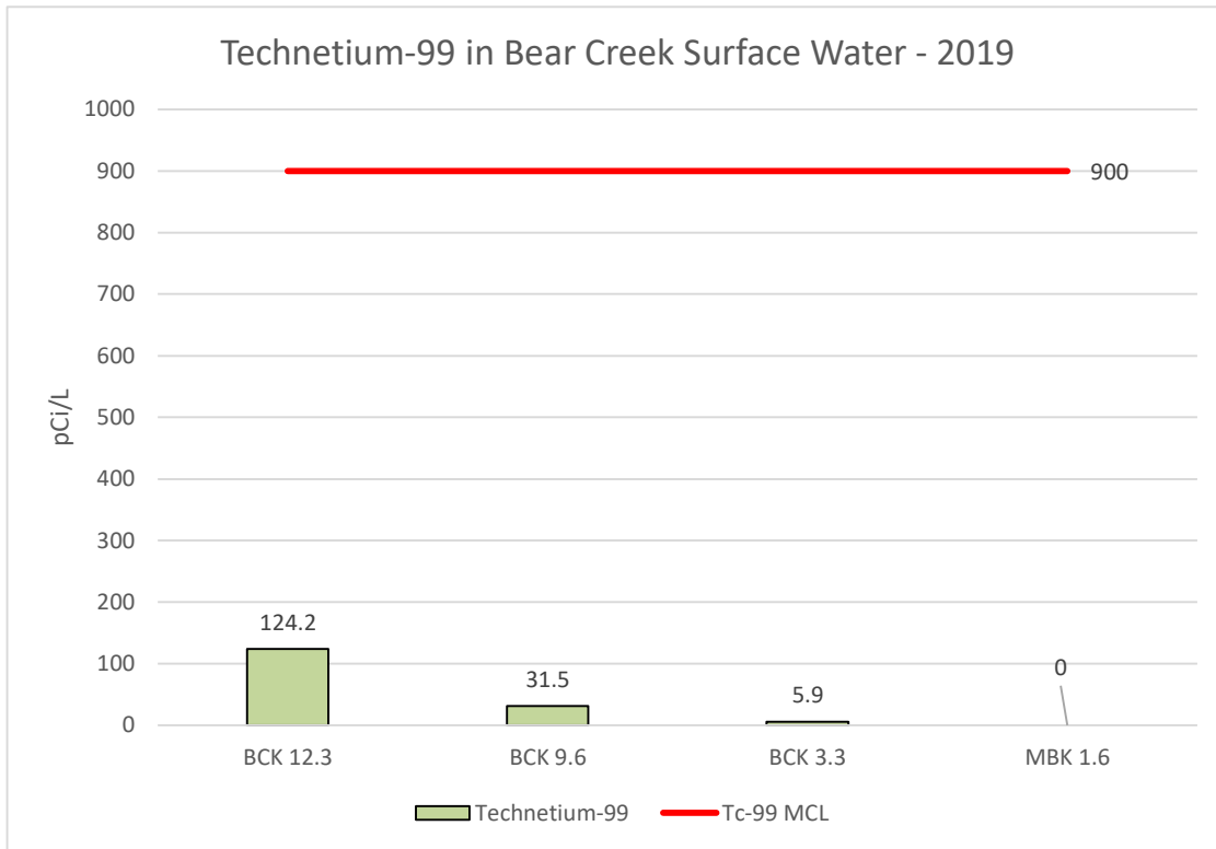
Figure 10.1.20: Technetium-99
