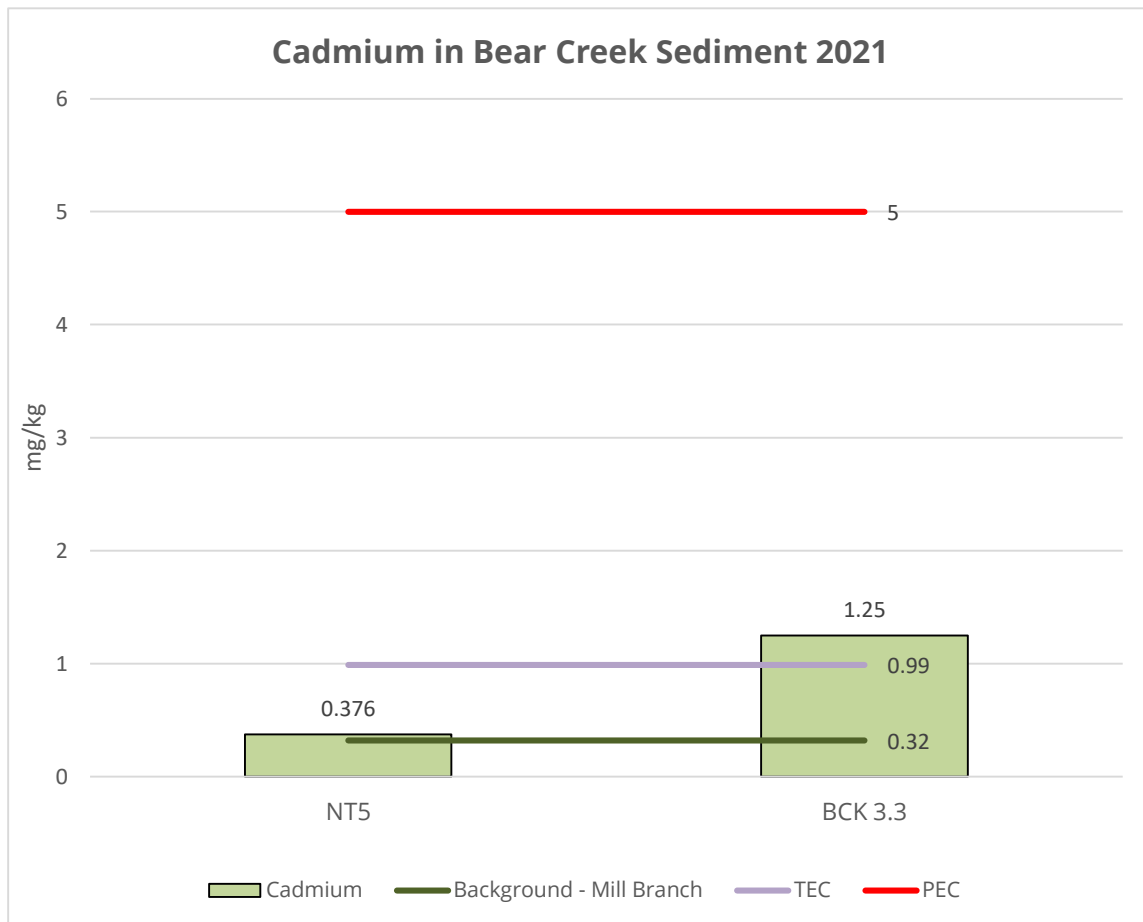
Figure 10.1.4: Sediment Cadmium
