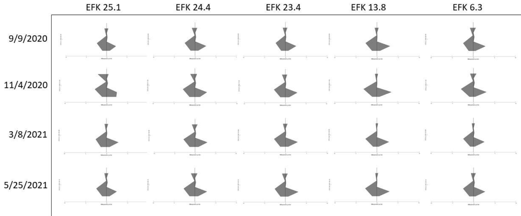
Figure 9.2.5: East Fork Poplar Creek stiff plots in milliequivalents per liter for four sampling events. Nodes on left side of stiff plot axis from top to bottom include sodium, potassium, calcium, and magnesium. Nodes on the right side of axis from top to bottom include chloride, fluoride, nitrates, phosphate, carbonate/bicarbonate, and sulfate. A predominant calcium bicarbonate water is shown at all sampling events with a fair amount of magnesium. A small amount of sodium, chloride, and sulfate are also present.
