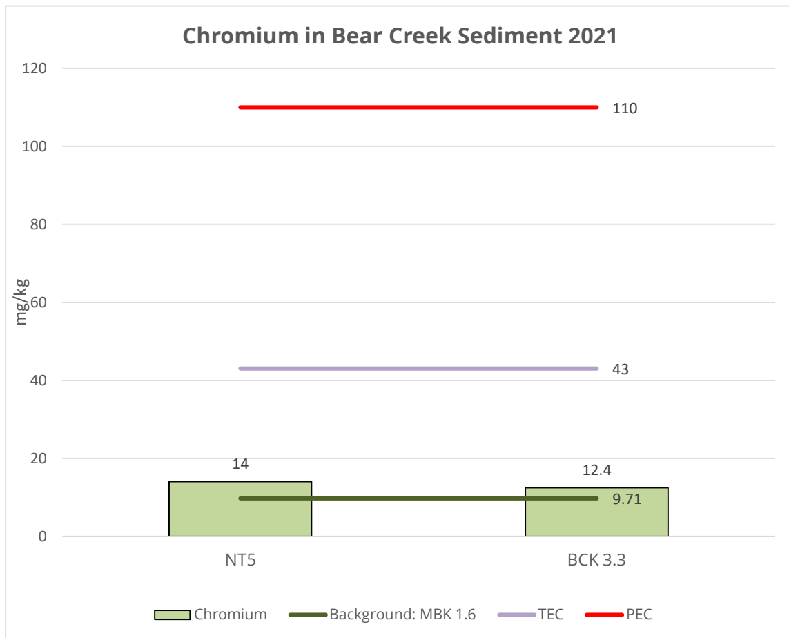
Figure 10.1.5: Sediment Chromium
