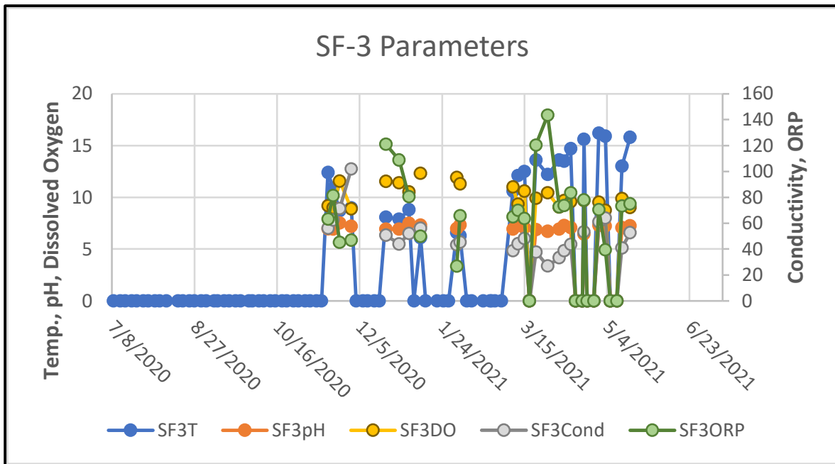
Figure 5.1.4: SF-3 Water Quality Parameters
