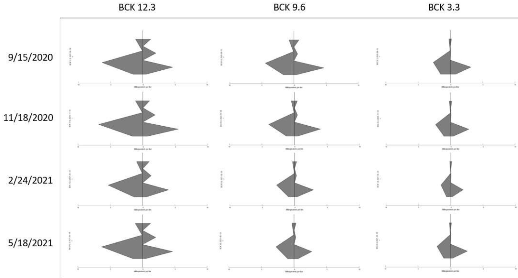
Figure 9.2.7: Bear Creek stiff plots in milliequivalents per liter for four sampling events. Nodes on left side of stiff plot axis from top to bottom include sodium, potassium, calcium, and magnesium. Nodes on the right side of axis from top to bottom include chloride, fluoride, nitrates, phosphate, carbonate/bicarbonate, and sulfate. A predominant calcium bicarbonate water is shown at all sampling events with a fair amount of nitrates. A small amount of sodium, chloride, and sulfate are also present. Dilution occurs from BCK 12.3 to downstream sites for all cations and anions.
