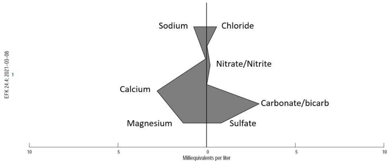
Figure 9.2.4: Typical East Fork Poplar Creek stiff plot. This plot shows EFK 24.4 on 3/8/2021 in milliequivalents per liter. Note the predominately calcium carbonate water signature.
