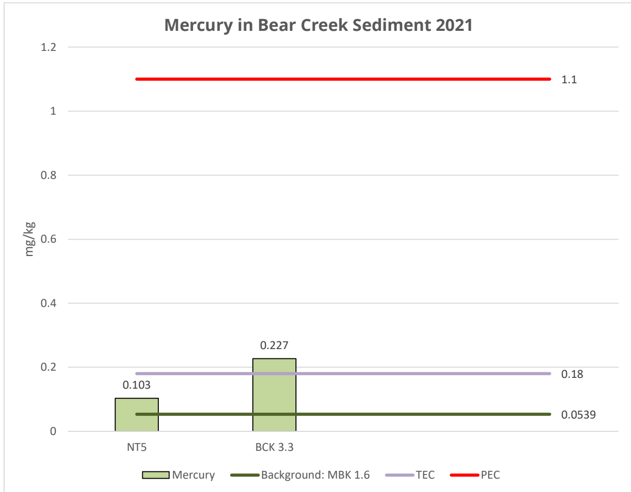
Figure 10.1.8: Sediment Mercury
