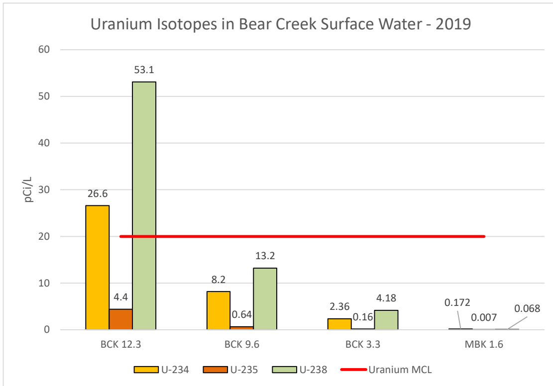
Figure 10.1.19: Uranium isotopes
