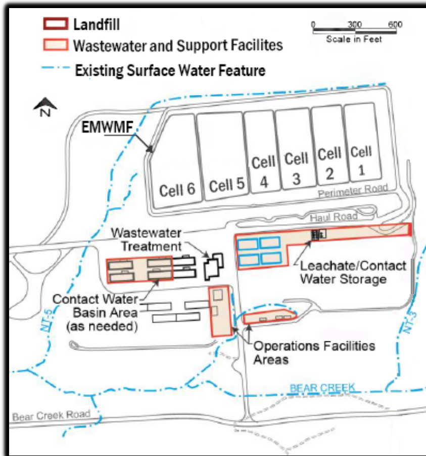
Figure 5.2.1.1 EMWMF Diagram
