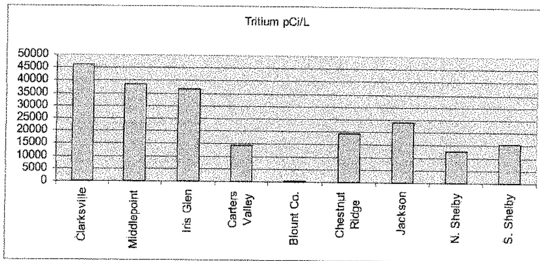
Figure 2. Tritium concentrations in leachate from nine Tennessee landfills.
