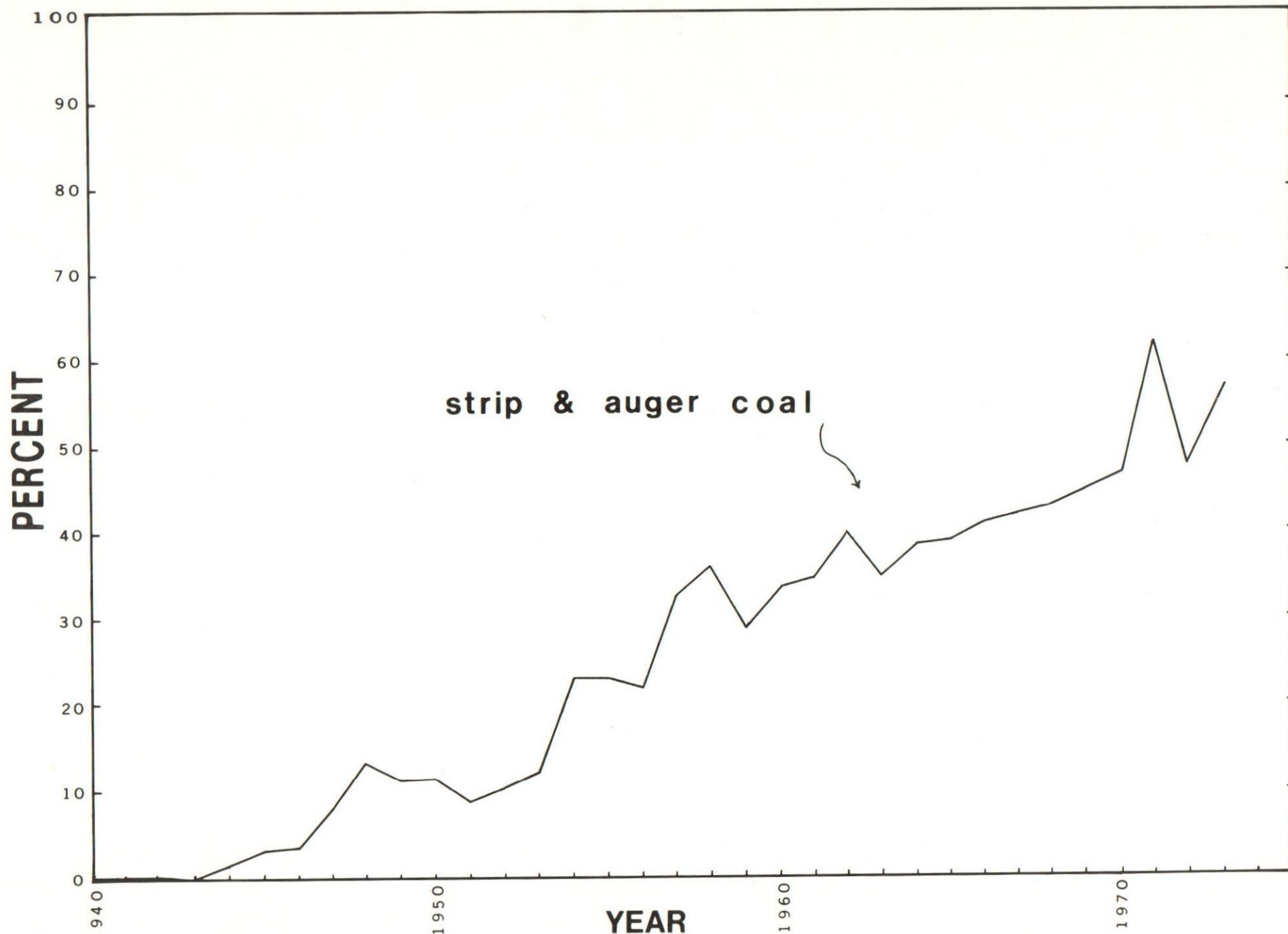
Figure 4. Coal production from strip and auger mines as a percentage of Tennessee's total production, 1940-1973.
