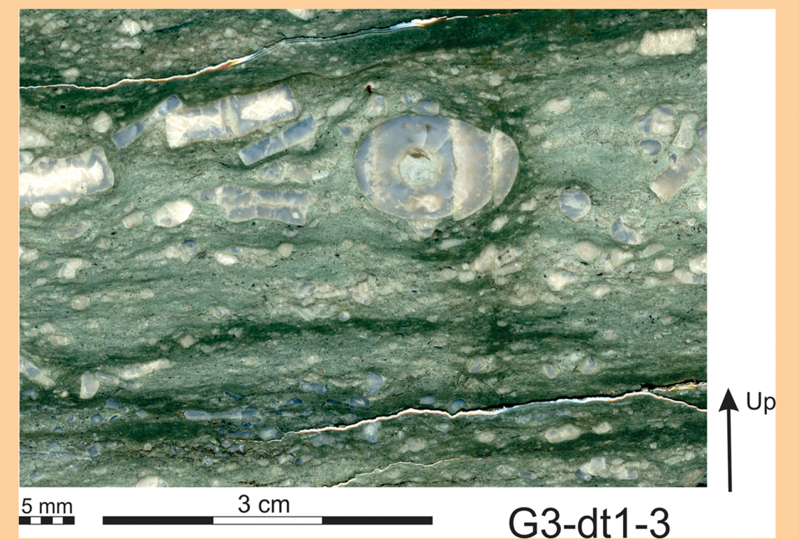
Siliciclastic Mudstone with dispersed crinoid grains Facies
