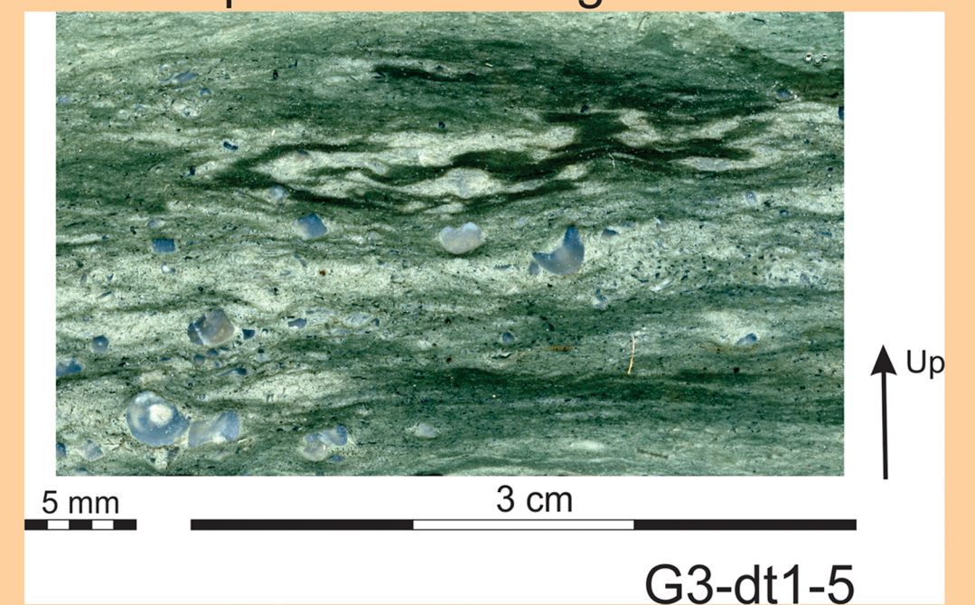
Siliciclastic Mudstone with dispersed crinoid grains Facies
