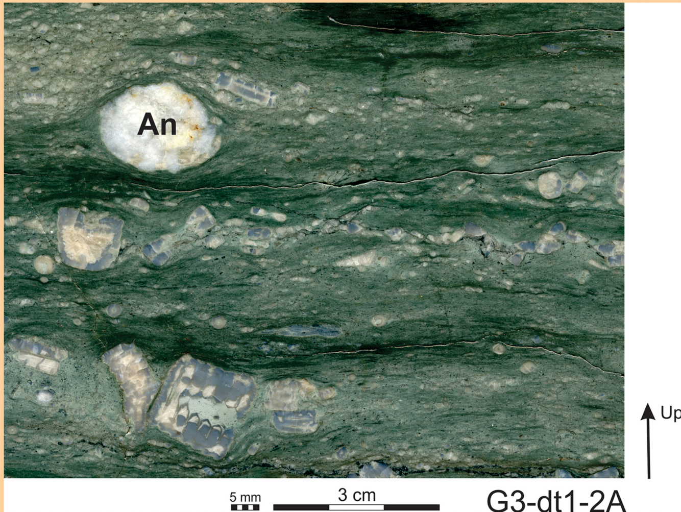
An: anhydrite nodule "Layered" Siliciclastic Mudstone with dispersed crinoid grains Facies
