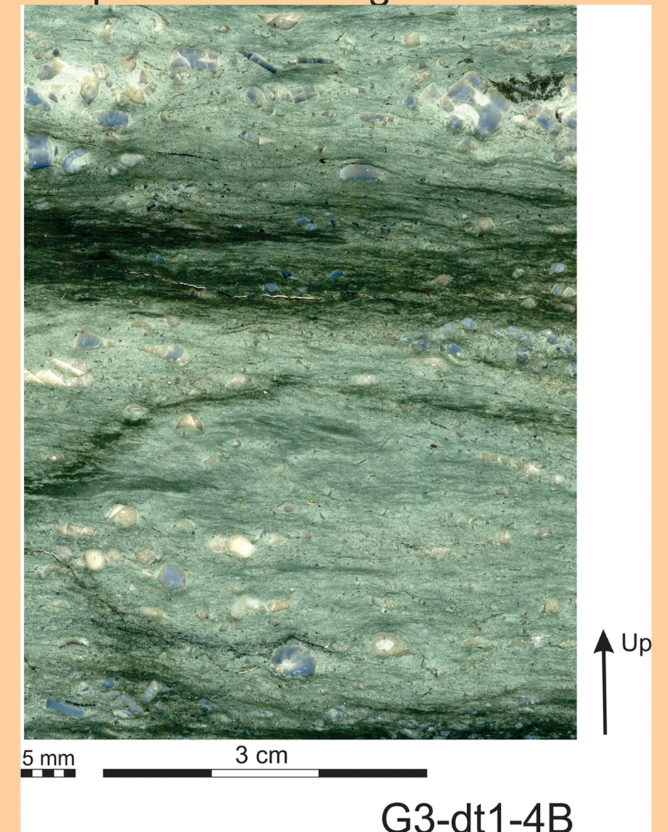
Siliciclastic Mudstone with dispersed crinoid grains Facies
