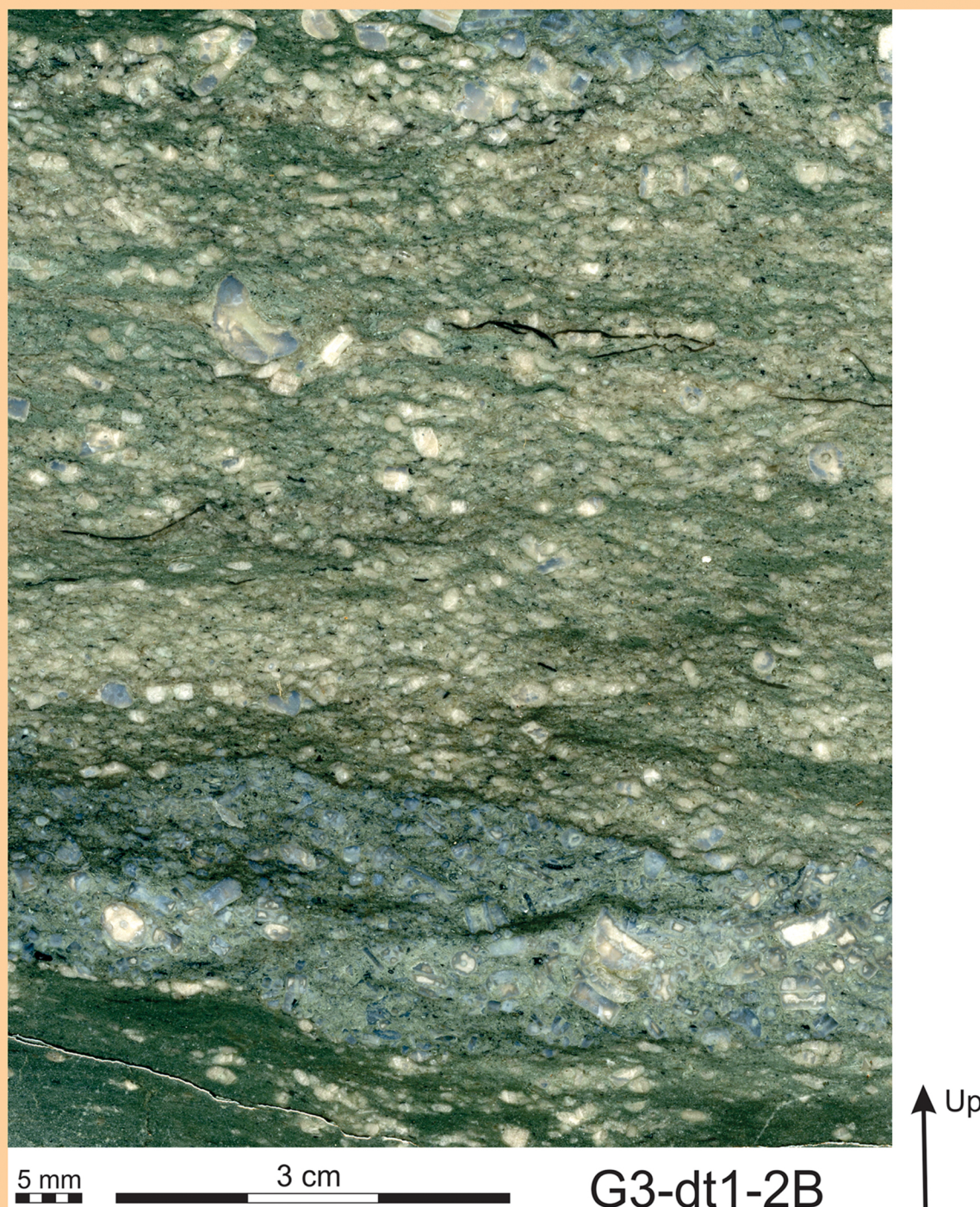
Grain-/packstone lens within the Siliciclastic Mudstone with dispersed crinoid grains Facies
