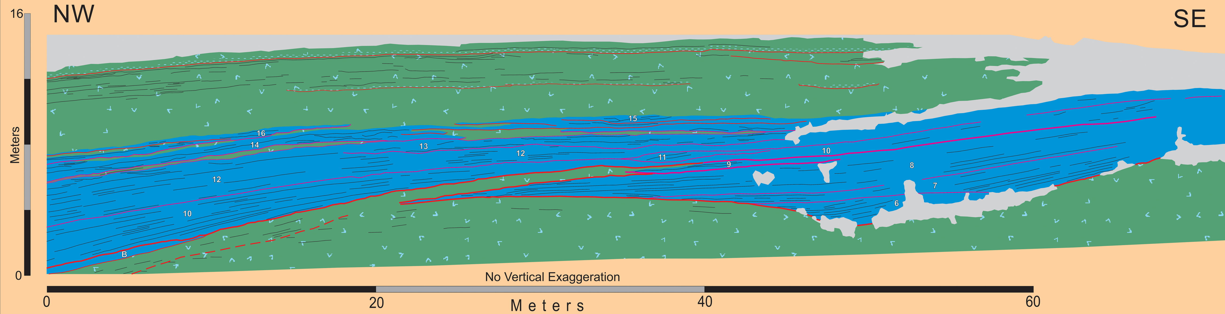
Section A1, Northwest Part Southwest-facing roadcut TN 52
