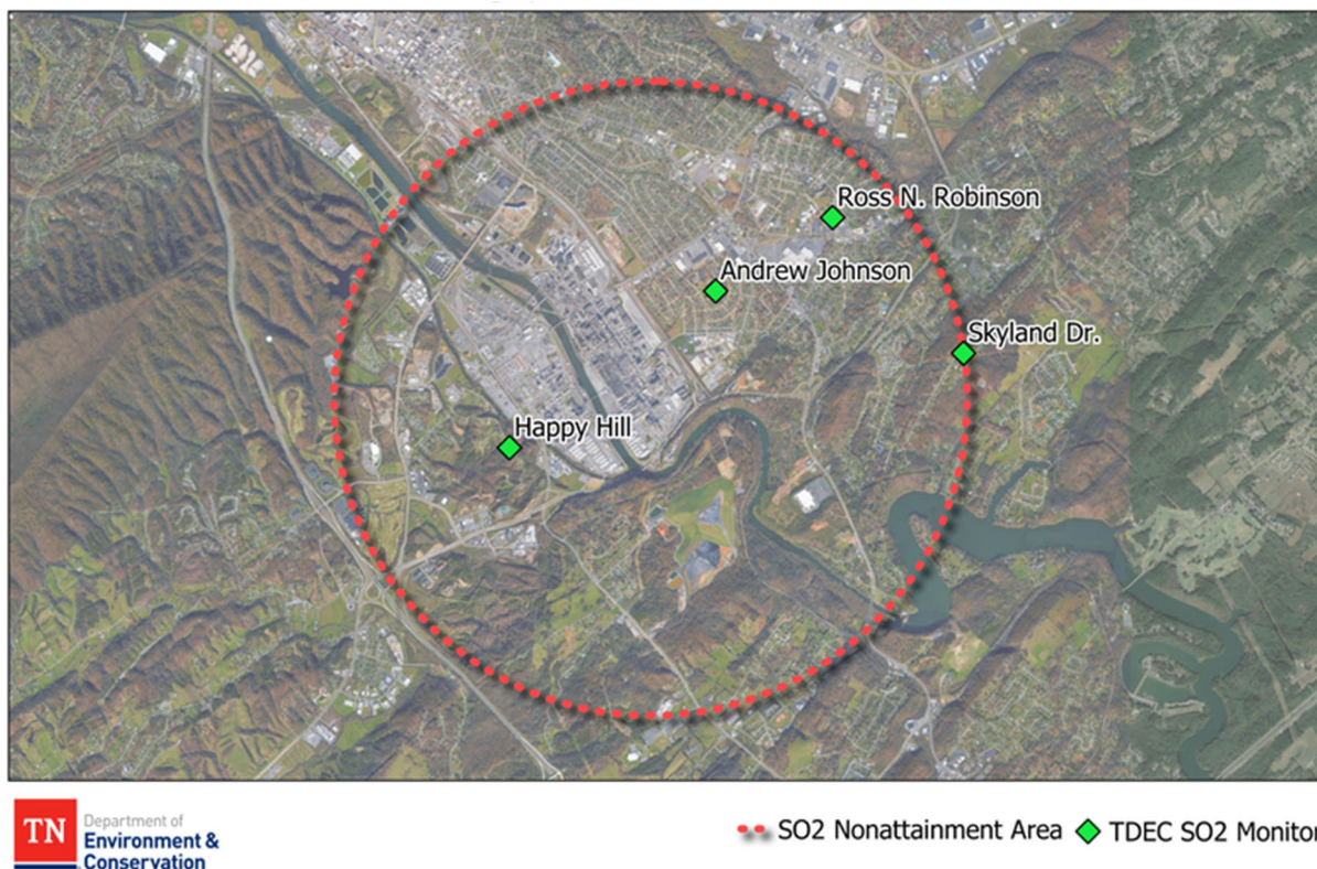
Figure 1-1: Kingsport SO 2 Nonattainment Area
