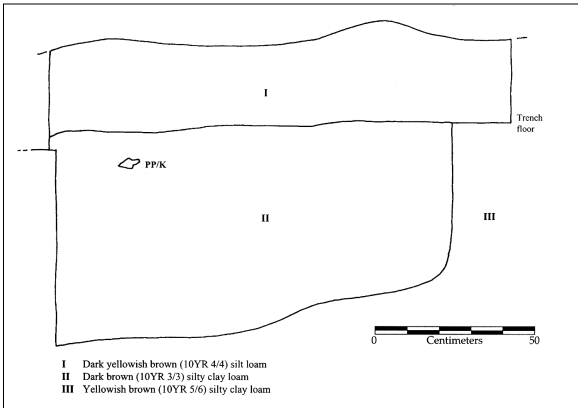
Figure 39. Drawing of Feature 1X profile in north wall of Block 1.
