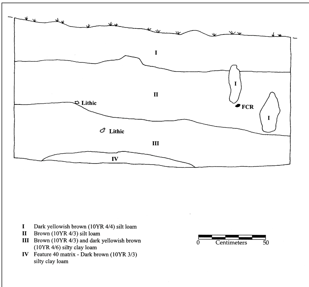
Figure 16. Profile of Feature 40 within the south wall of Trench 6.
