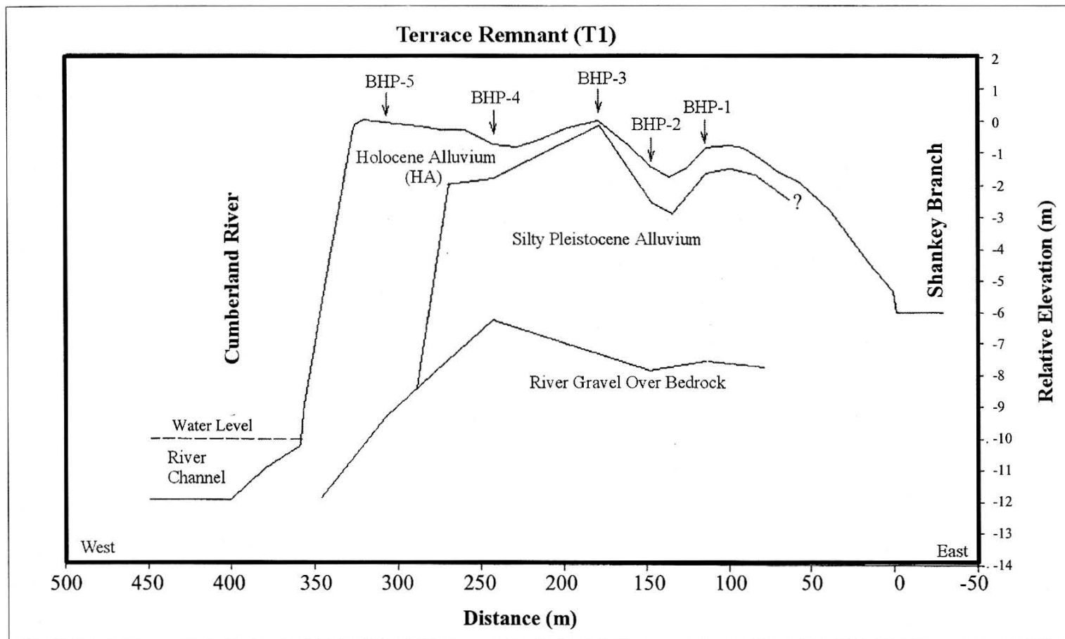
Figure 9: Stratigraphic cross-section through the line of section of backhoe pits 1-5.
