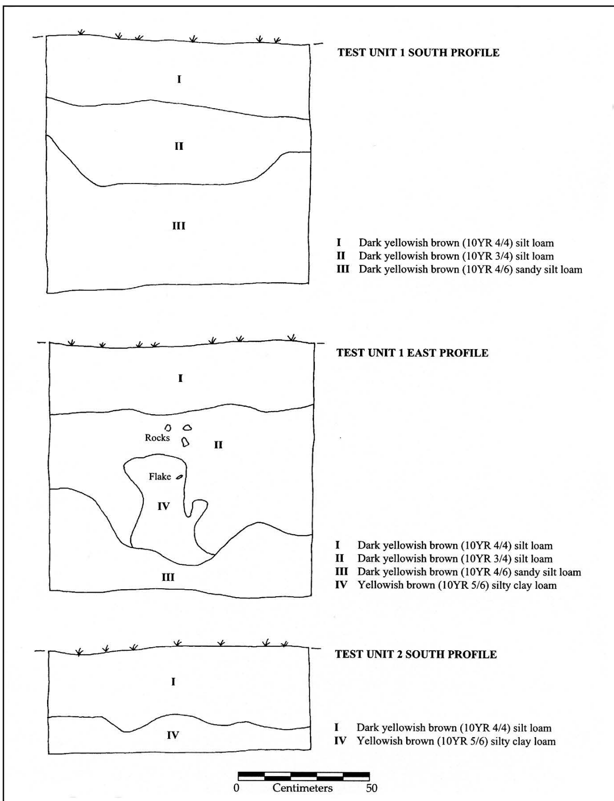
Figure 21. Test unit profiles from site 40CY64.
