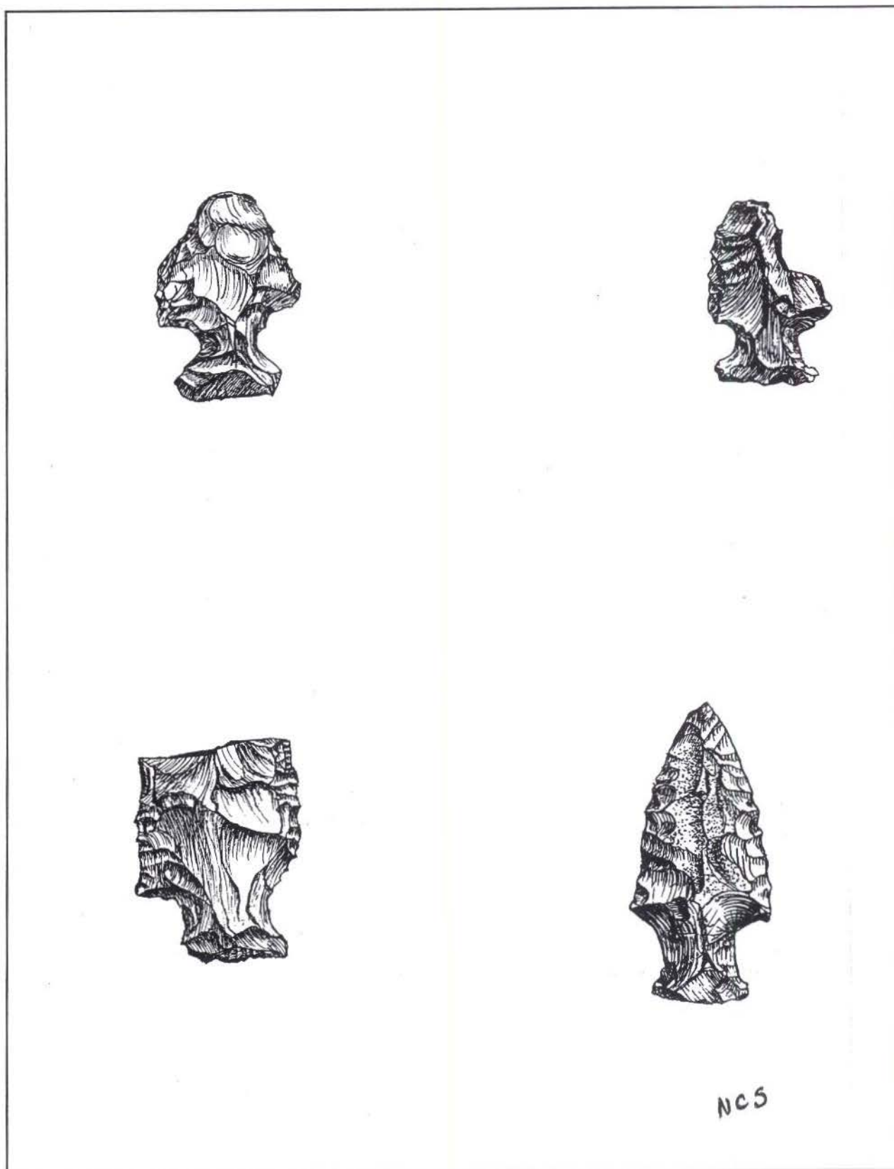
Figure 38. Motley Points.
