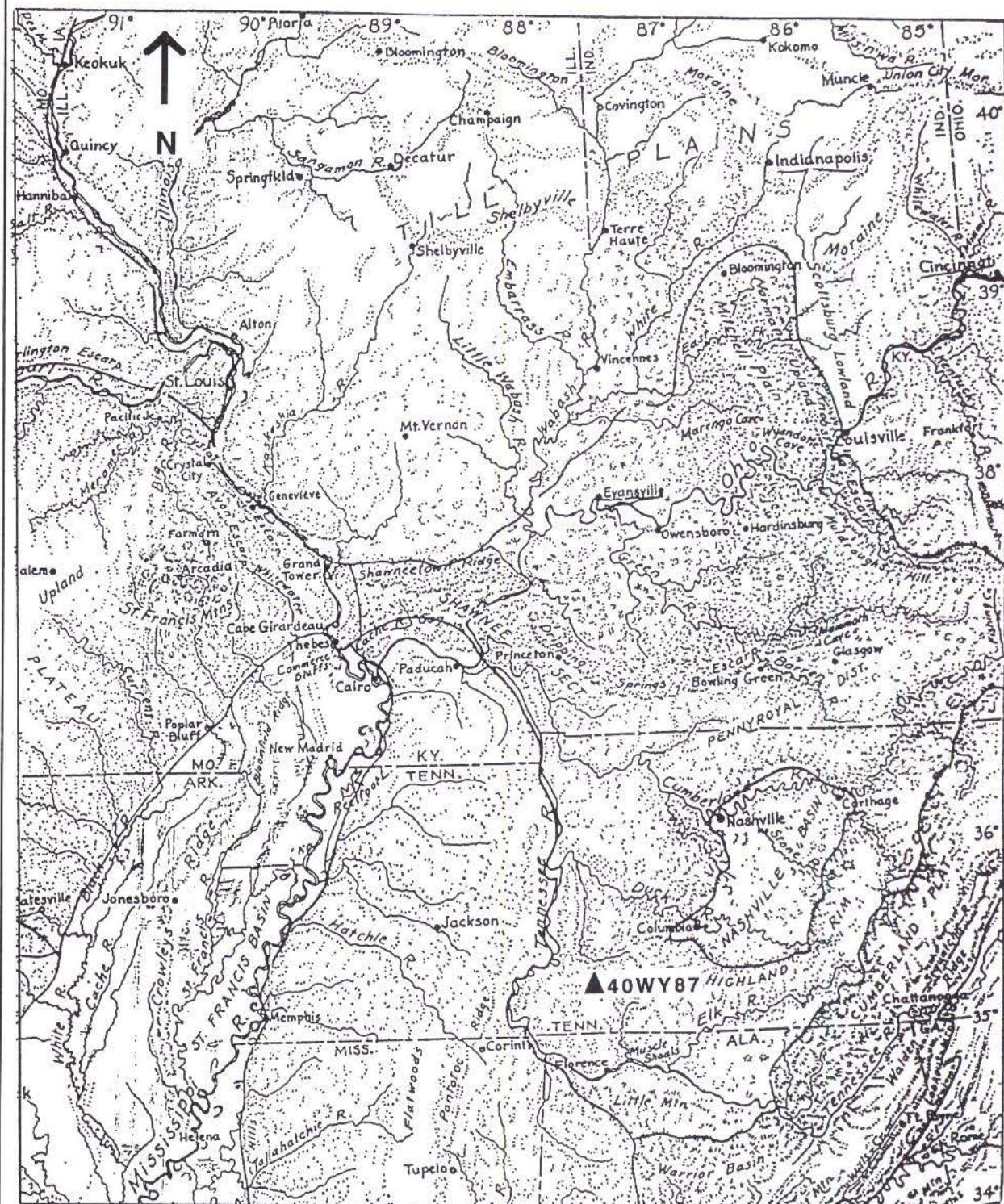
Figure 3. Regional Physiography.
