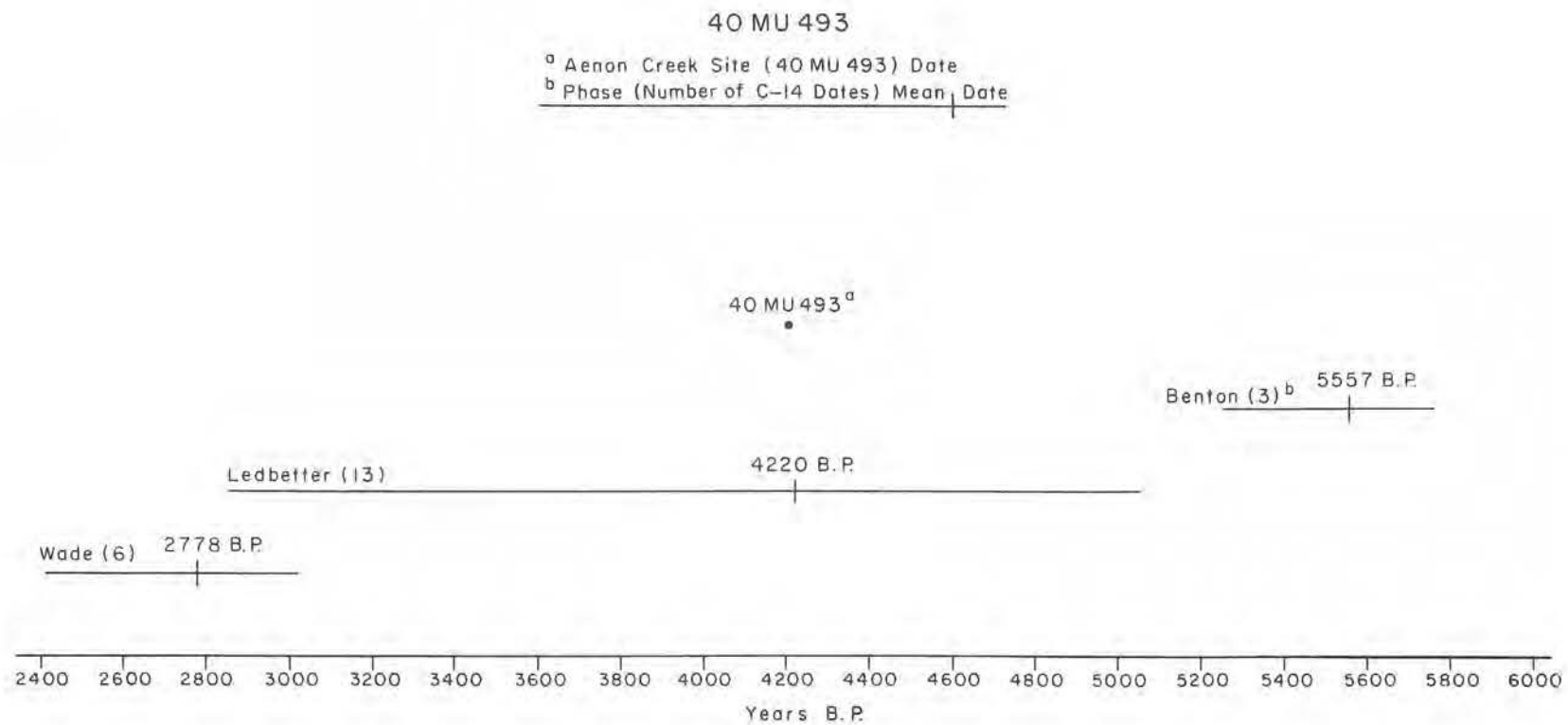
Figure 29. Chronological Distribution of Late Archaic Archaeological Phases.
