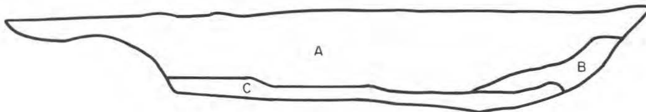
Feature 15
