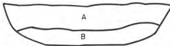
Feature 72
