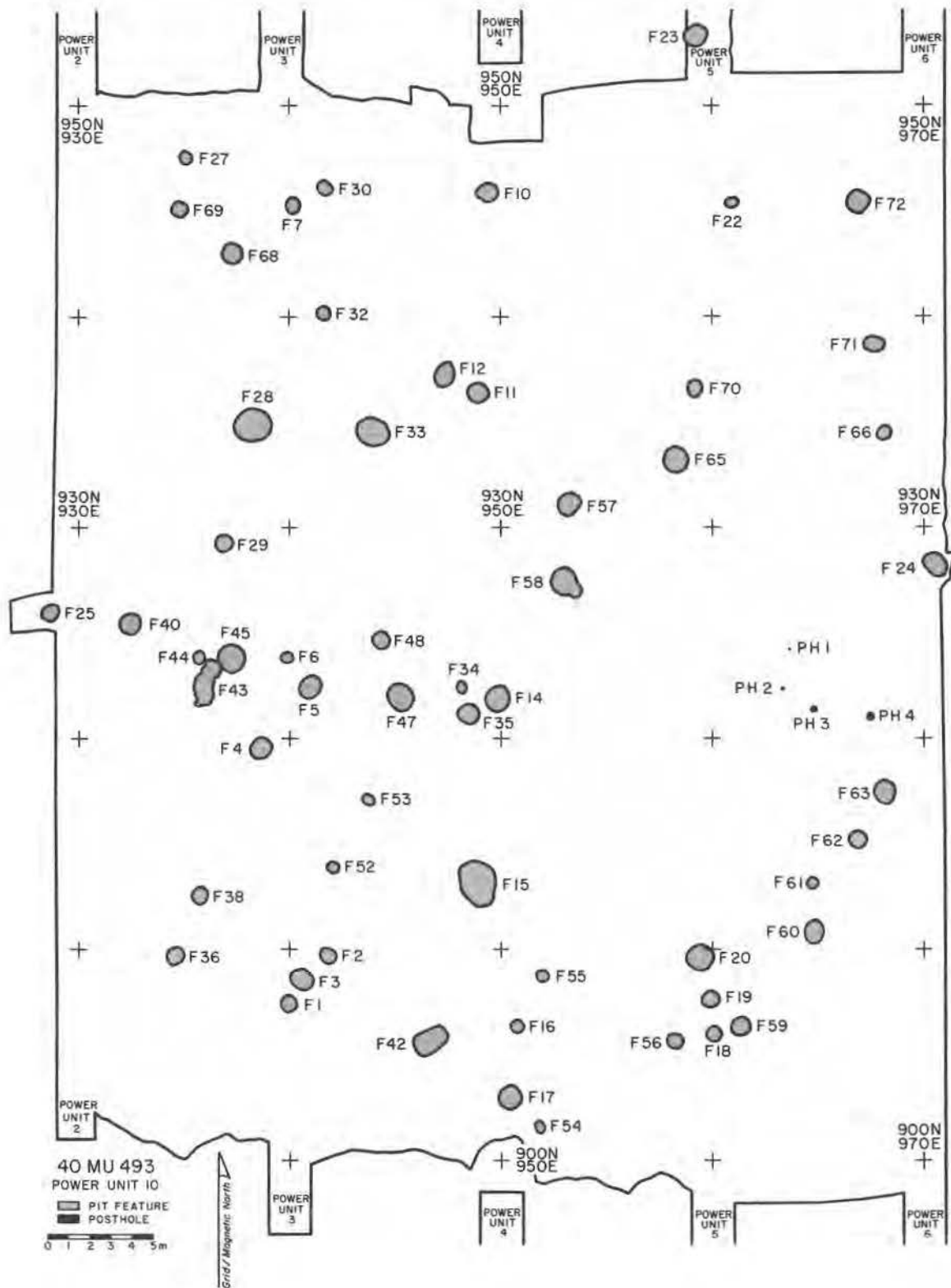
Figure 16. Feature Distribution.
