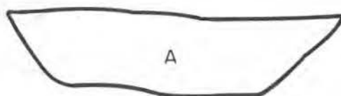
Feature 38
