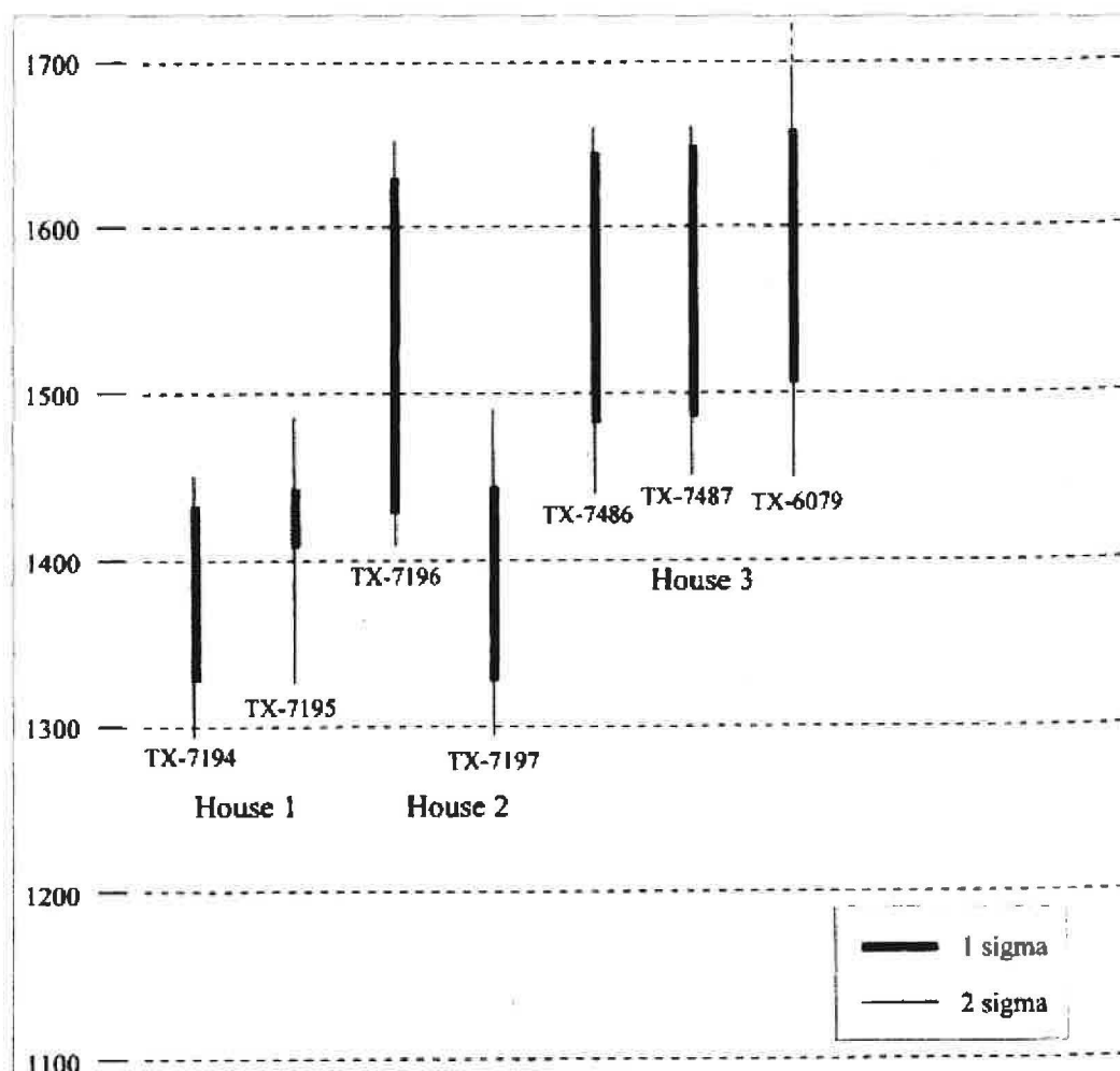
Figure 5-10. Radiocarbon determinations for Graves Lake (calibrated using CALIB 2.0 [Stuiver and Becker 1986]).
