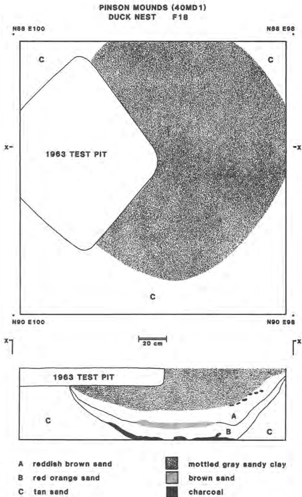
Fig. 23. Duck's Nest, Feature 18. Plan view: top; profile: bottom.
