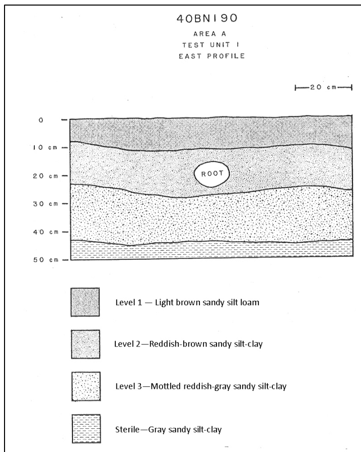
Figure 15. Test Unit 1, east profile.
