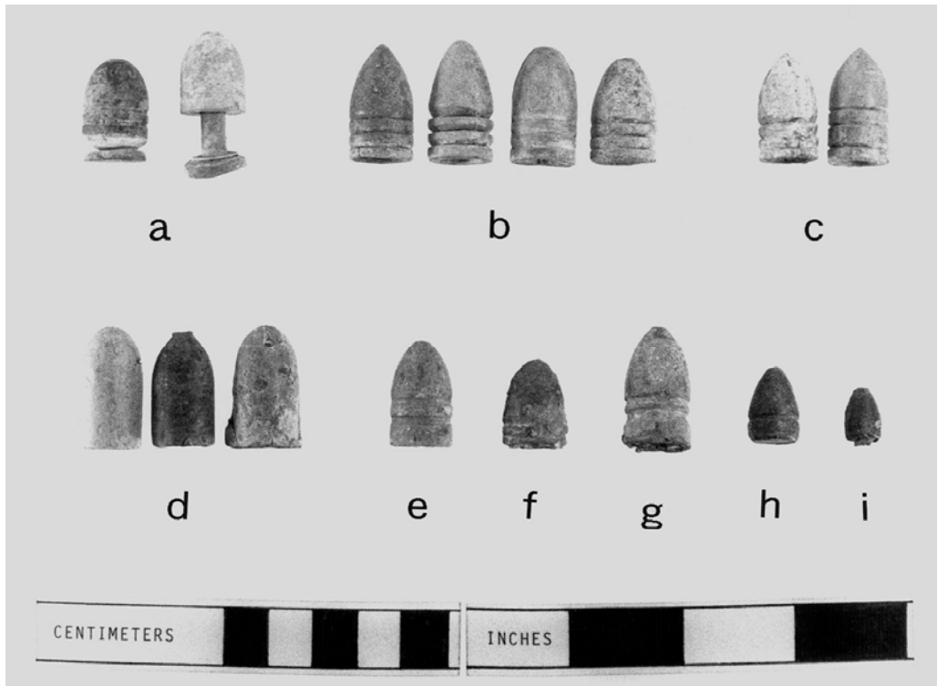
Figure 46. Conical bullet types: (a) Williams Cleaner (Type III), (b) 3-ring Minié (.58 cal.), (c) 3-ring Minié (.54 cal.), (d) Enfield-Pritchett, (e) Sharps, (f) Burnside, (g) Gardner, (h) .44 caliber, (i) .31 caliber.
