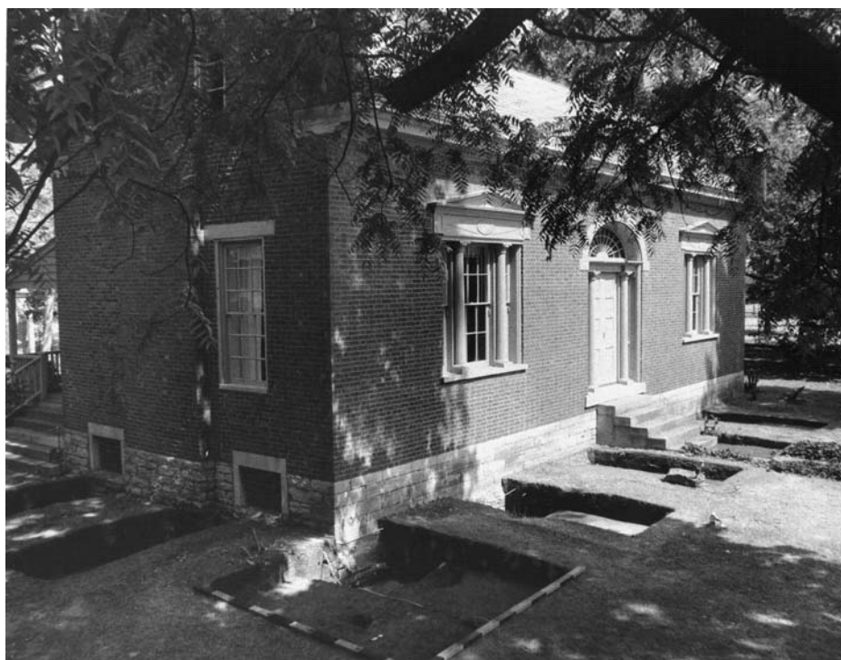
Figure 37. View of the Carter House (facing northwest) after completion of the first series of 1988 excavation units.
